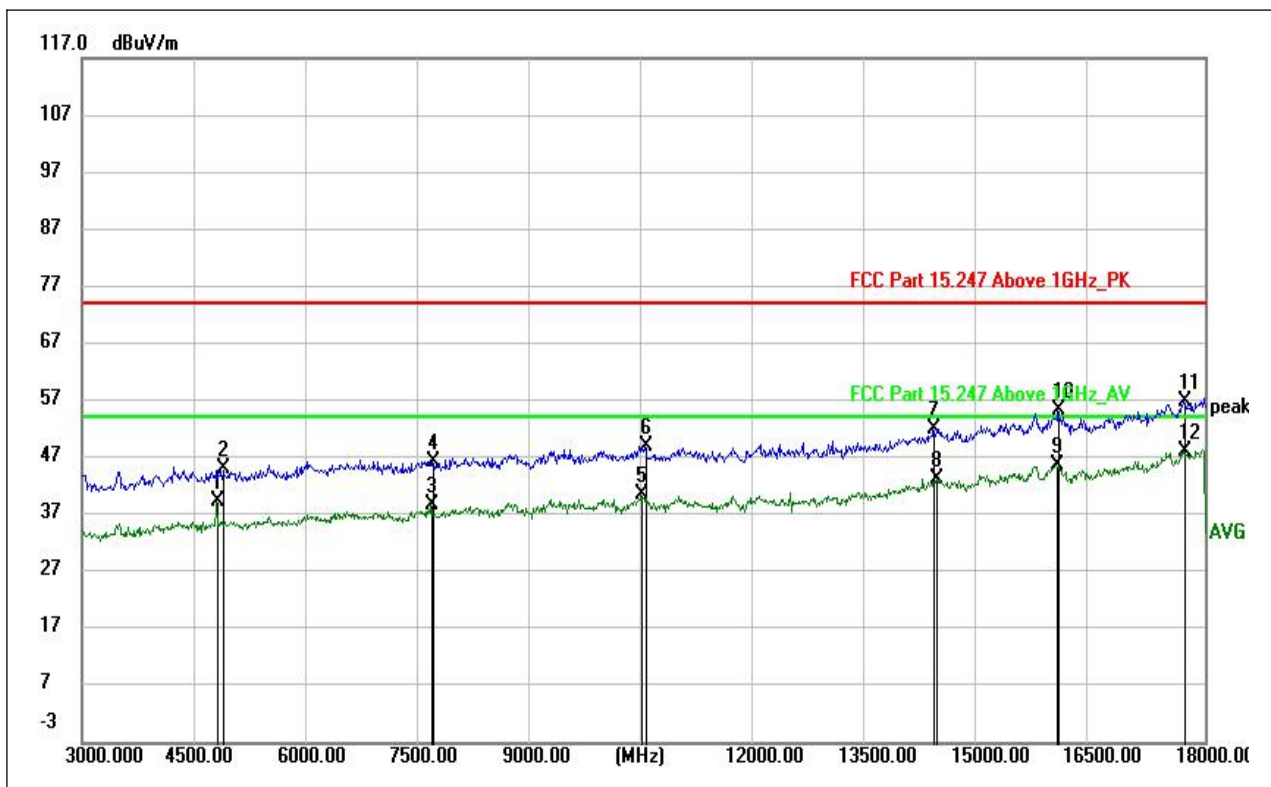
(LE 1M PHY _2405MHz, Antenna Horizontal, 3GHz to 18GHz)
