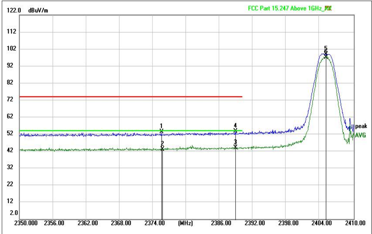
(BLE 1M PHY_2405MHz, Antenna Horizontal)
