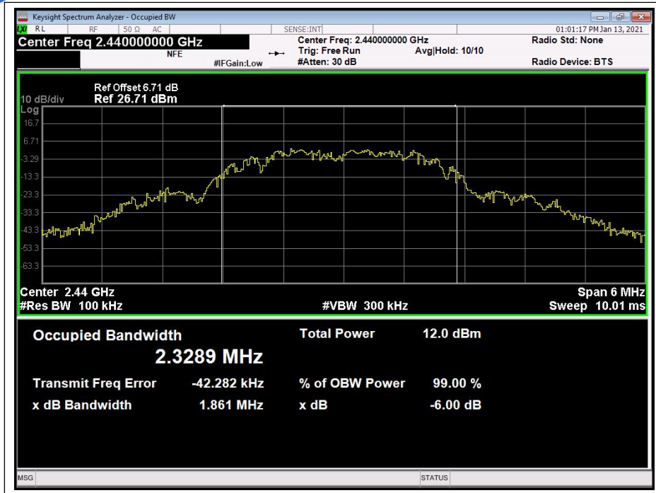
(Channel 18: 2440 MHz)
