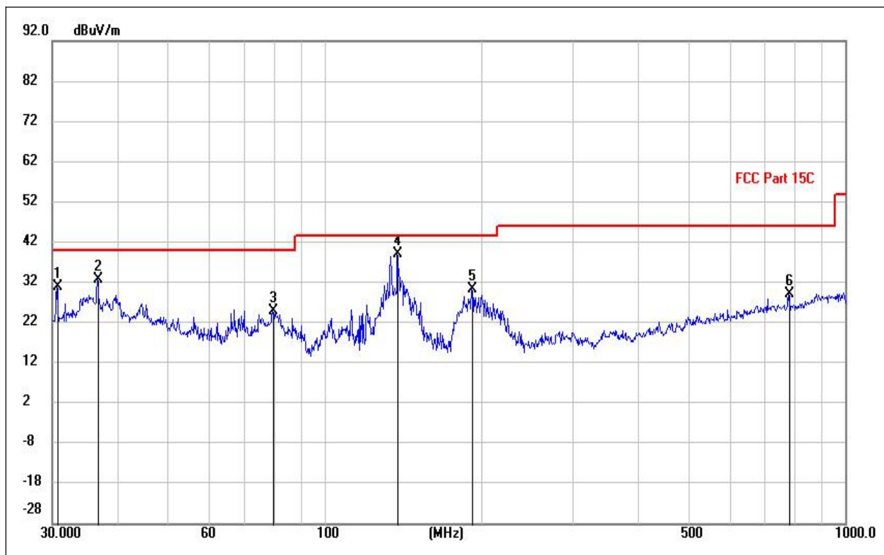
(LE 1M PHY _2405MHz, Antenna Vertical, 30MHz to 1GHz)
