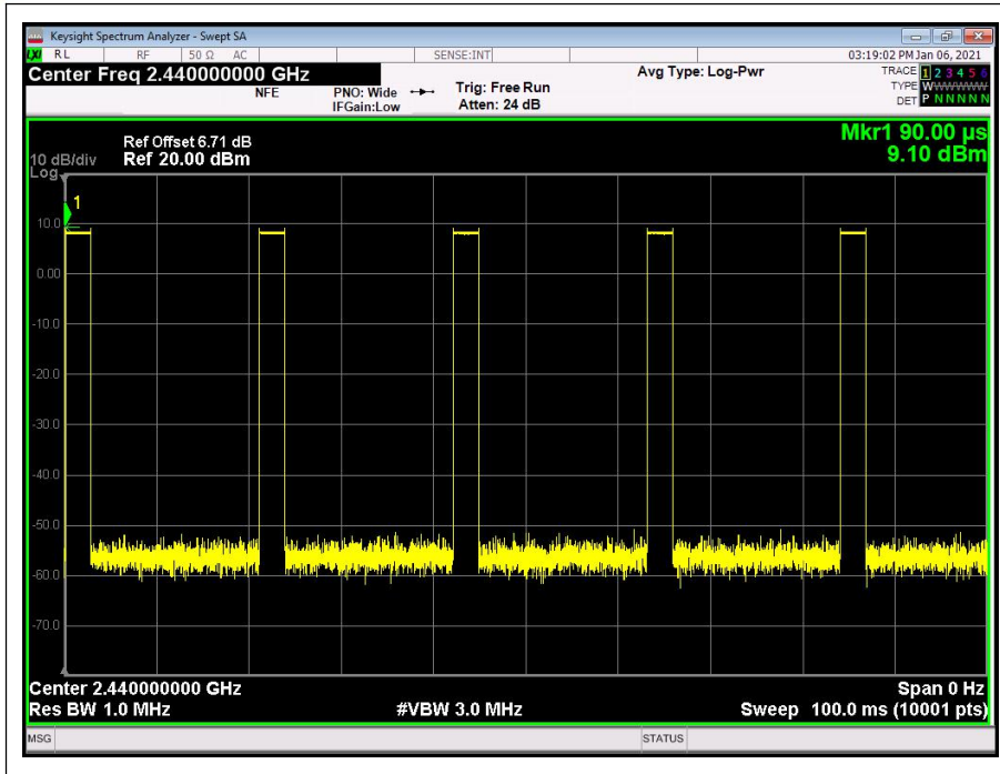
(Channel 18,2440MHz)
