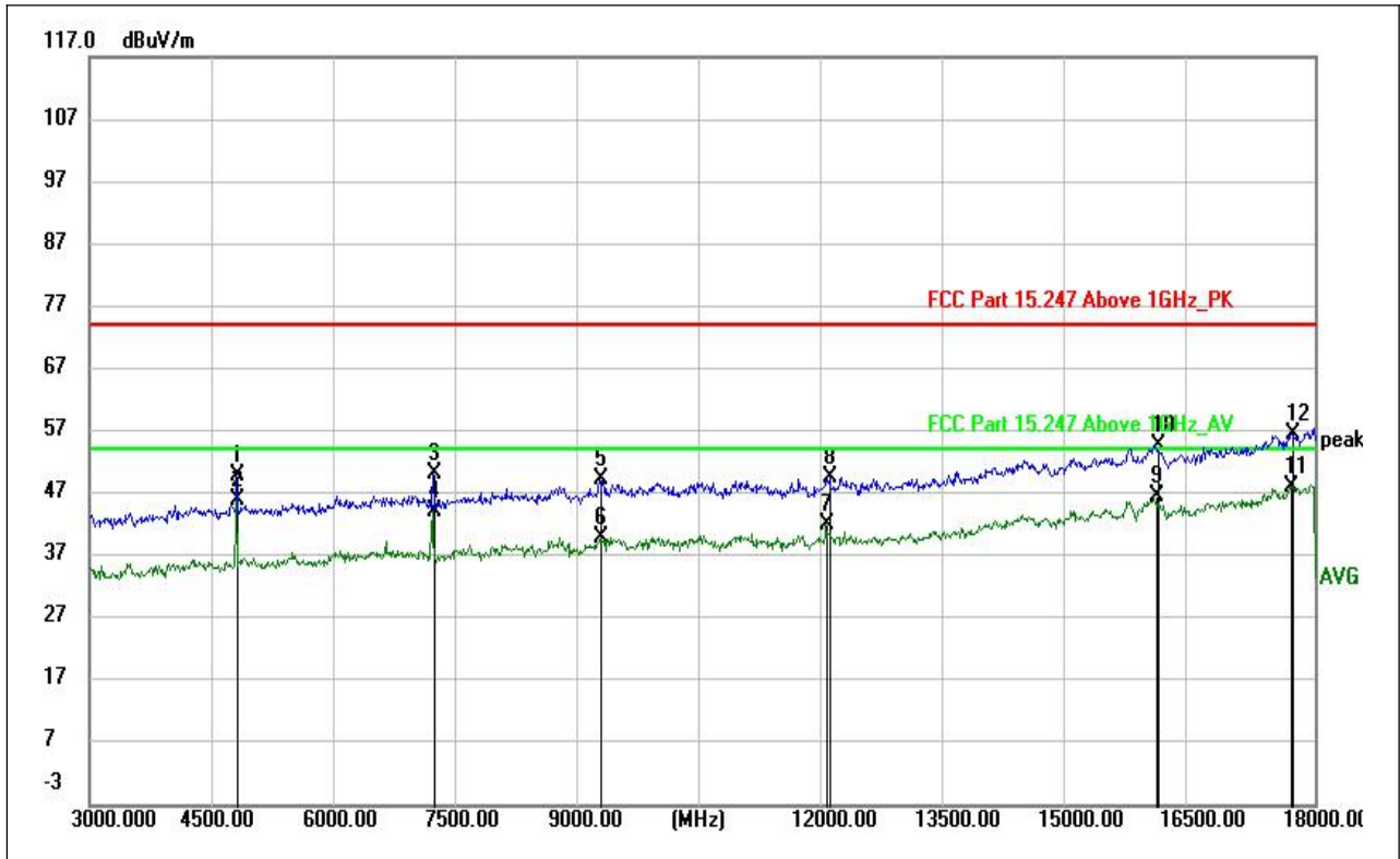
(LE 1M PHY _2405MHz, Antenna Vertical, 3GHz to 18GHz)
