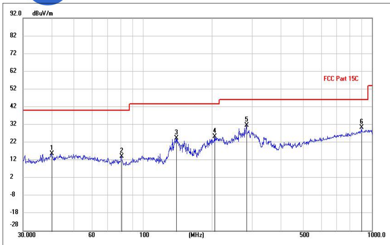
(LE 1M PHY_2440MHz, Antenna Horizontal, 30MHz to 1GHz)
