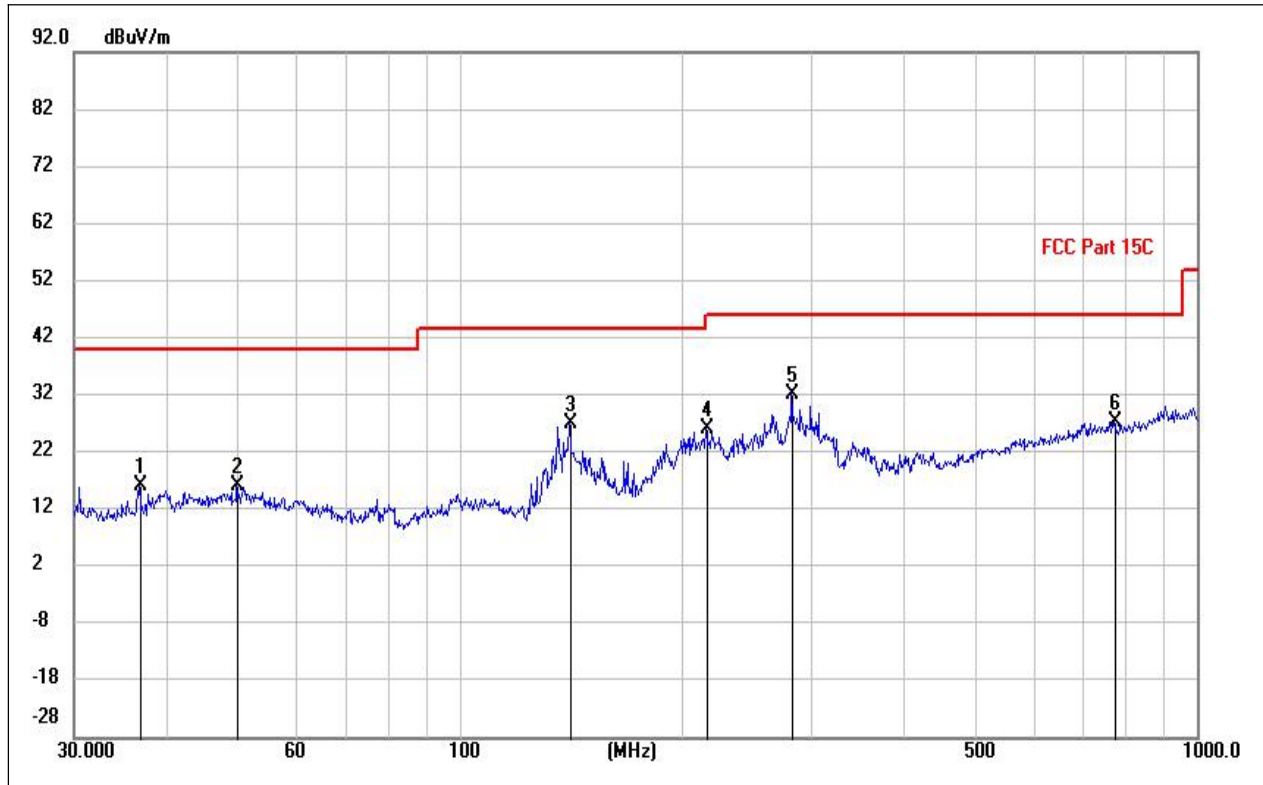
(LE 1M PHY _2480MHz, Antenna Horizontal, 30MHz to 1GHz)
