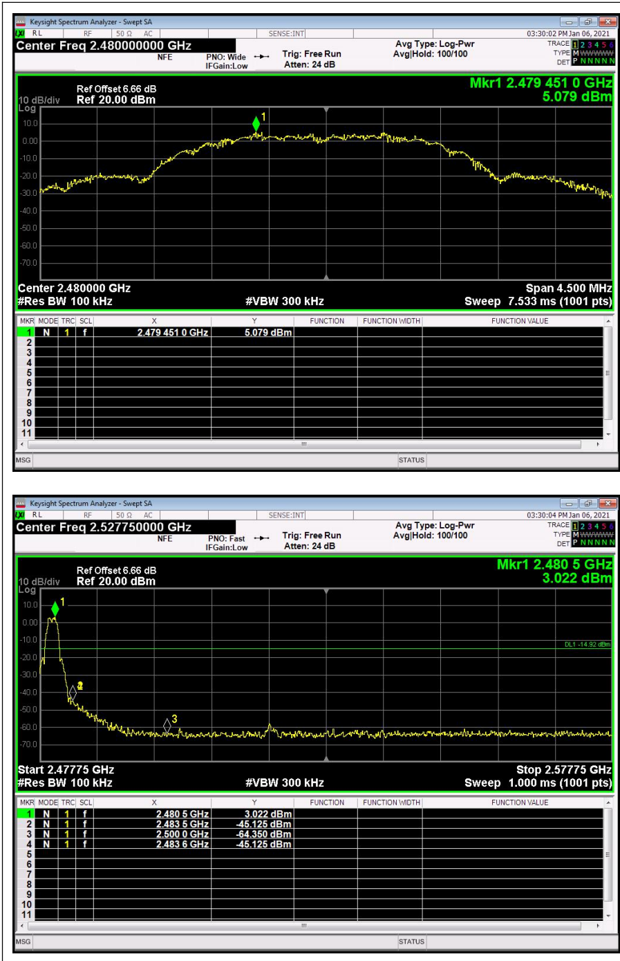
(Band Edge, Channel = 26)
