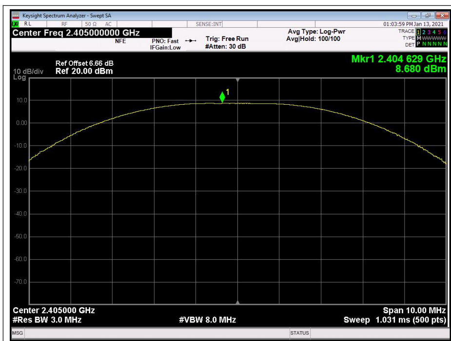
(Channel 11,2405MHz)
