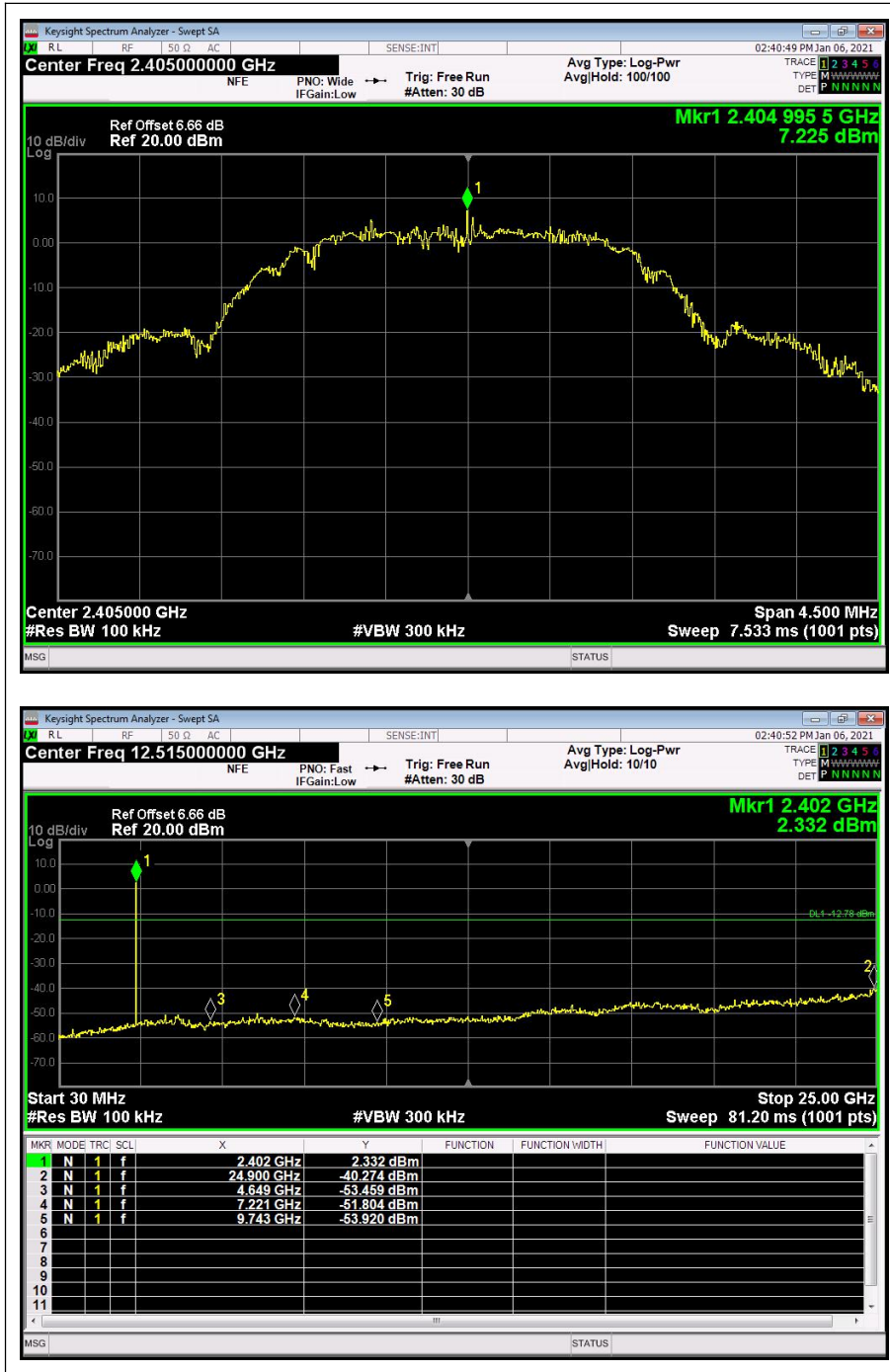
(Channel = 11, 30MHz to 25GHz)
