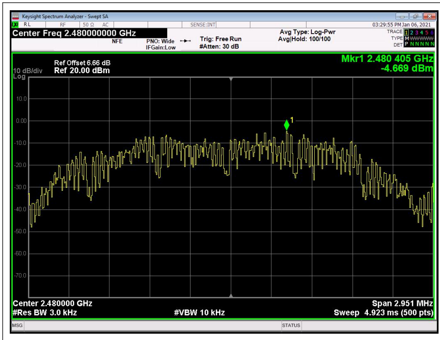
(Channel = 26, 2480MHz)
