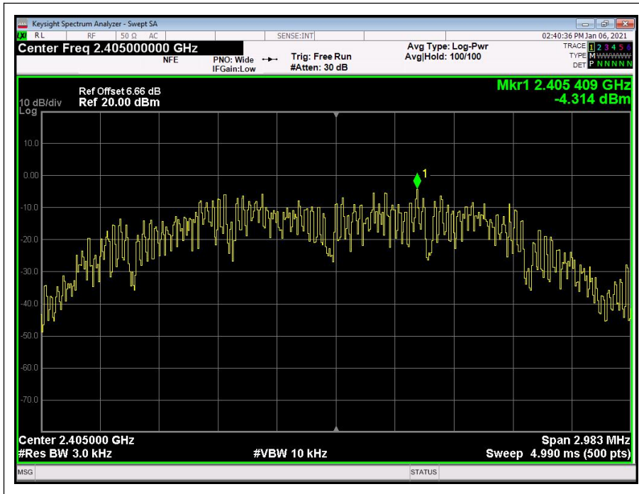
(Channel = 11, 2405MHz)
