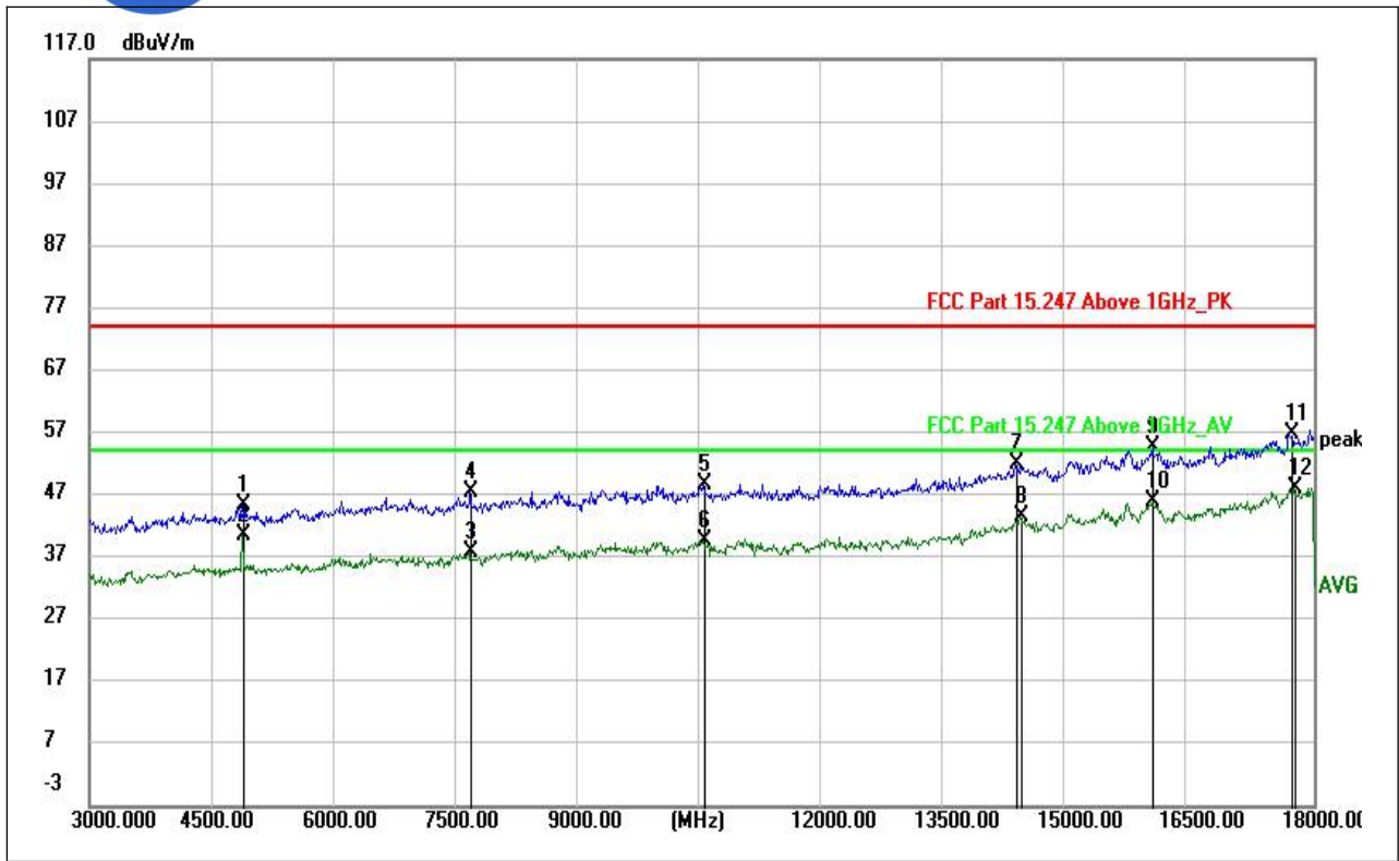
(LE 1M PHY_2440MHz, Antenna Horizontal, 3GHz to 18GHz)
