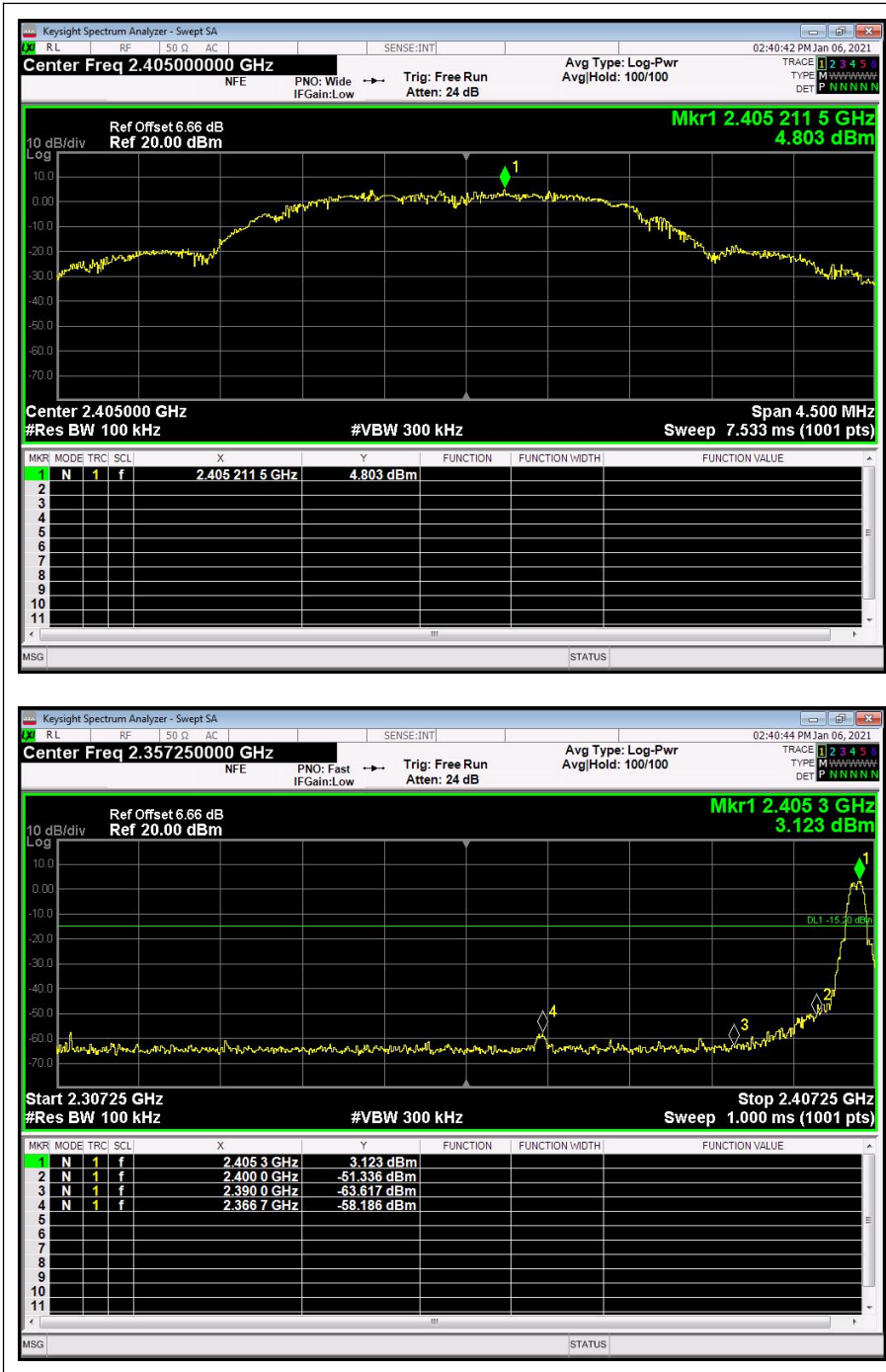
(Band Edge, Channel = 11)
