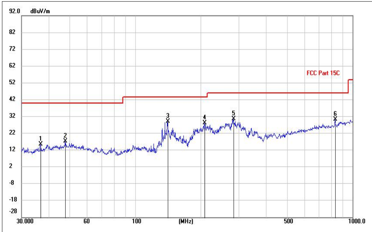
(LE 1M PHY_2405MHz, Antenna Horizontal, 30MHz to 1GHz)
