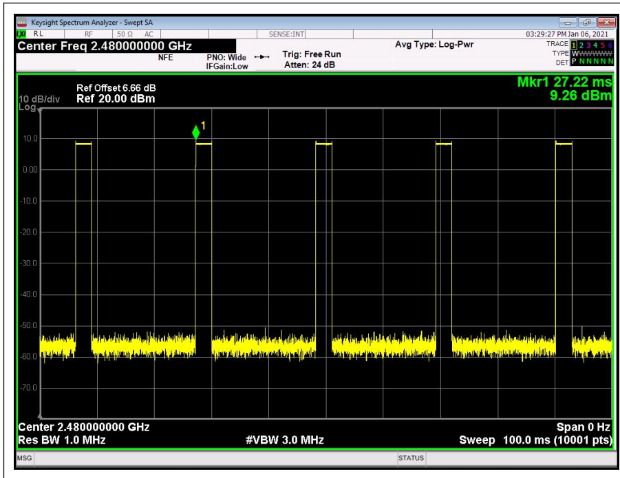
(Channel 39,2480MHz)
