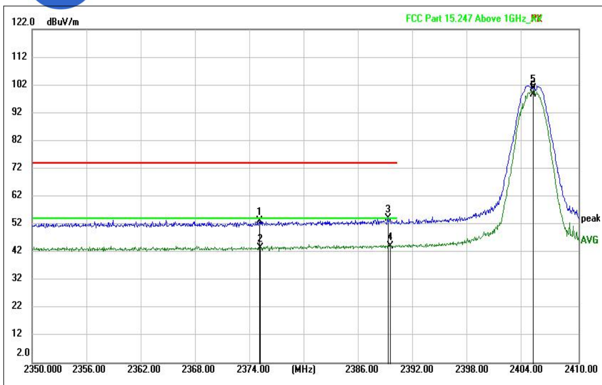
(LE 1M PHY_2405MHz, Antenna Vertical)
