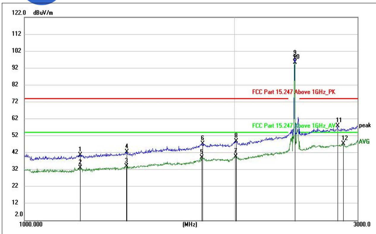
(LE 1M PHY _2440MHz, Antenna Horizontal, 1GHz to 3GHz)
