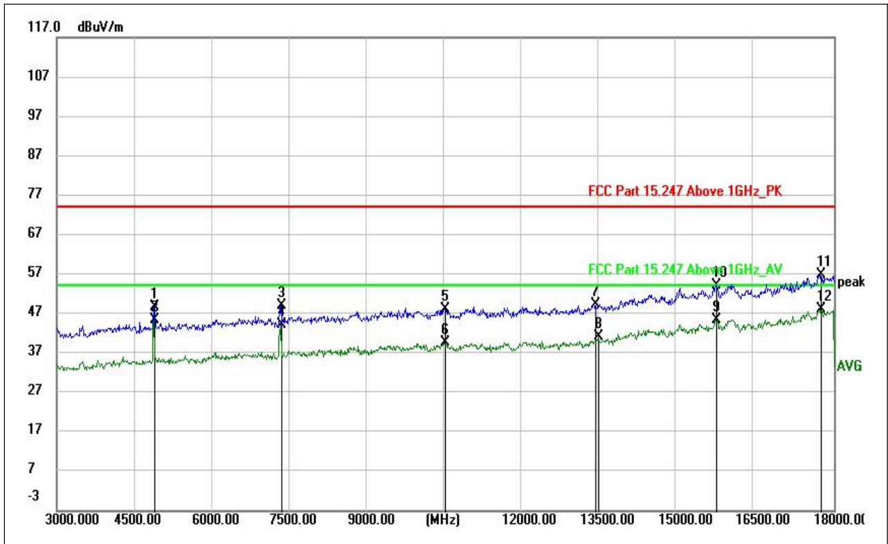
(LE 1M PHY _2440MHz, Antenna Vertical, 3GHz to 18GHz)
