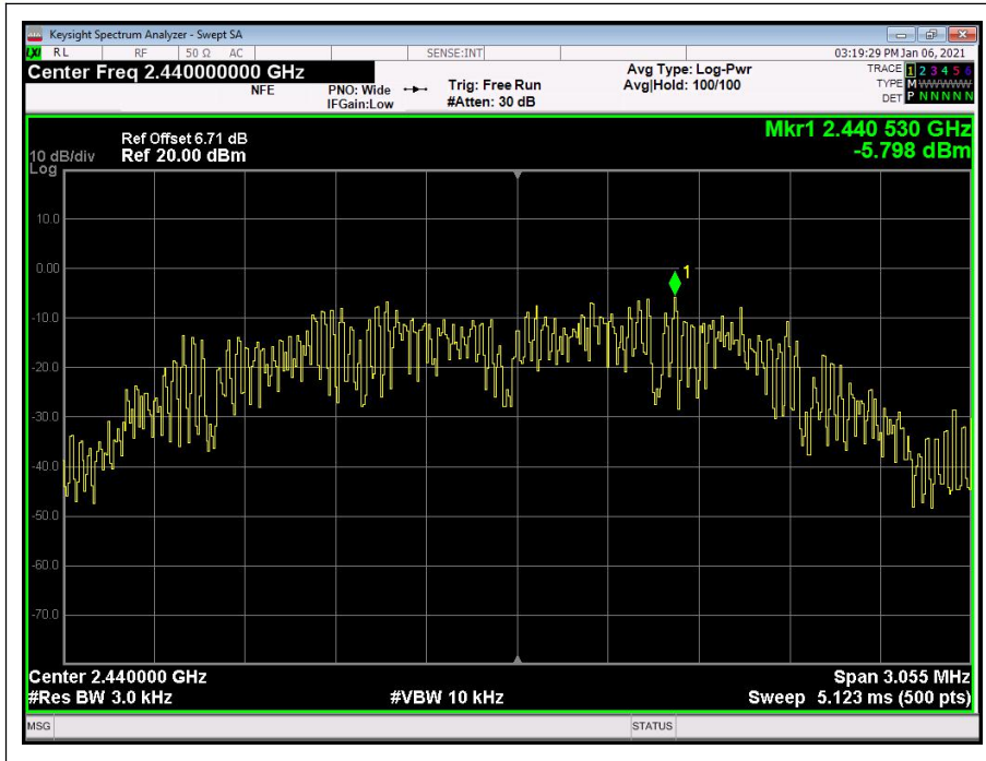
(Channel = 18, 2440MHz)
