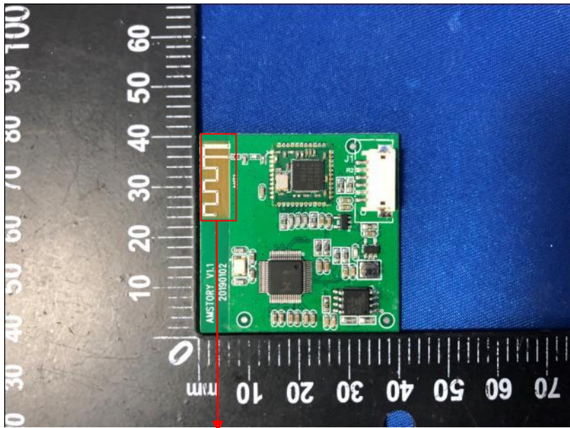
RF Antenna
