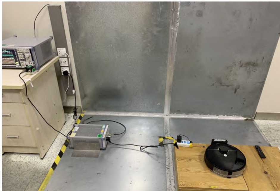
Radiated Spurious Emissions From 30MHz-1000MHz
