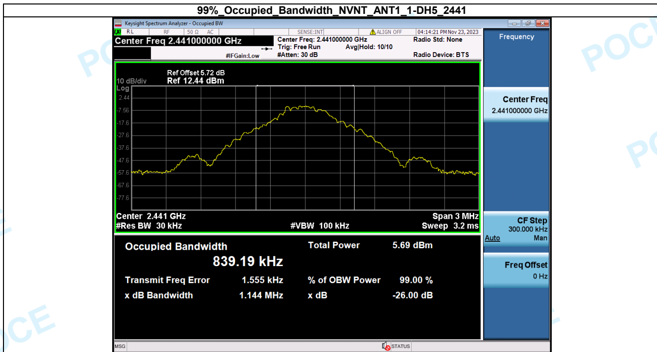
99%_Occupied_Bandwidth_NVNT_ANT1_1-DH5_2441
