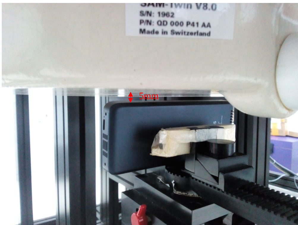
Body Left Setup Photo (5mm)
