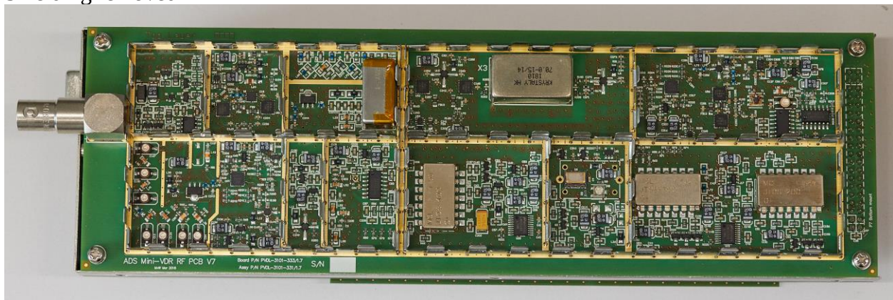
Shielding removed
