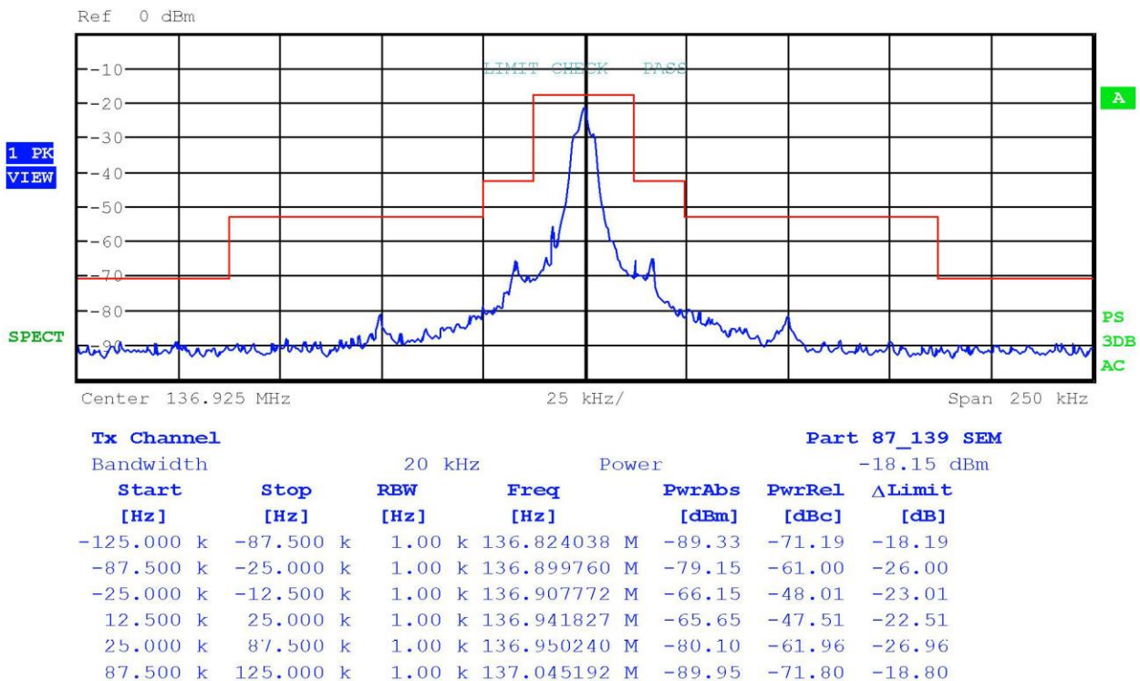
Figure 7 Spectral Emission Mask at Antenna Terminal ACARS
