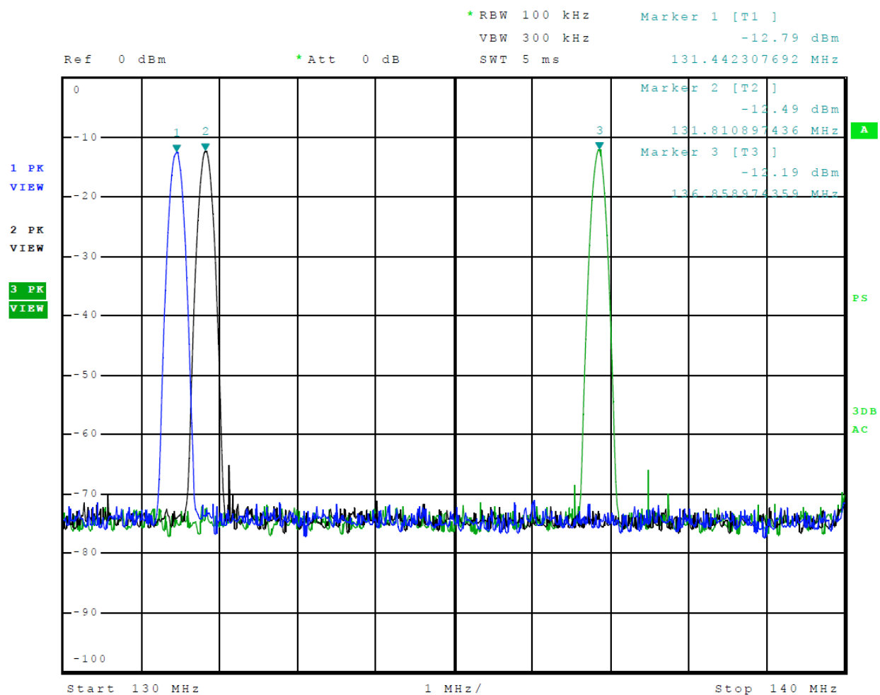
Figure 1 Power Output Across Frequency Band 131 and 136.850 MHz (VDL)
