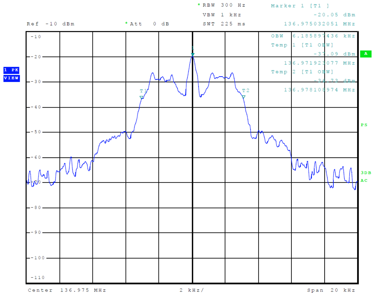
Figure 4 Occupied Band Width ACARS
