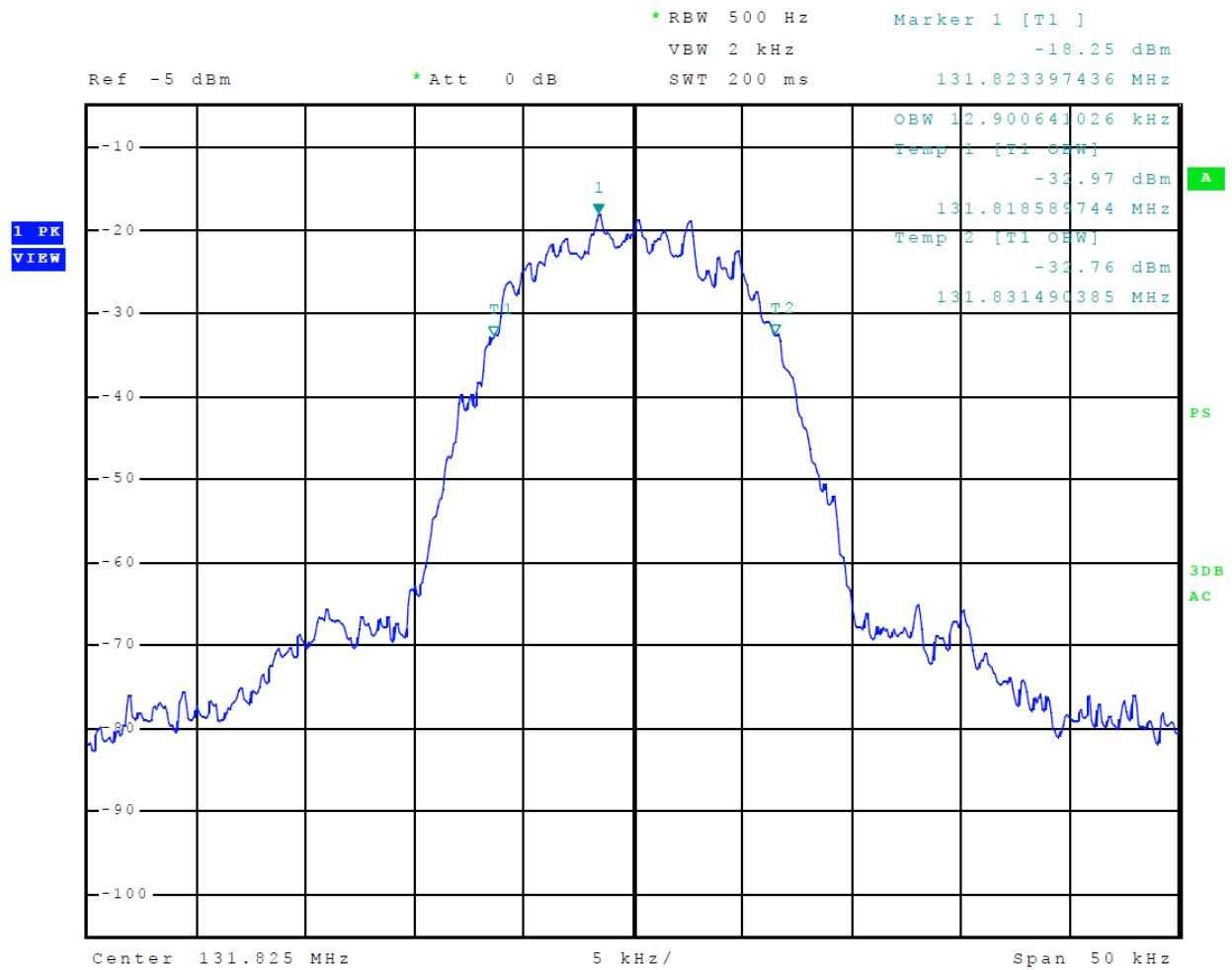
Figure 3 Occupied Band Width VDL
