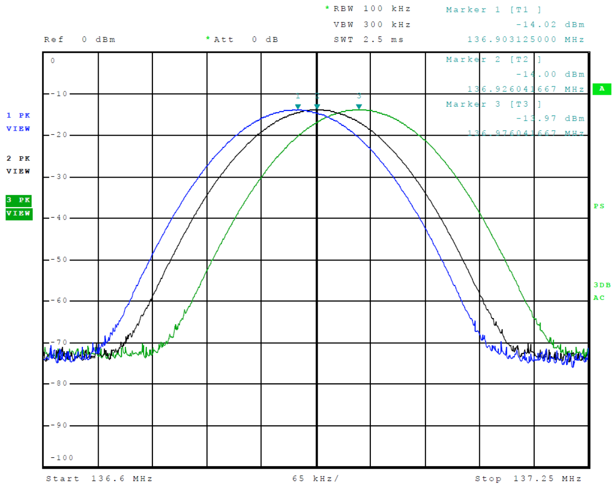
Figure 2 Power Output Across Frequency Band 136. MHz (ACARS)
