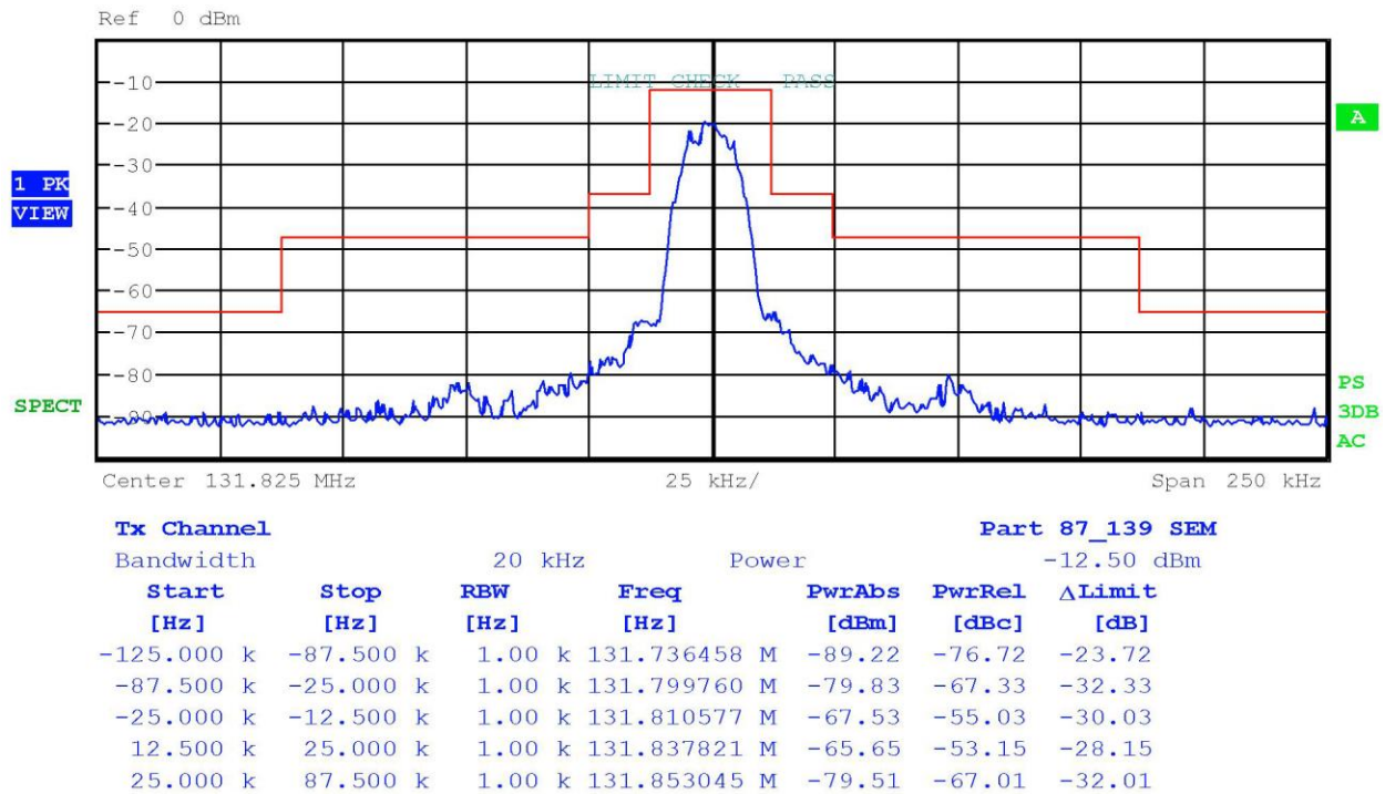
Figure 6 Spectral Emission Mask at Antenna Terminal VDL
