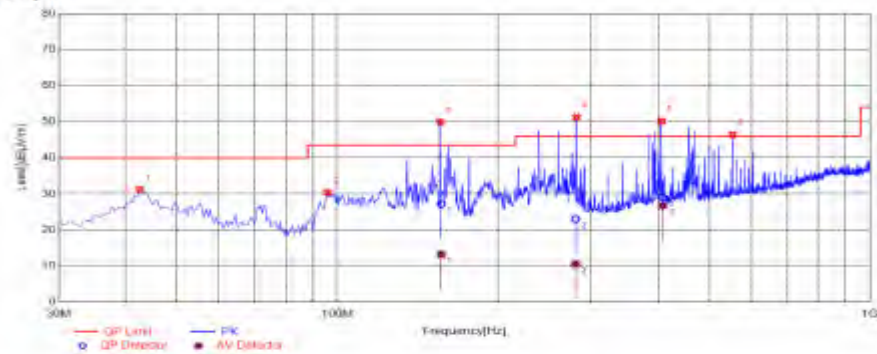
Test Graph
