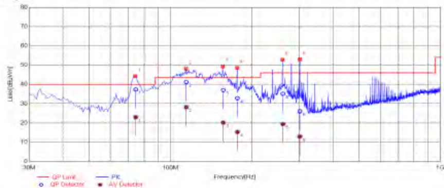
Test Graph
