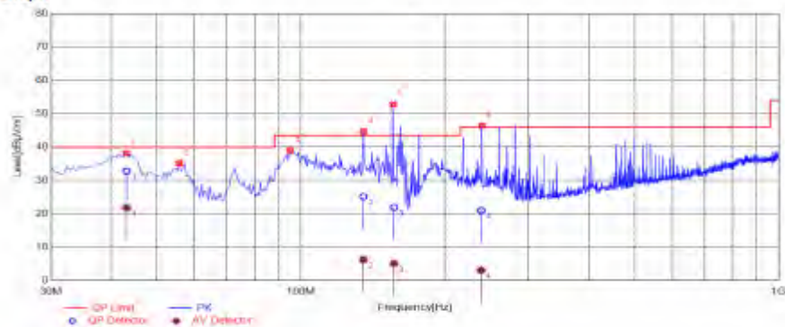
Test Graph
