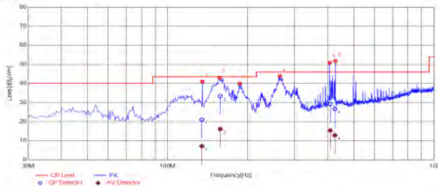
Test Graph
