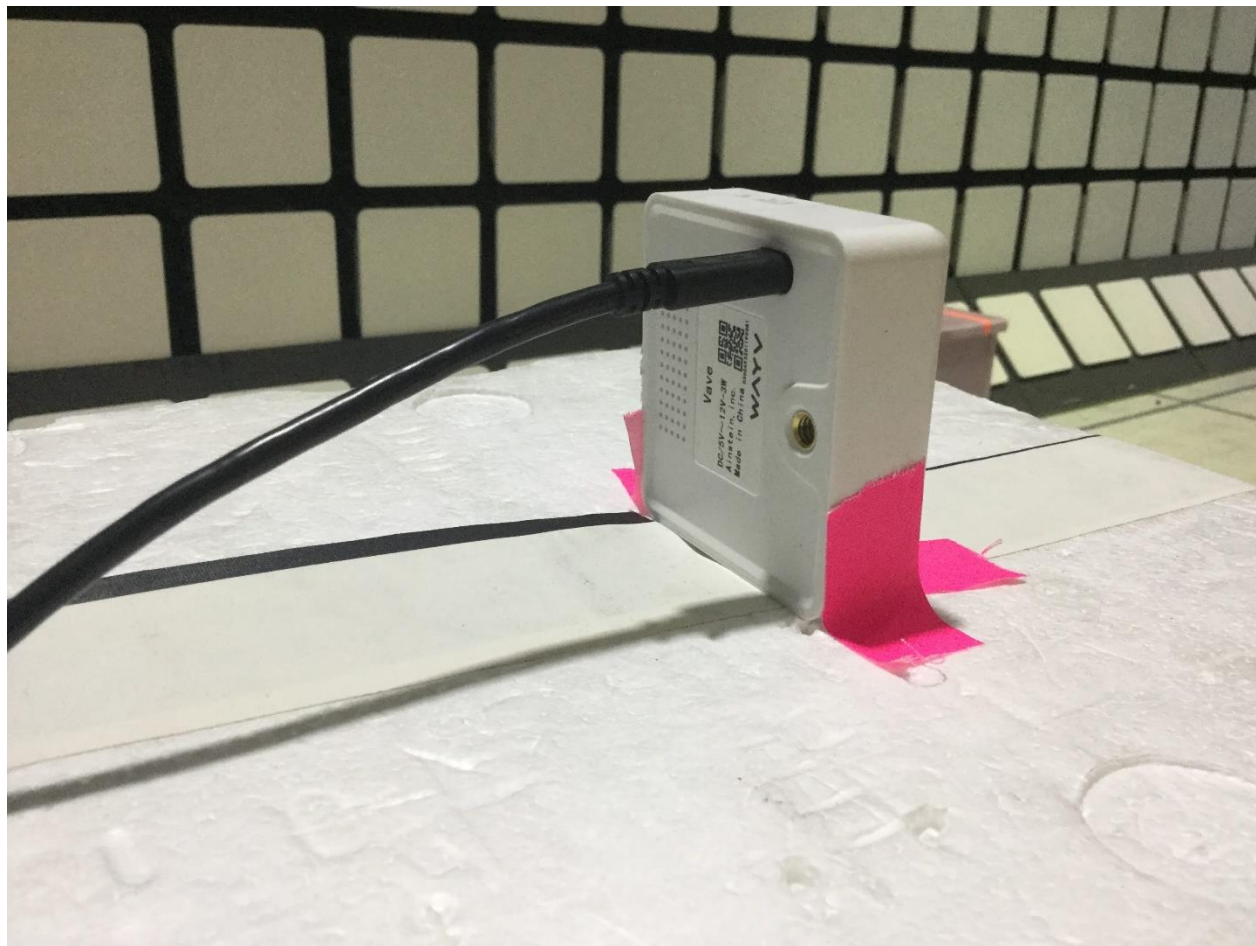
Radiated Emissions, 1 – 18 GHz, 3m
