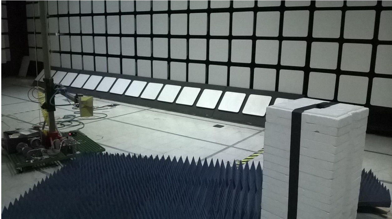
Radiated Emissions, 1 – 18 GHz, 3m, Setup only, EUT not shown
