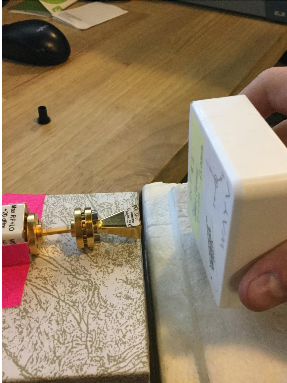
Radiated emissions, 140 - 220 GHz, 3 cm
