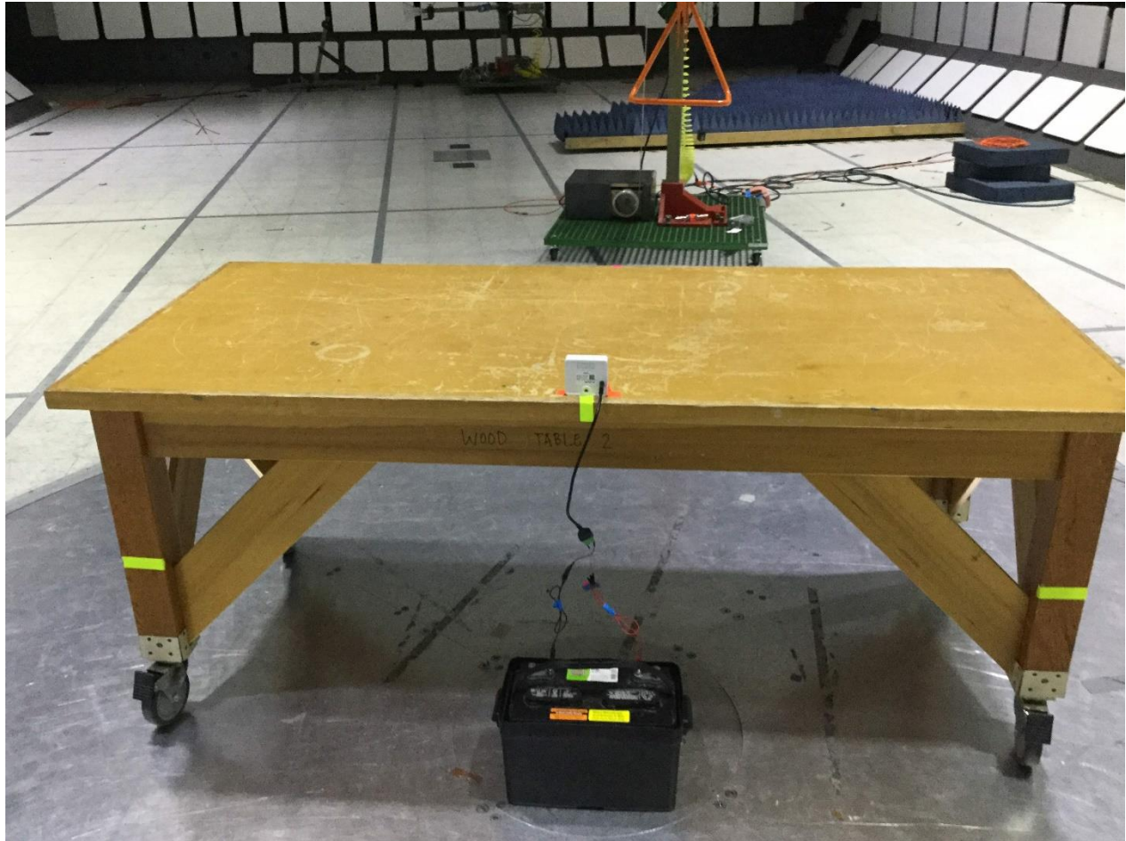
Radiated emissions, 30 MHz – 1 GHz, 3m
