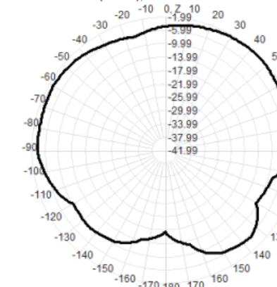
900.0MHz Total(E2-YZ), Max=-2.23dBi
