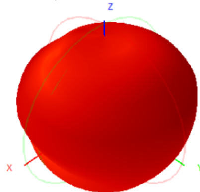
980.0MHz H+V, Eff: 35.5%
