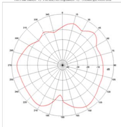
Far-field Power Distribution(H+V) on X-Z Plane Plot Peak Gain(H+V)= 1.68 dBi; Plot AvgGain(H+V)= -3.80dBi @2.44000 GHz
