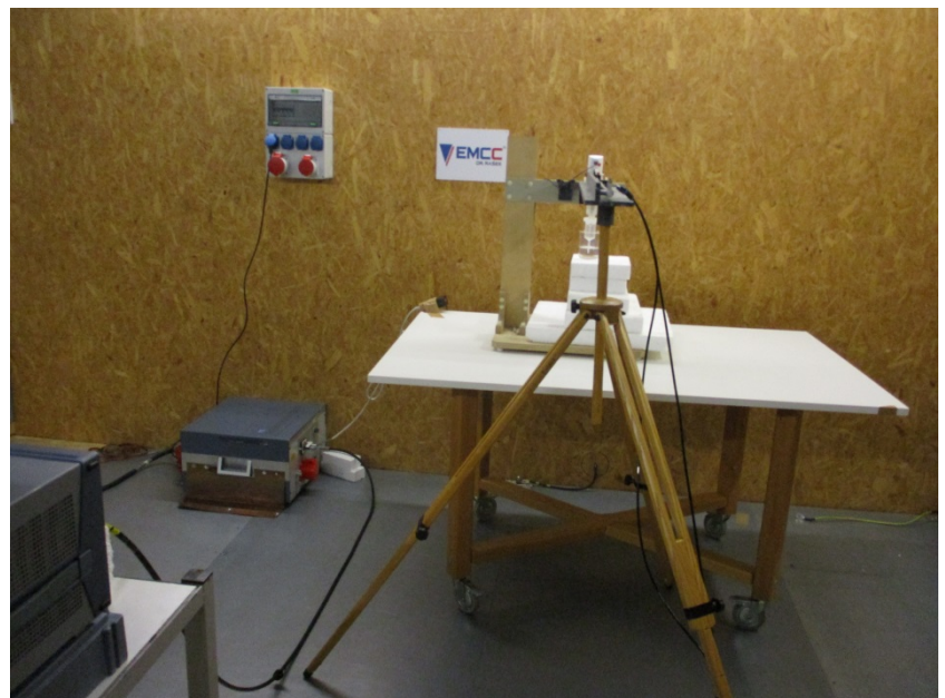
Photo of setup, Mode 2
