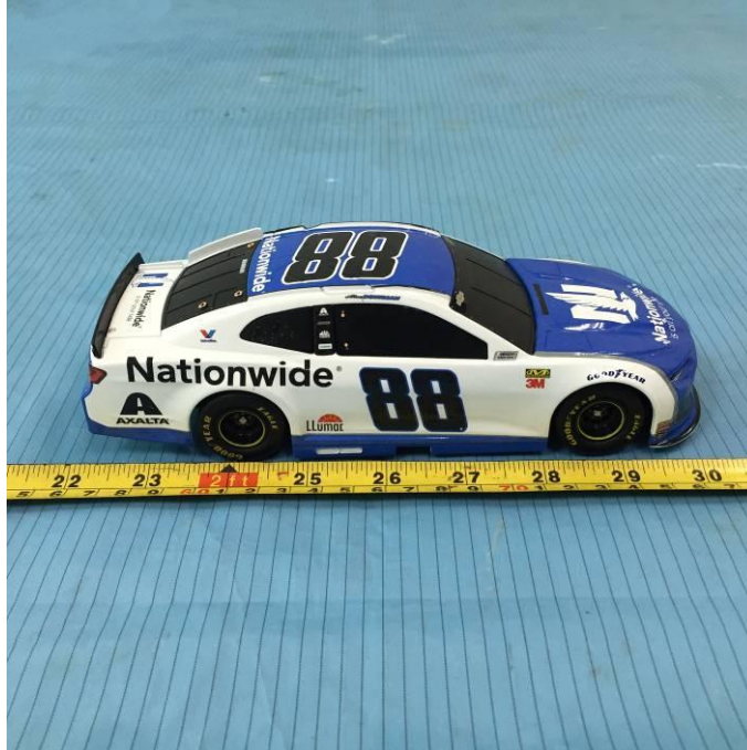
EUT-Left View
