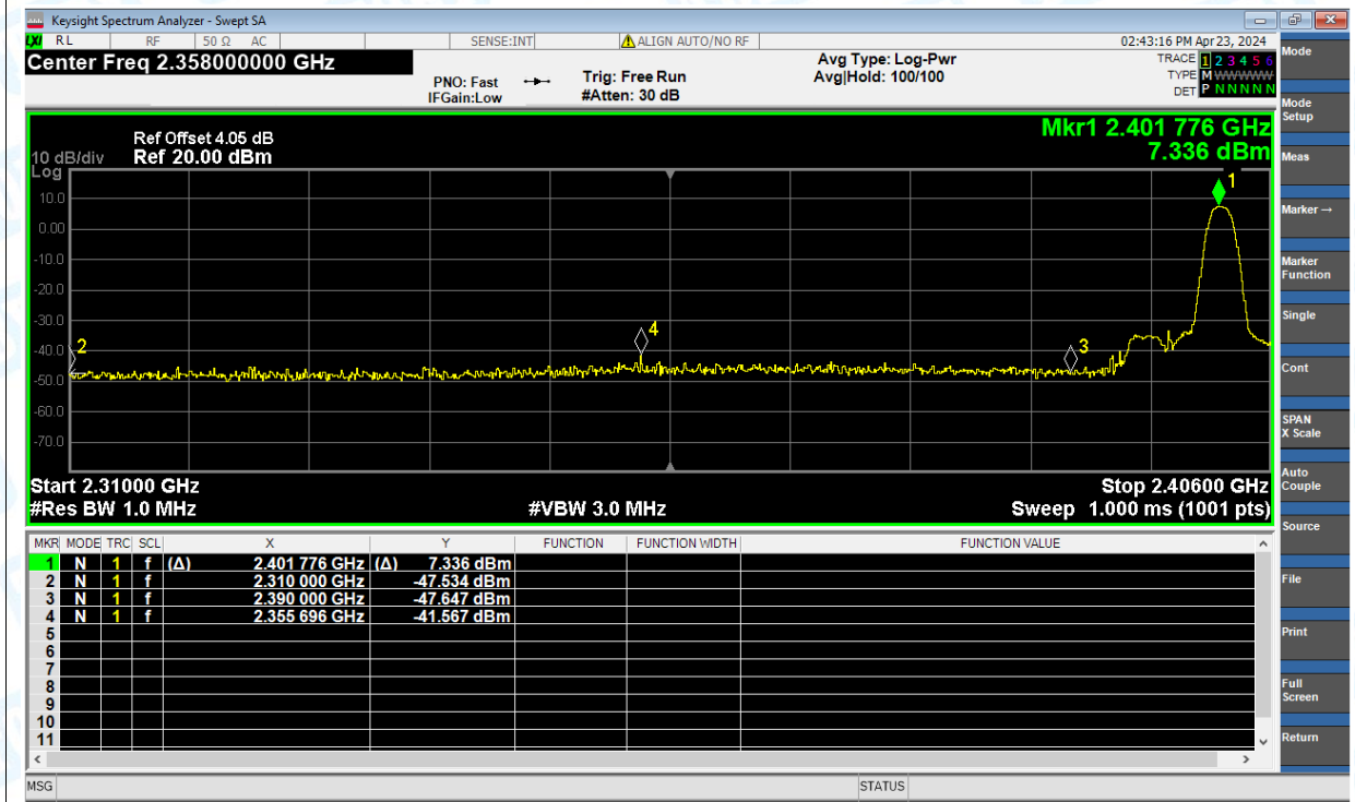
Restrict Band NVNT BLE 1Mbps 2402MHz Ant1 Average
