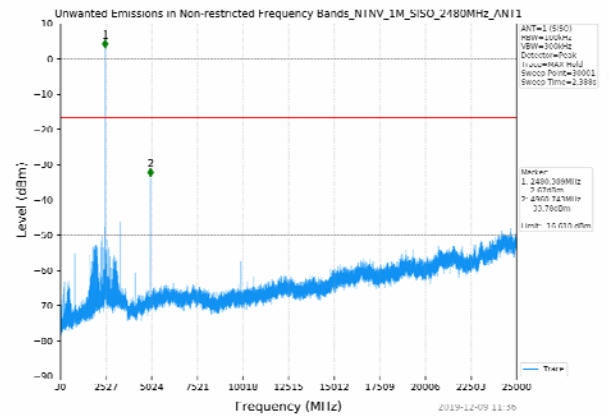
30MHz-25GHz CH39
