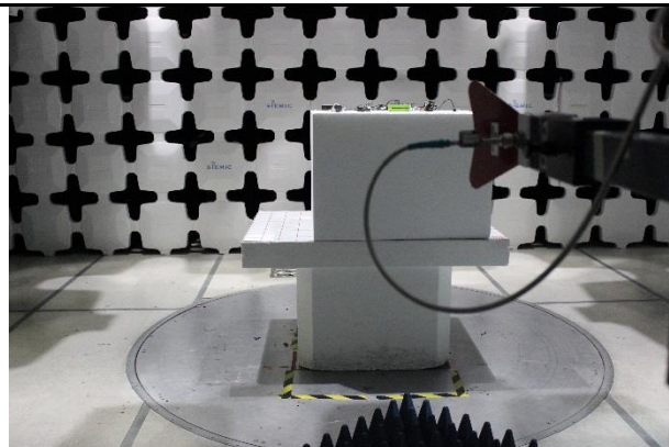
Radiated Emission Above 1G – Rear View
