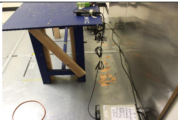
Conducted Emission – Side View
