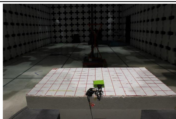
Radiated Emission Below 1G – Front View
