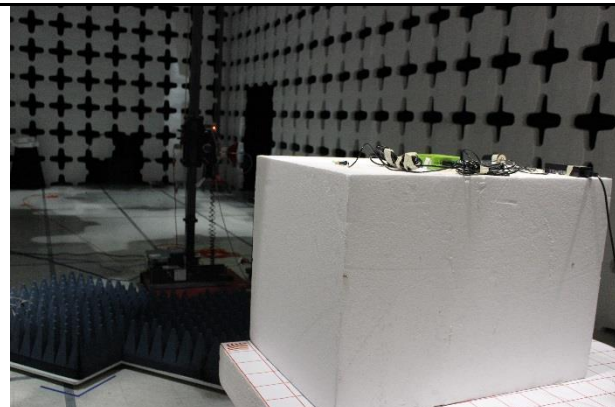
Radiated Emission Above 1G – Front View
