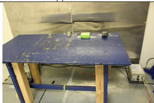
Conducted Emission – Front View
