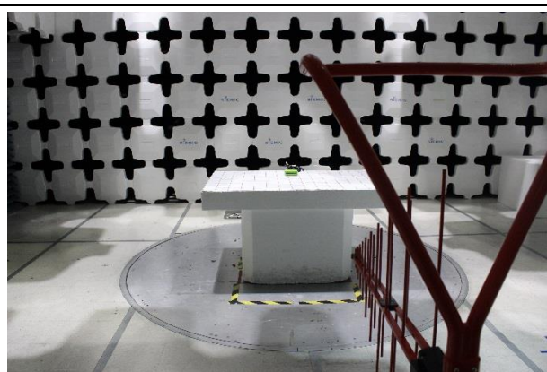
Radiated Emission Below 1G – Rear View
