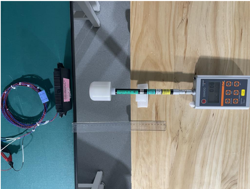
Description: RF Exposure for Electric Field Test Setup
