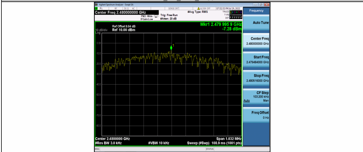
BLE_1M_Ant1_2480
