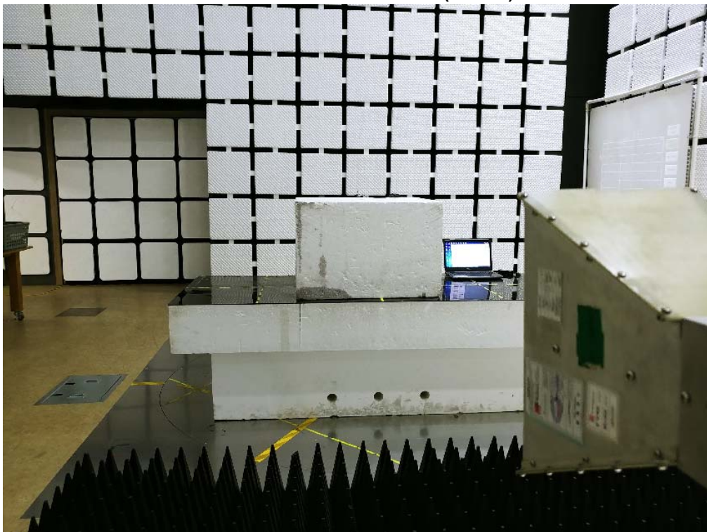
Radiated RF measurement (>1GHz)
