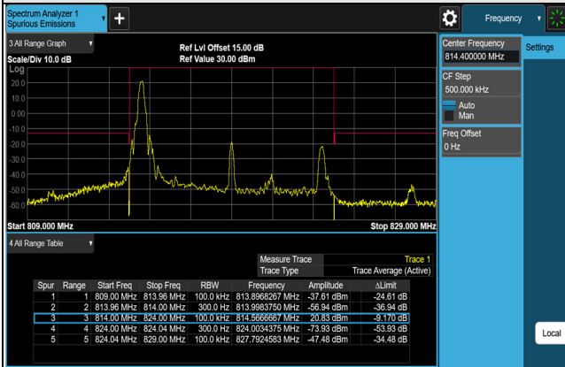
FULL (819MHz)
