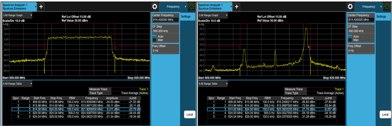
FULL (819MHz)
