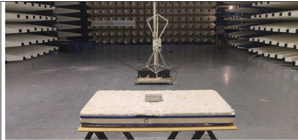
Fig 1b Test setup 30MHz -300MHz Rad Emissions
