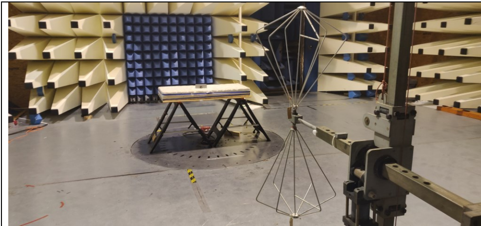
Fig 1a Test setup 30MHz -300MHz Rad Emissions
