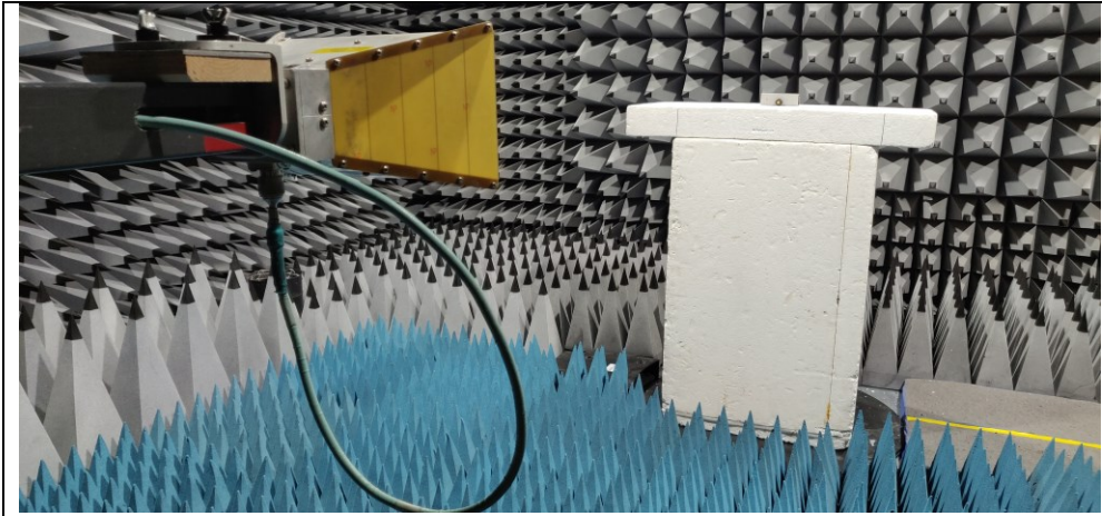
Fig 3 Test setup 1GHz 6GHz Rad Emissions
