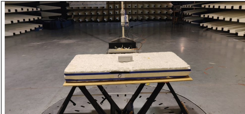
Fig 2b Test setup 300MHz -1GHz Rad Emissions
