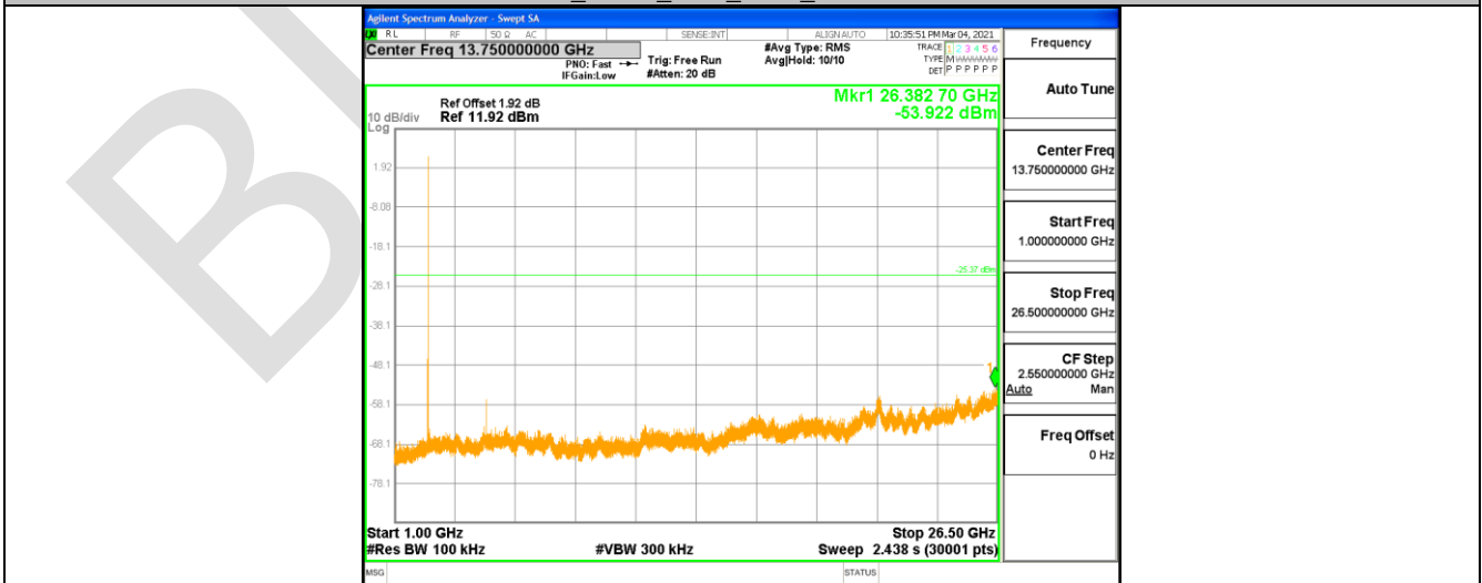
BLE_BT4.0_Ant1_2480_0~Reference
