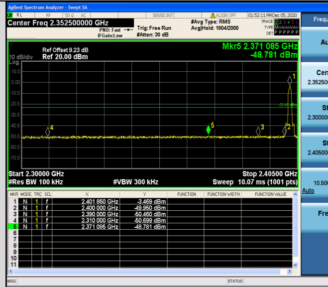
Channel 0 / 2402 MHz – Non-Hopping
