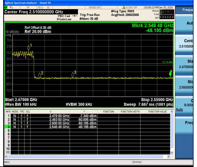
Channel 78 / 2480 MHz – Hopping
