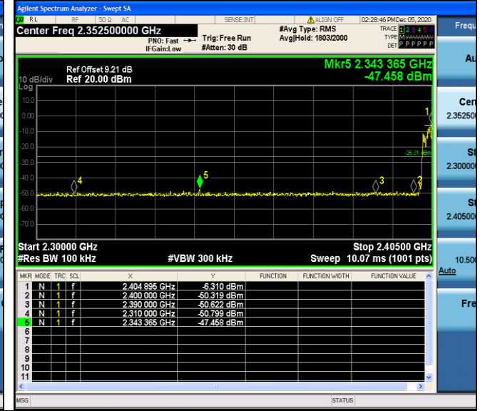
Channel 0 / 2402 MHz – Hopping
