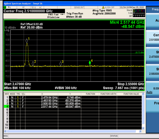
Channel 78 / 2480 MHz – Non-Hopping
