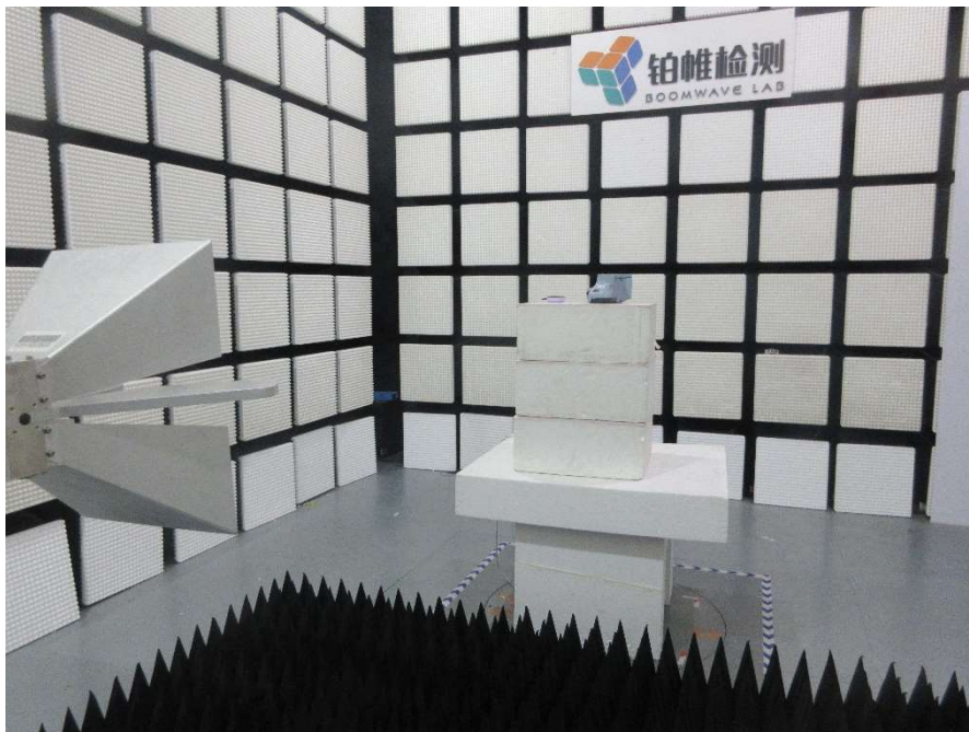
Radiated Emission 1GHz-6GHz (Front view) – Mode 1
