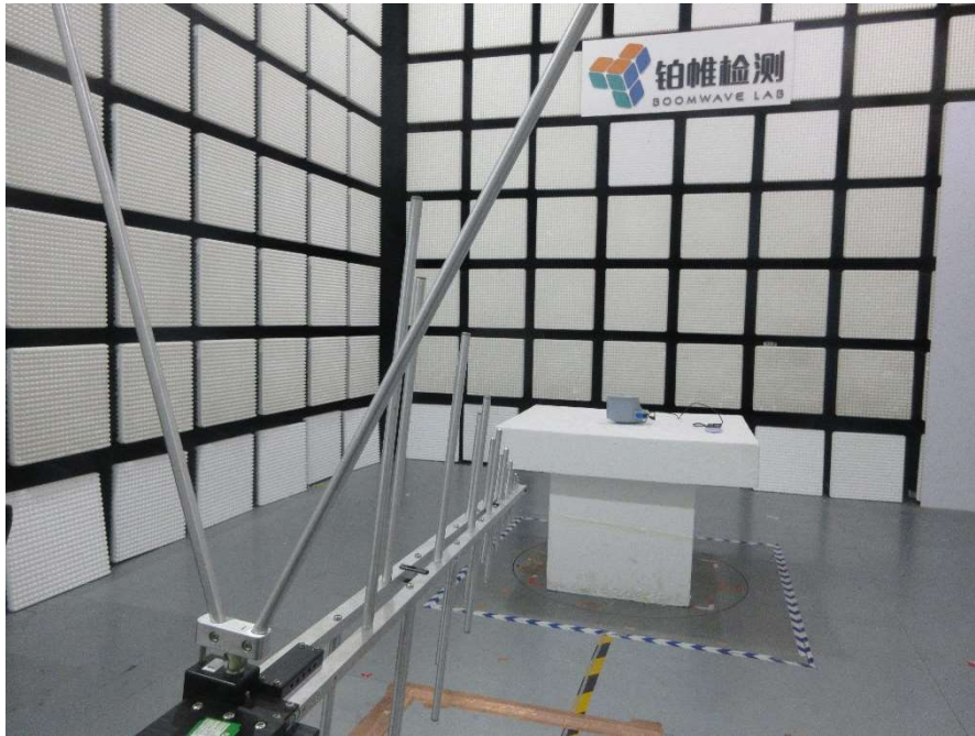
Radiated Emission 30MHz-1GHz – Mode 1
