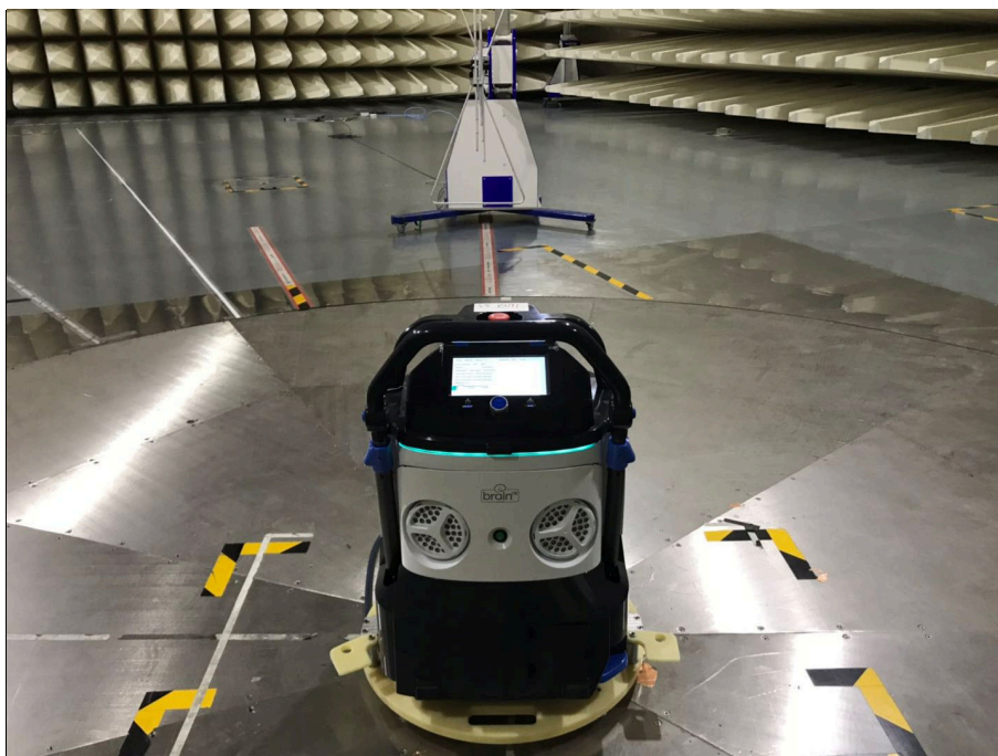
Radiated Emissions Test Setup (operation mode) (30-1000MHz)
