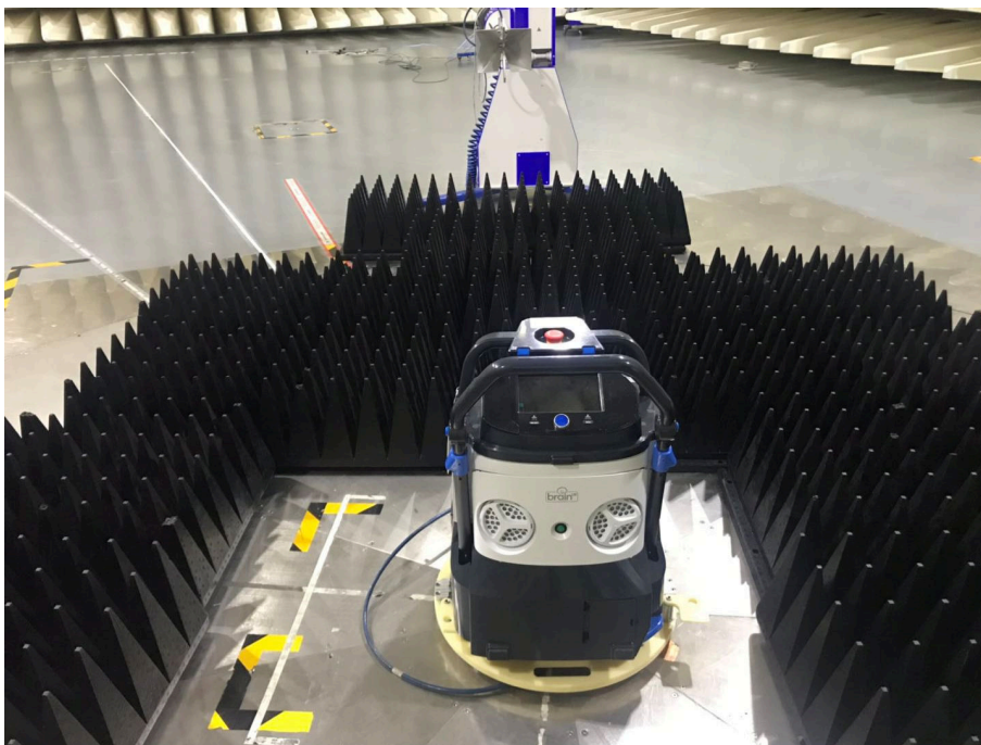
Radiated Emissions Test Setup (operation mode) (above 1GHz)
