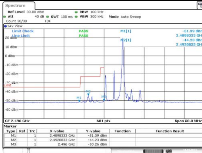
Band41-5MHz-QPSK-39675-1RB#24
