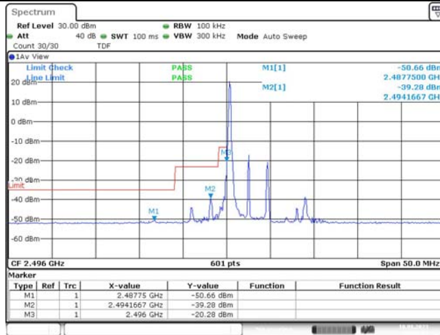
Band41-5MHz-QPSK-39675-1RB#0
