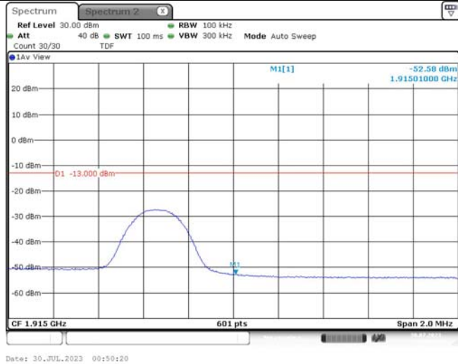
Band25-5MHz-16QAM-26665-1RB#24
