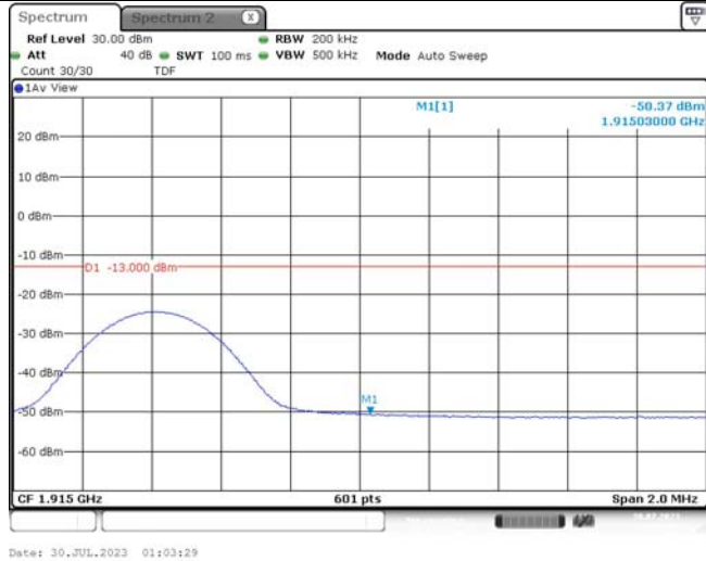
Band25-10MHz-16QAM-26640-1RB#49
