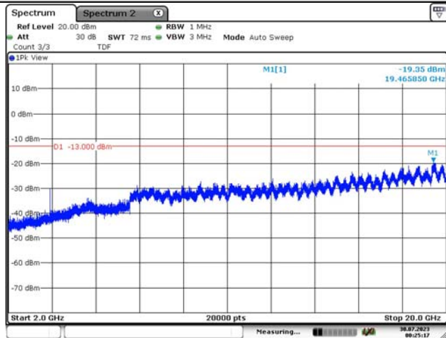
Band25-1.4MHz-QPSK-26047-1RB#0-Range3:2000~20000MHz
