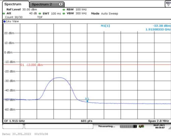
Band25-5MHz-QPSK-26665-1RB#24
