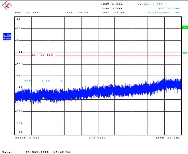
Band2-20MHz-16QAM-19100-1RB#0-Range3:2000~20000MHz
