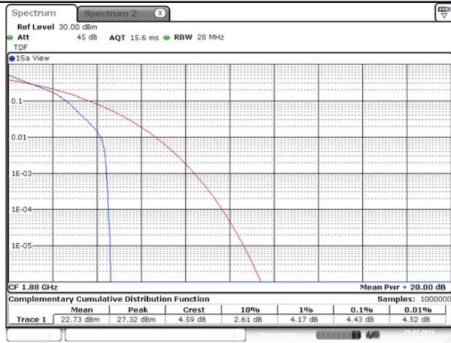
Band2-1.4MHz-QPSK-18900-1RB#0
