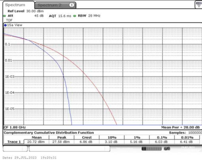
Band2-3MHz-16QAM-19185-1RB#0
