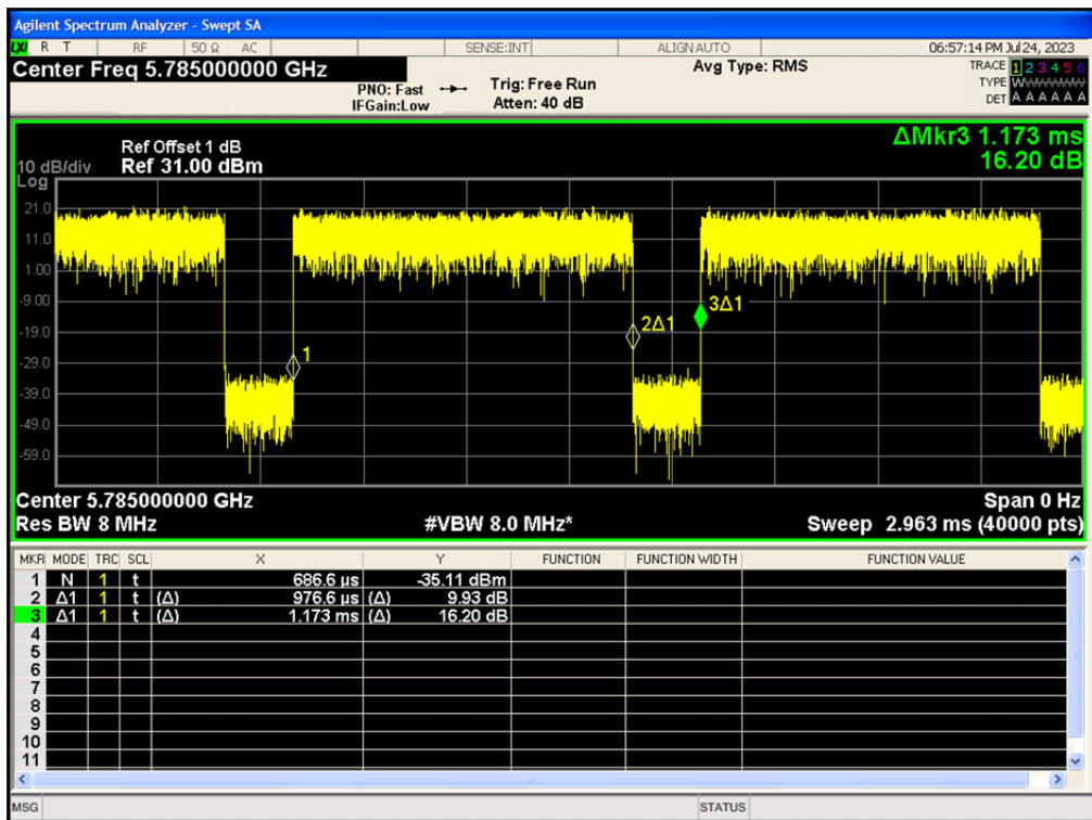
802.11ac(VHT20)_5785
