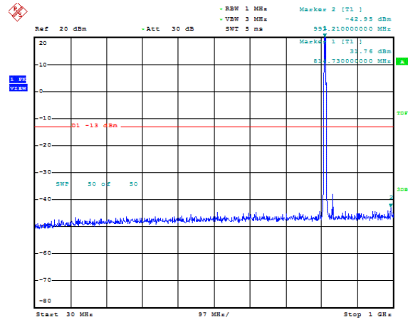
Band26-1.4MHz-QPSK-26697-1RB#0-Range1:30~1000MHz
