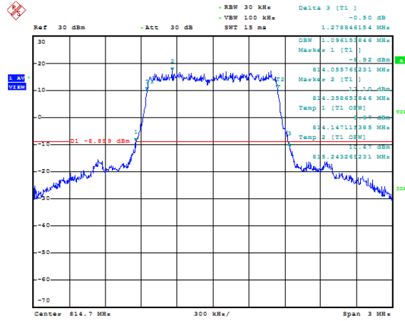
Band26-1.4MHz-QPSK-26697-6RB#0-1.096
