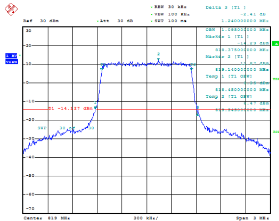
Band26-1.4MHz-QPSK-26740-6RB#0-1.095
