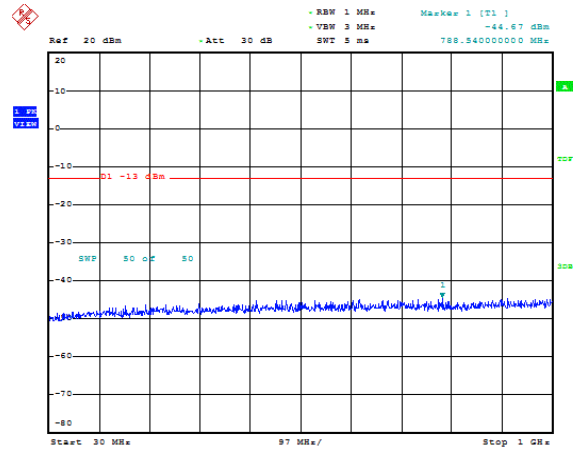
Band25-1.4MHz-QPSK-26047-1RB#0-Range1:30~1000MHz
