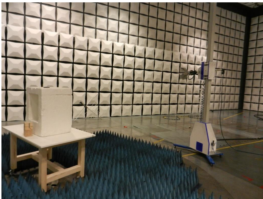
Radiated Emissions above 1 GHz, EUT flat on table
