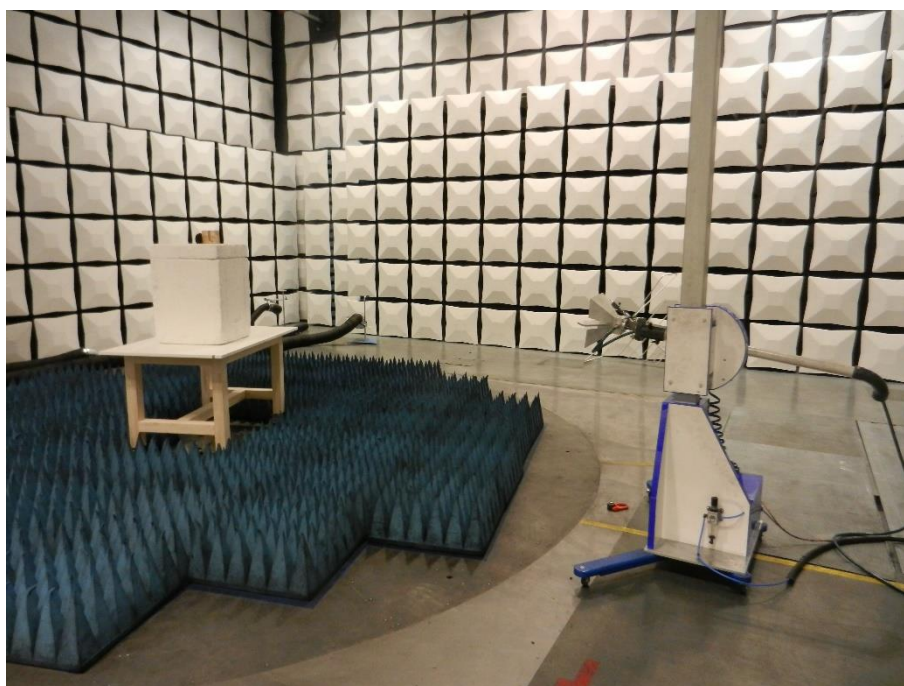
Radiated Emissions above 1 GHz, EUT on long side
