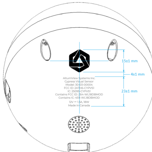
Figure 2 - Label 'A' view with dimensions.
