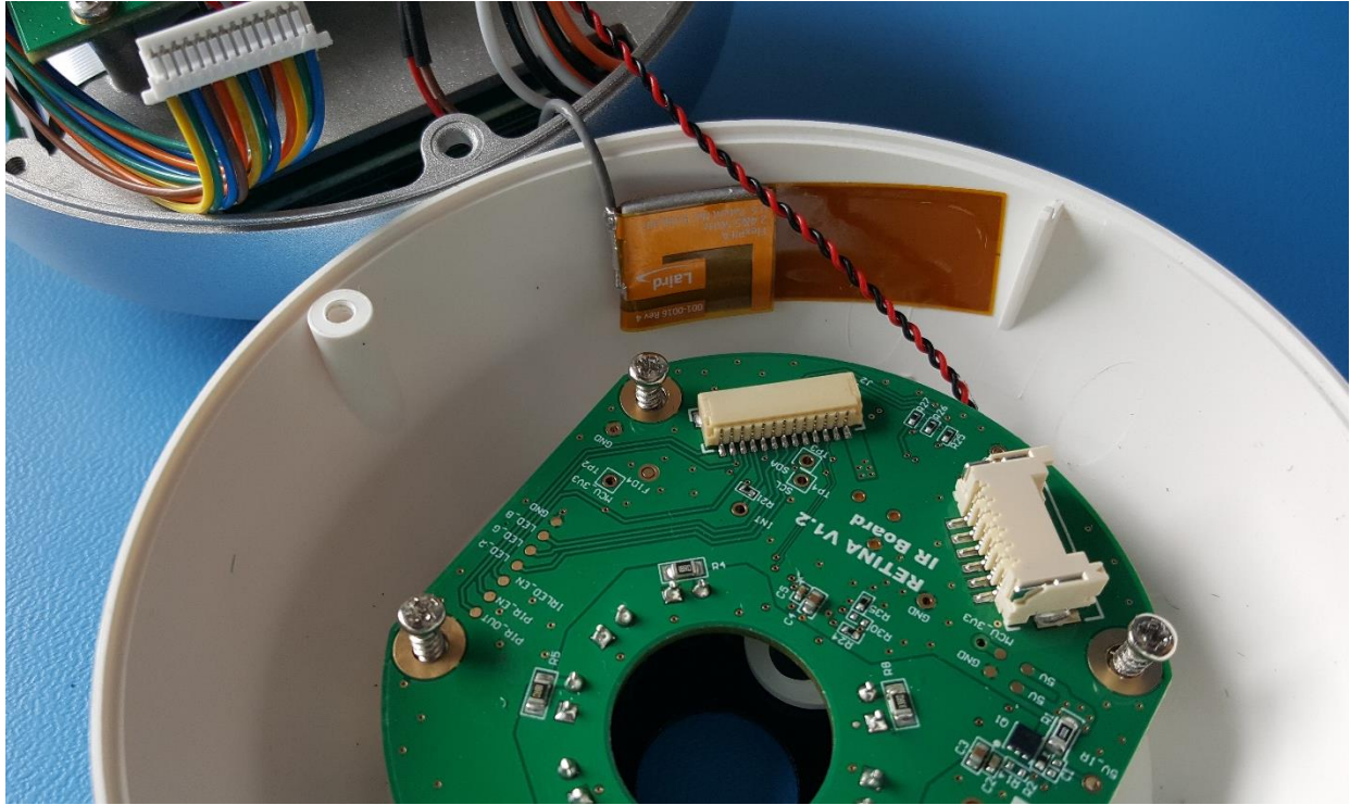
Figure 3 - Wi-Fi antenna
