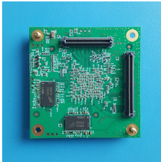
Figure 20 - CPU board rear view
