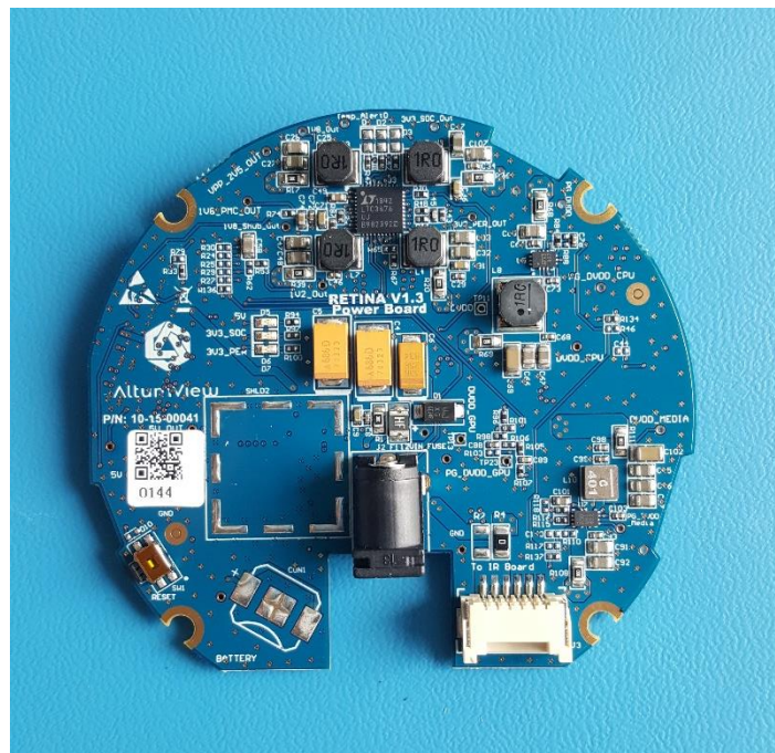
Figure 16 - Power board rear view
