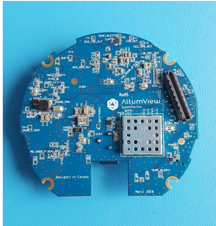
Figure 15 - Power board front view
