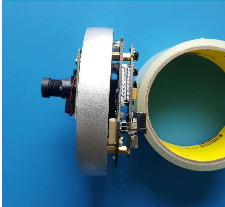
Figure 7 - Side view without enclosure
