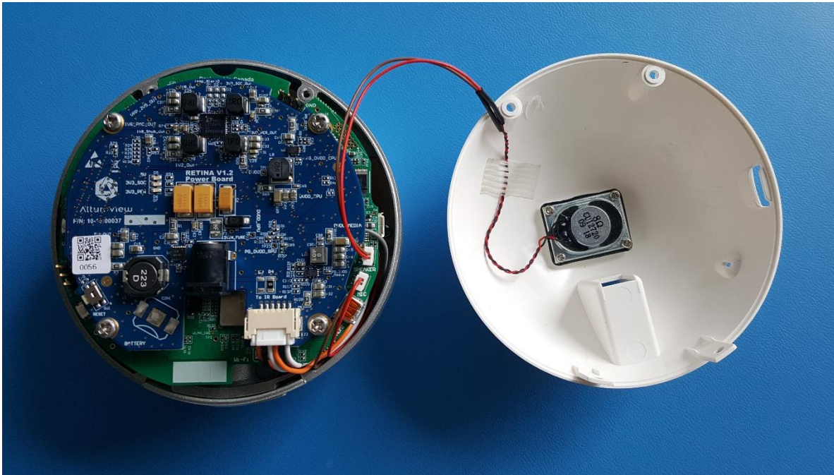
Figure 1 - Rear enclosure disassembled
