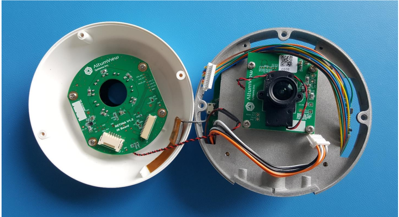
Figure 2 - Front enclosure disassembled
