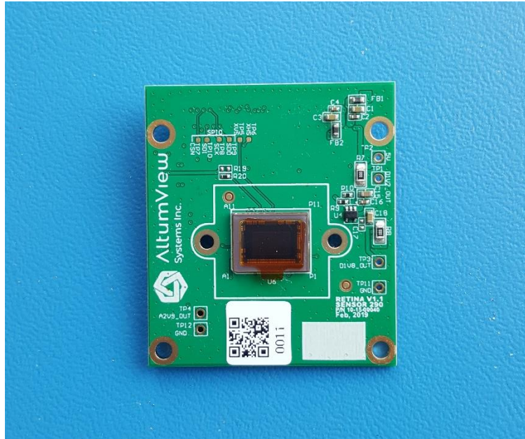
Figure 13 - Sensor board front view
