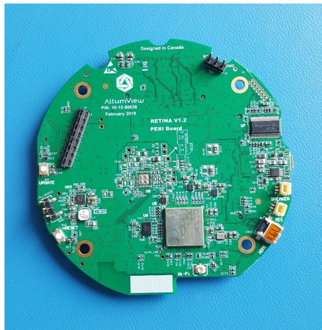
Figure 18 - Peri board rear view
