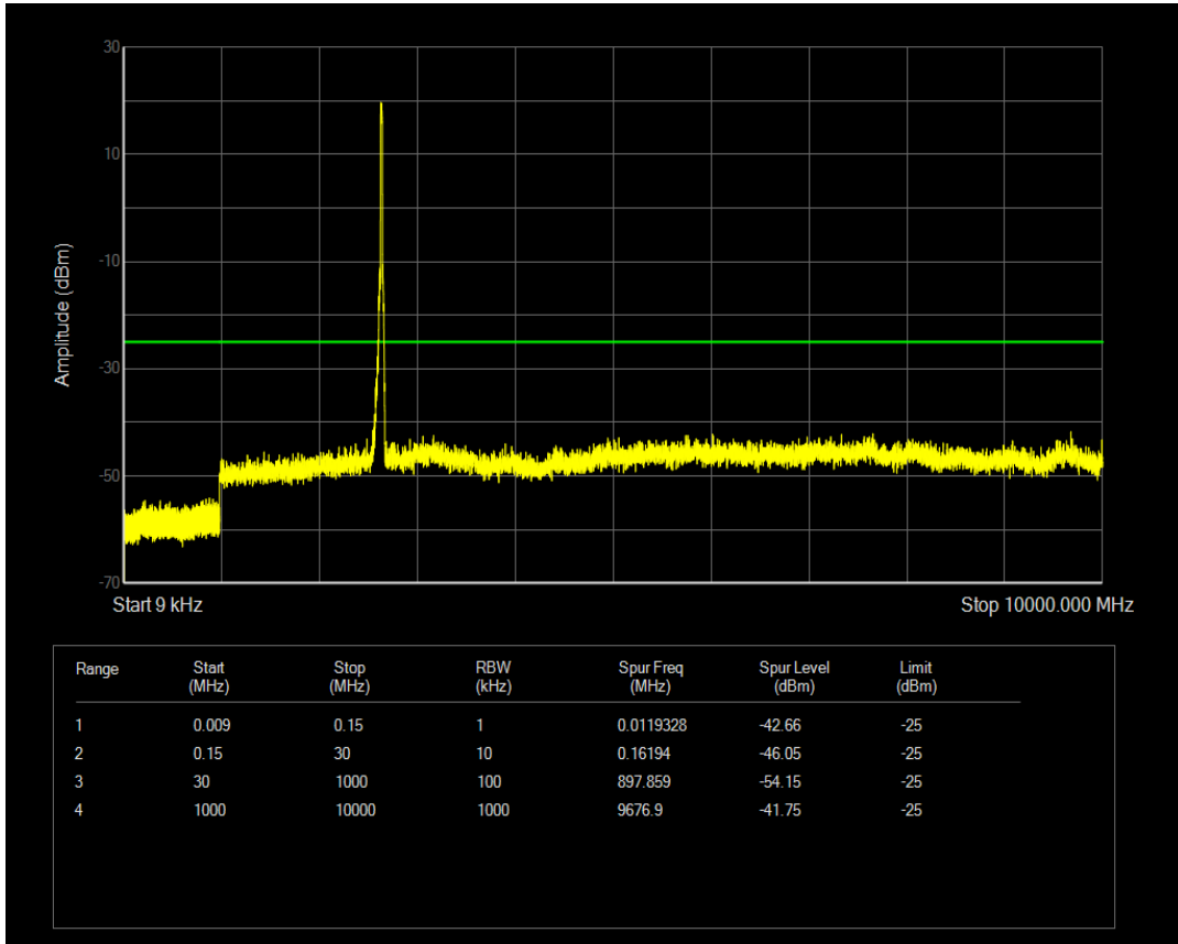
Band41 QAM16 BW=20MHz Channel=41190 RB Size=1 Position=#0
