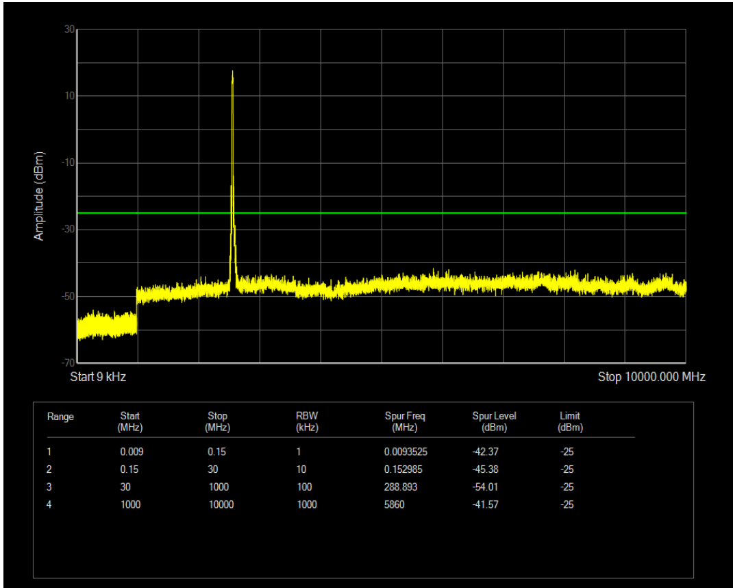
Band41 QAM16 BW=20MHz Channel=40390 RB Size=100 Position=#0
