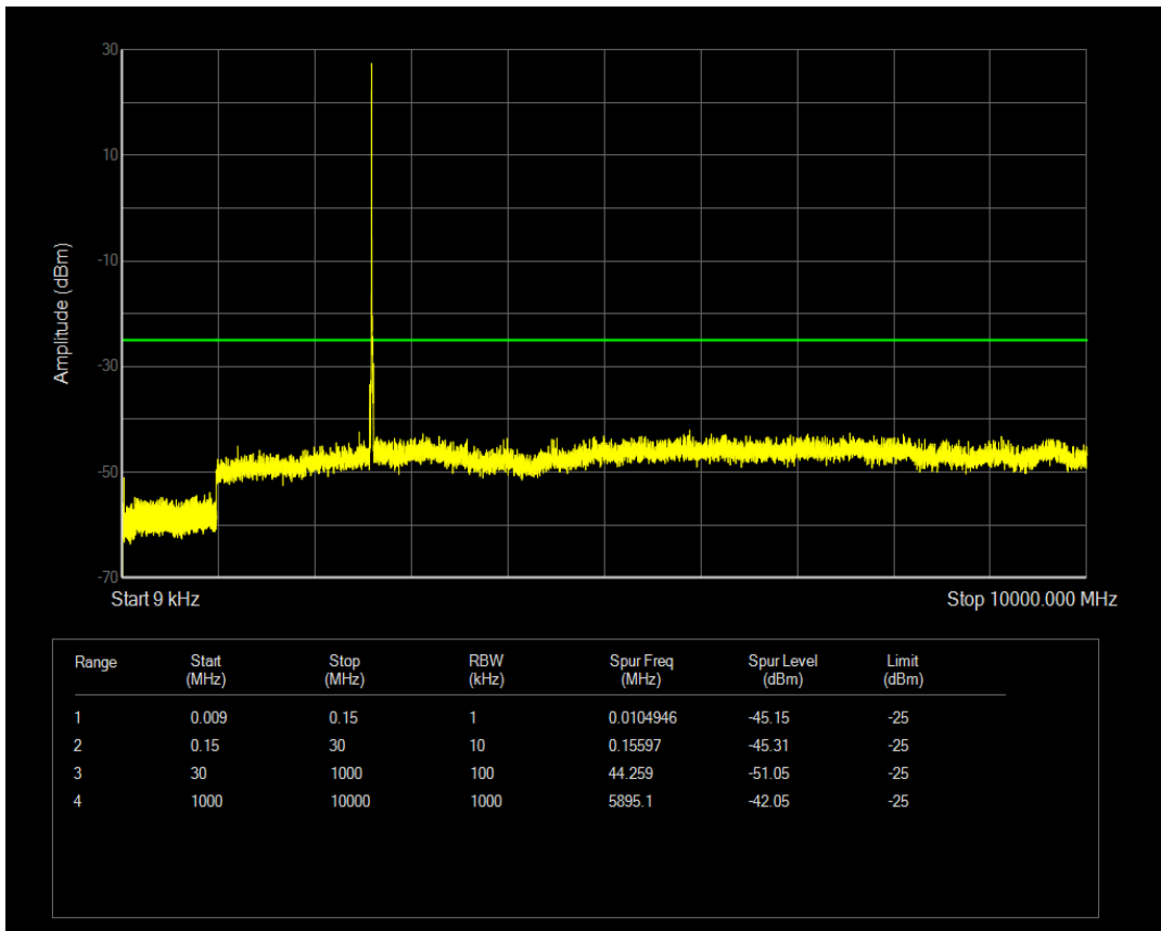
Band41 QPSK BW=10MHz Channel=41240 RB Size=1 Position=#0
