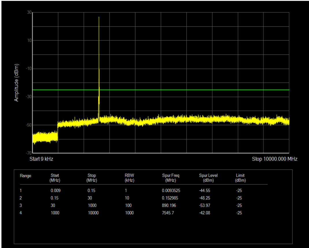
Band41 QAM16 BW=10MHz Channel=40790 RB Size=1 Position=#0
