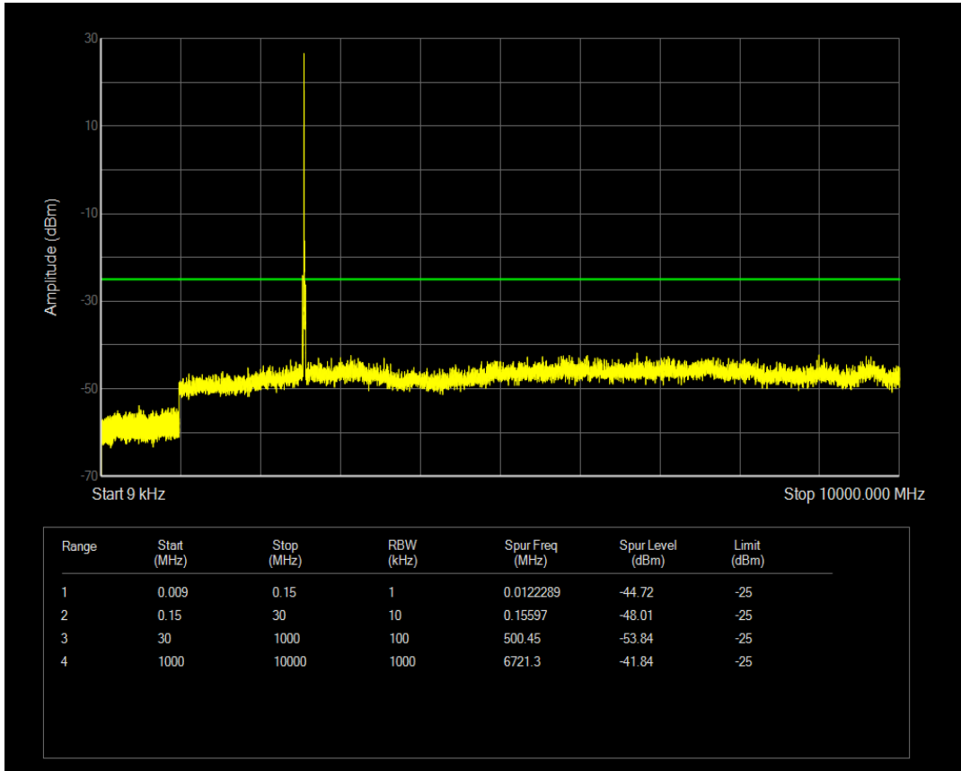
Band41 QAM16 BW=5MHz Channel=41265 RB Size=25 Position=#0
