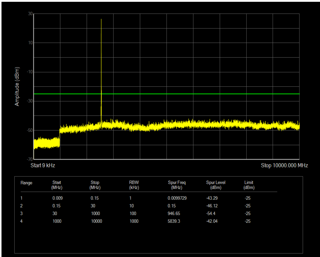
Band41 QPSK BW=5MHz Channel=40315 RB Size=25 Position=#0
