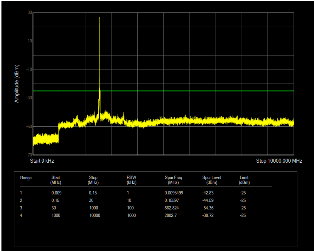
Band41 QAM16 BW=15MHz Channel=41215 RB Size=75 Position=#0
