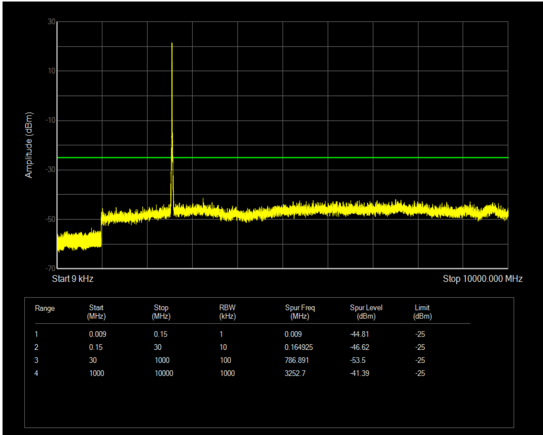
Band41 QPSK BW=10MHz Channel=40790 RB Size=50 Position=#0
