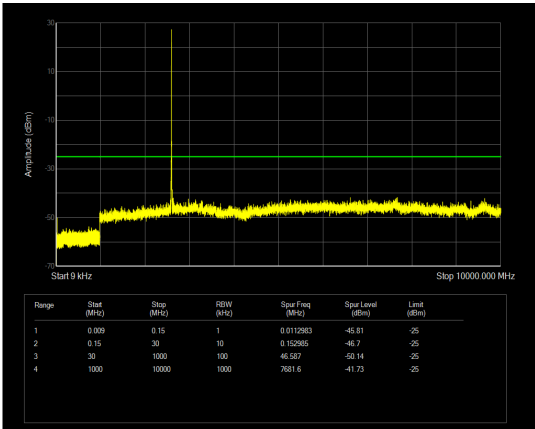
Band41 QAM16 BW=5MHz Channel=40790 RB Size=1 Position=#0
