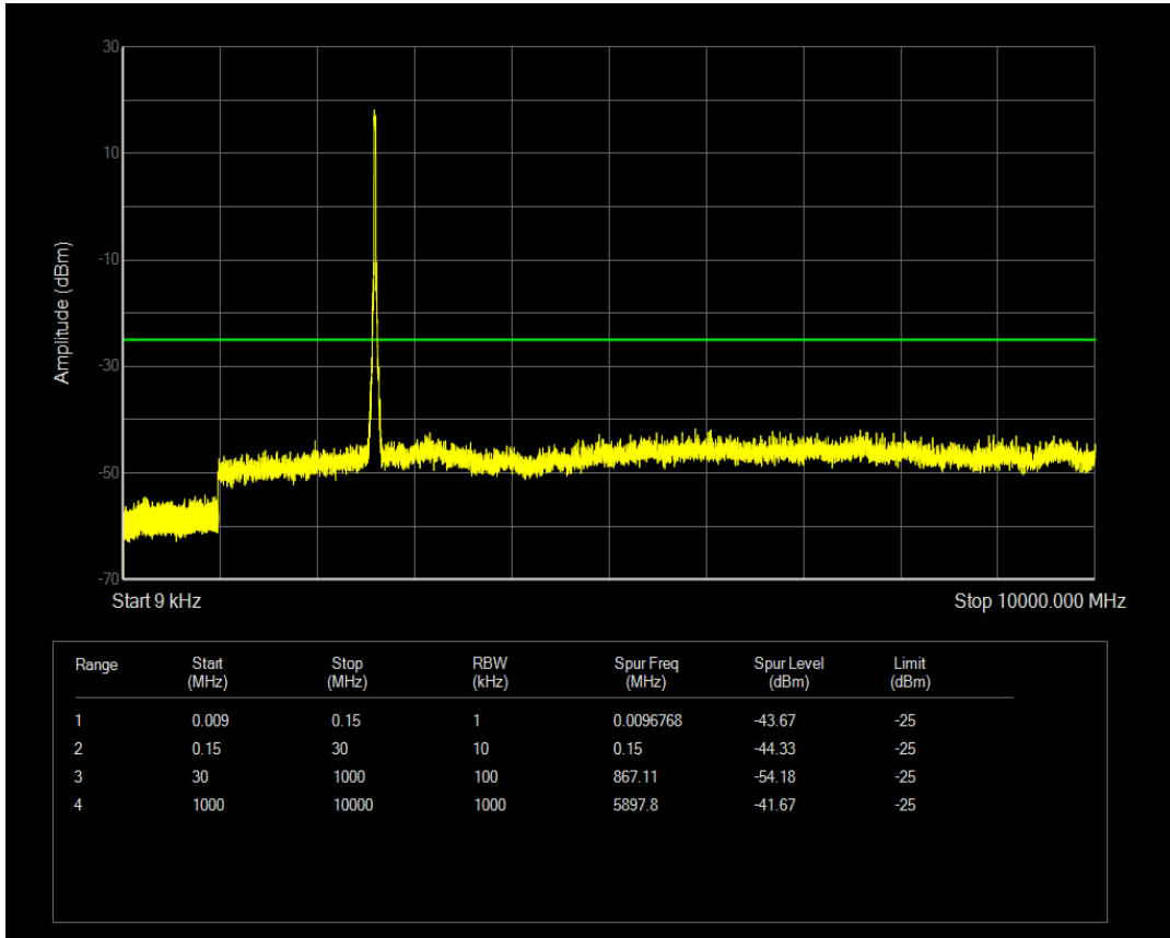
Band41 QPSK BW=20MHz Channel=41190 RB Size=1 Position=#0
