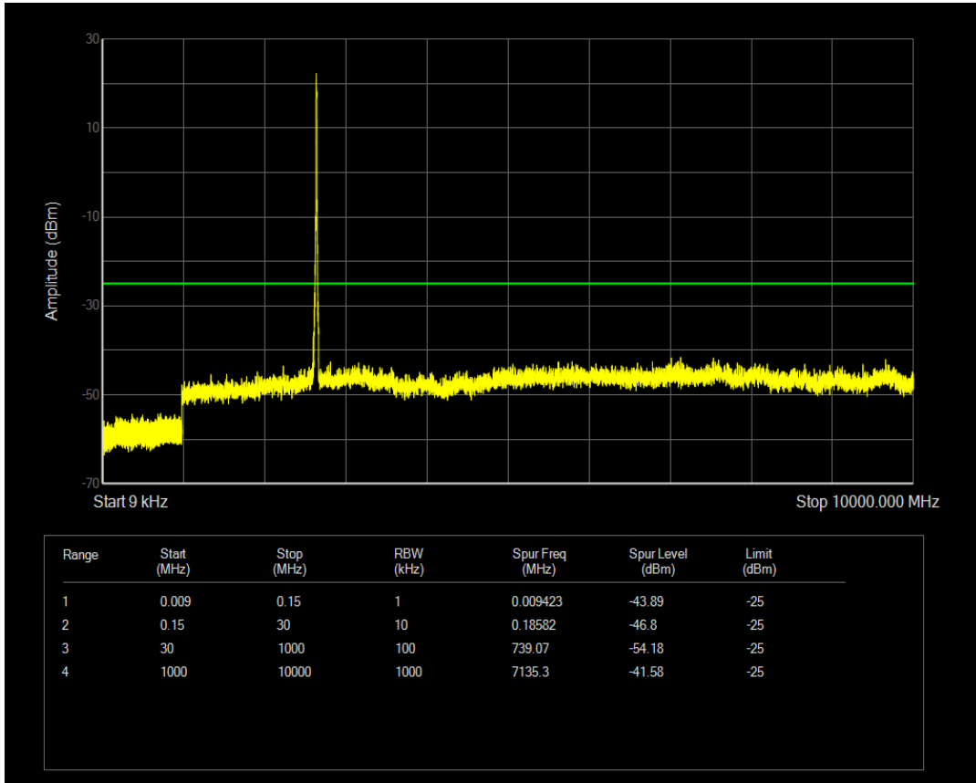
Band41 QPSK BW=15MHz Channel=40365 RB Size=75 Position=#0
