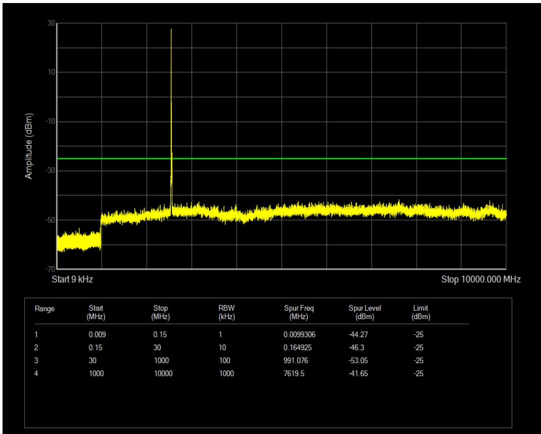
Band41 QAM16 BW=10MHz Channel=40340 RB Size=50 Position=#0
