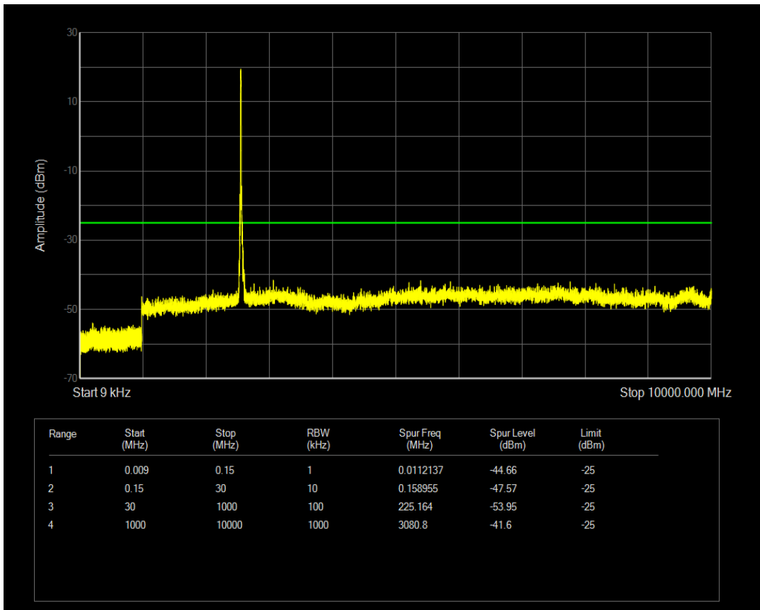
Band41 QPSK BW=15MHz Channel=40790 RB Size=75 Position=#0
