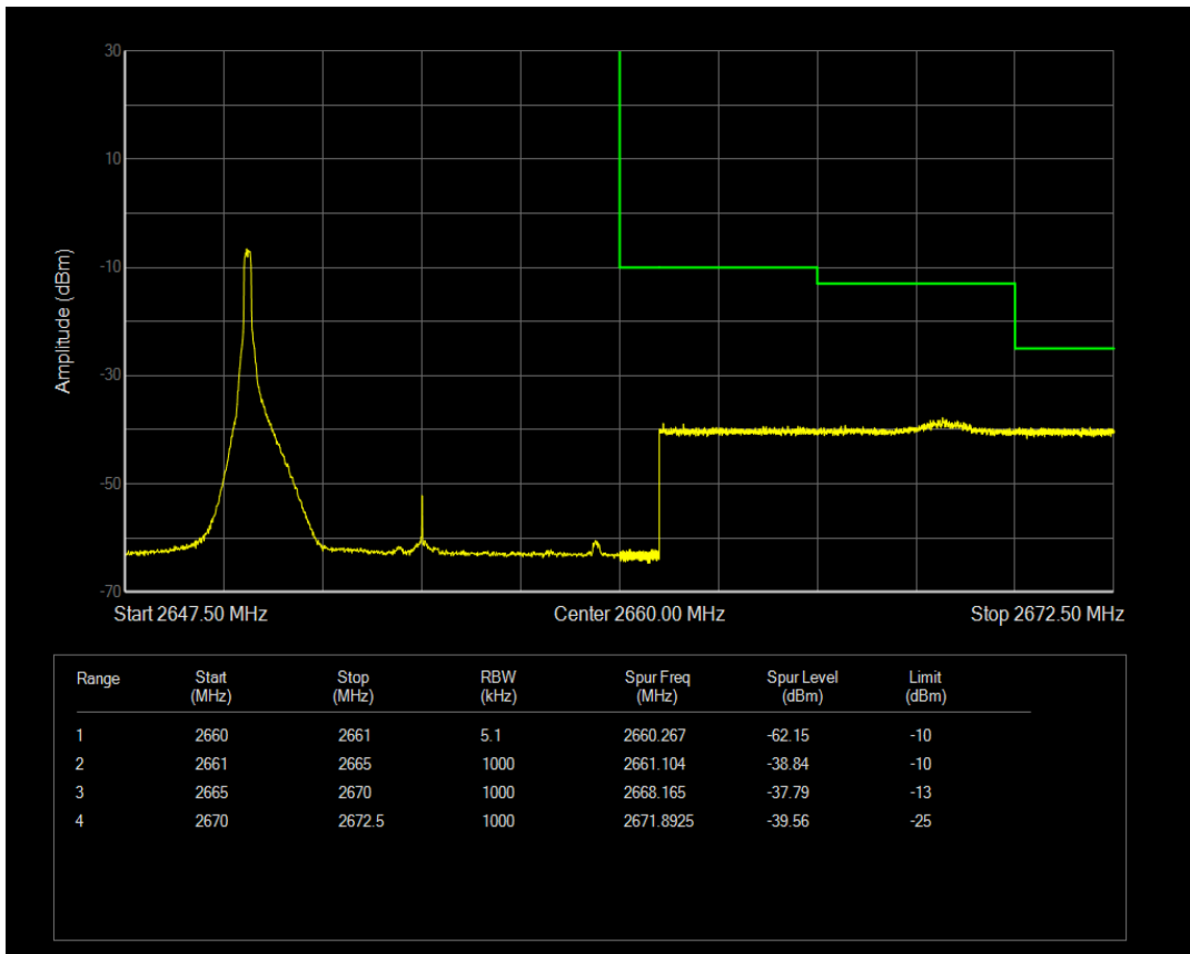
Band41 QPSK BW=10MHz Channel=41240 RB Size=1 Position=#Max
