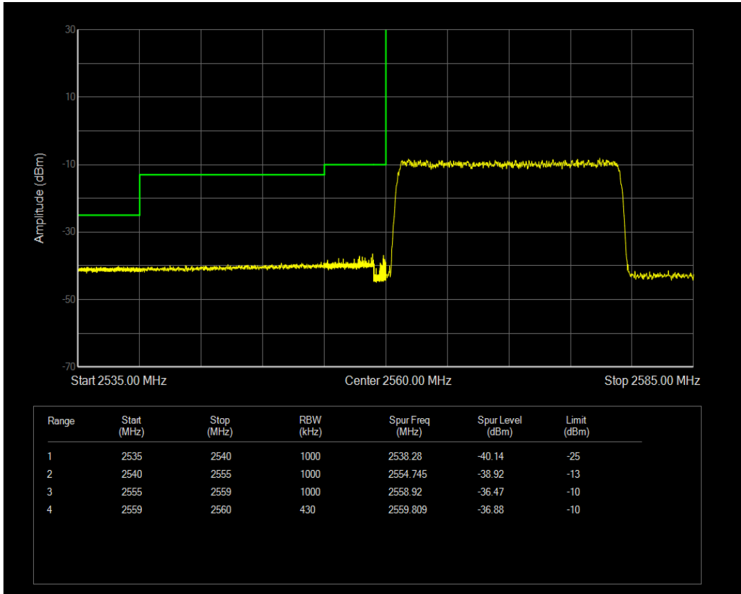
Band41 QPSK BW=20MHz Channel=40390 RB Size=1 Position=#Max
