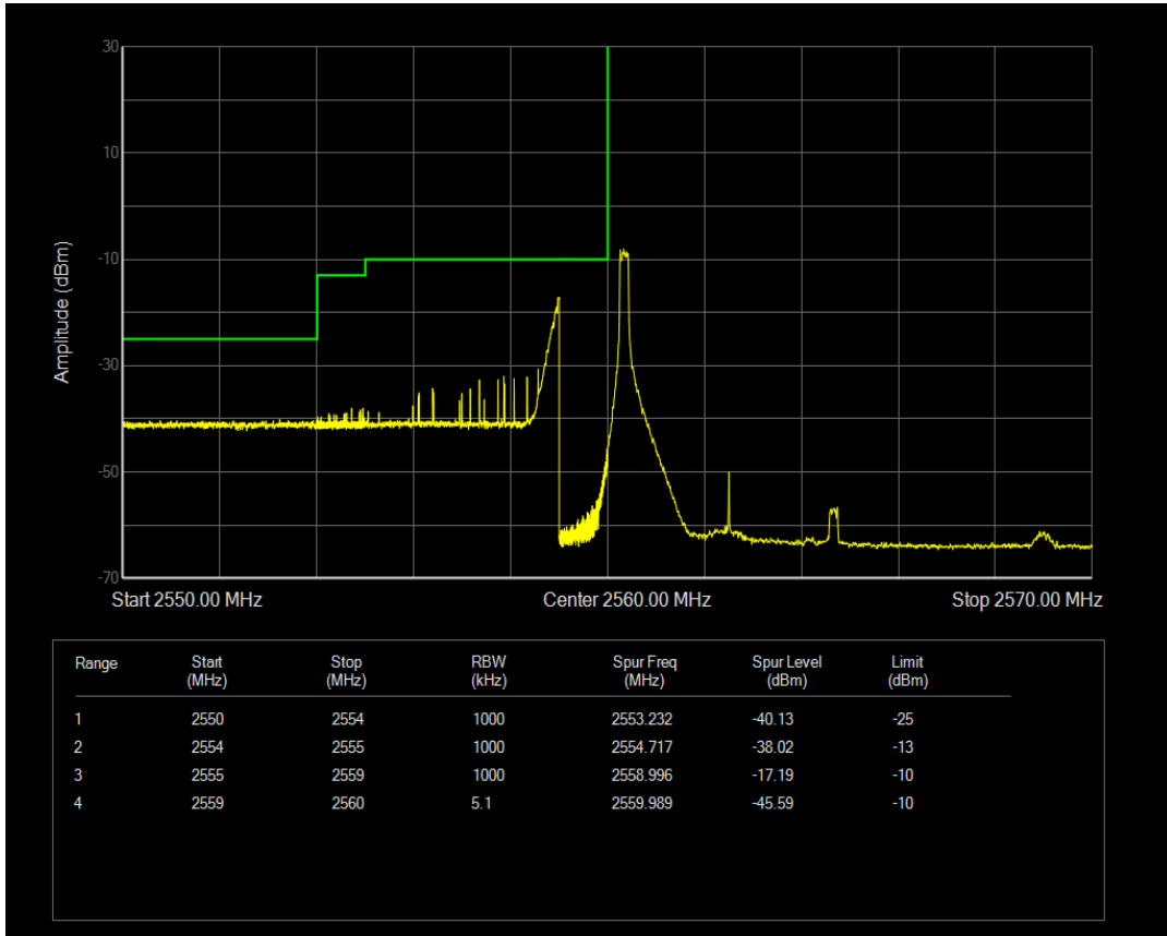
Band41 QAM16 BW=5MHz Channel=40315 RB Size=1 Position=#Max
