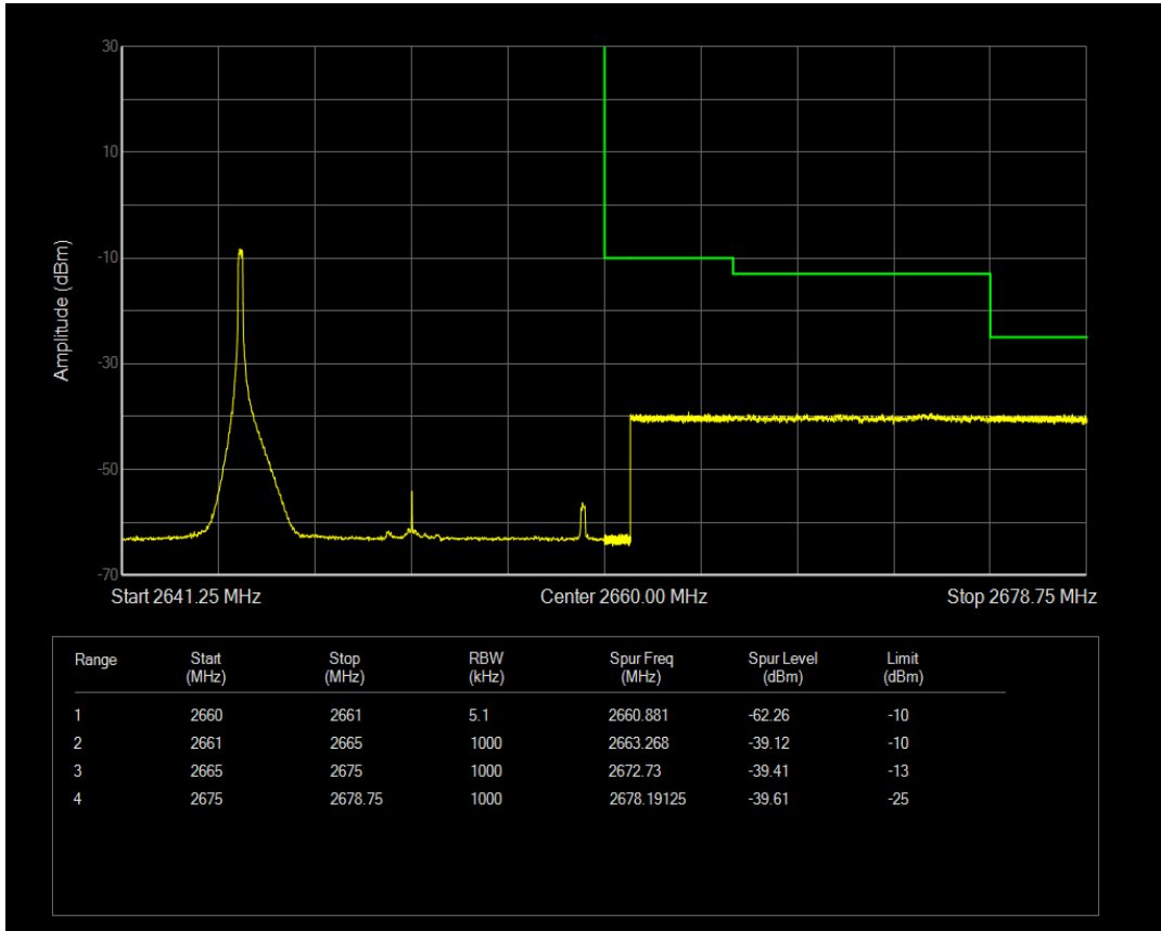
Band41 QAM16 BW=15MHz Channel=41215 RB Size=1 Position=#Max
