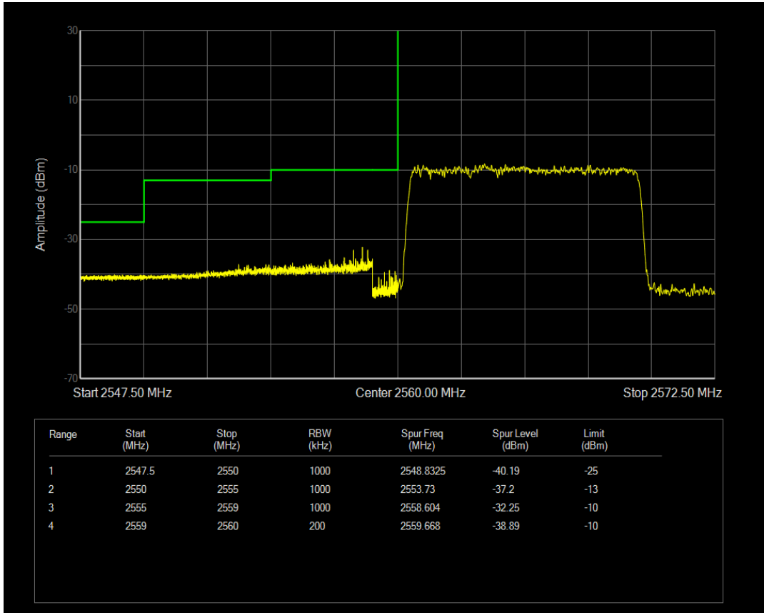
Band41 QAM16 BW=10MHz Channel=40340 RB Size=1 Position=#Max
