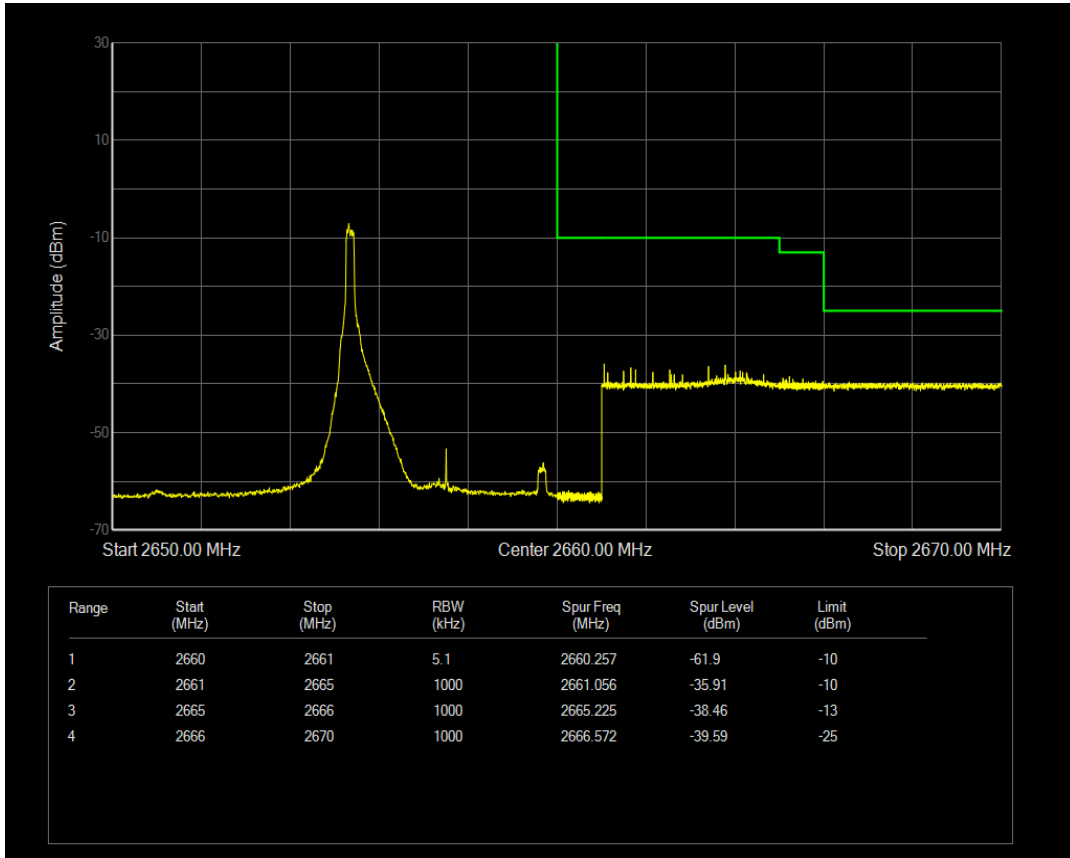
Band41 QAM16 BW=5MHz Channel=41265 RB Size=1 Position=#Max
