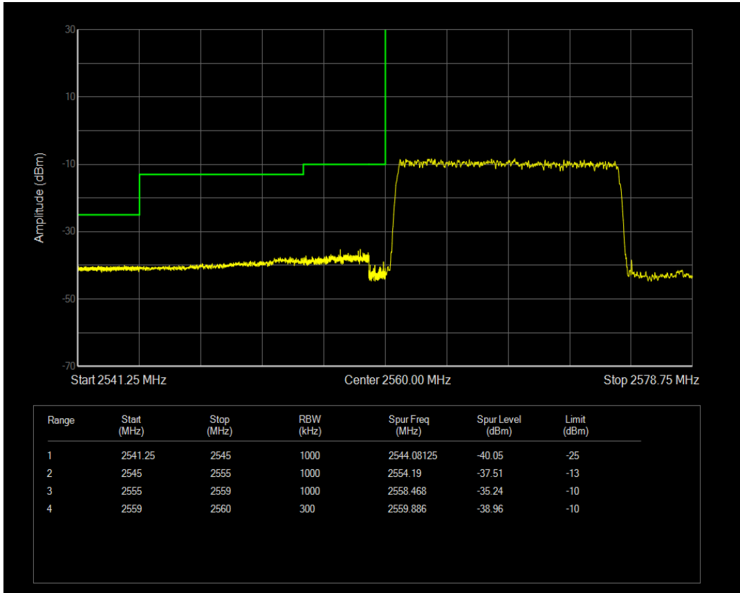
Band41 QPSK BW=15MHz Channel=40365 RB Size=1 Position=#Max
