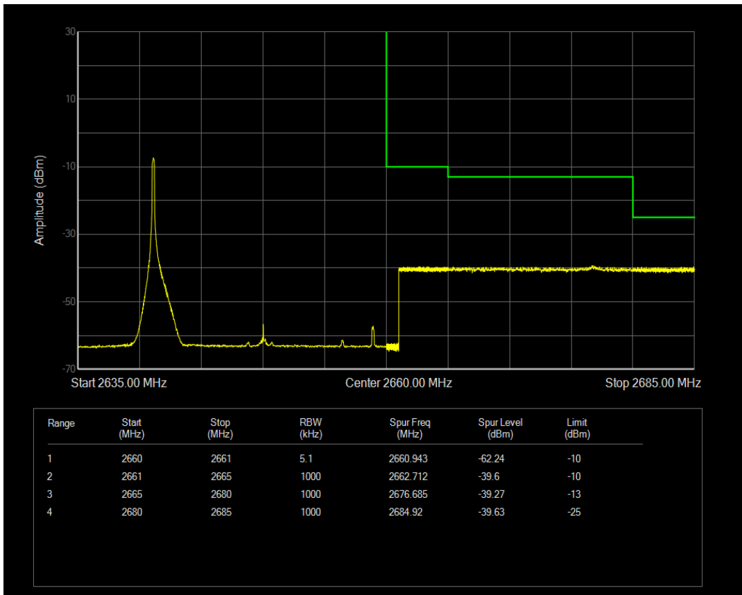
Band41 QPSK BW=20MHz Channel=41190 RB Size=1 Position=#Max
