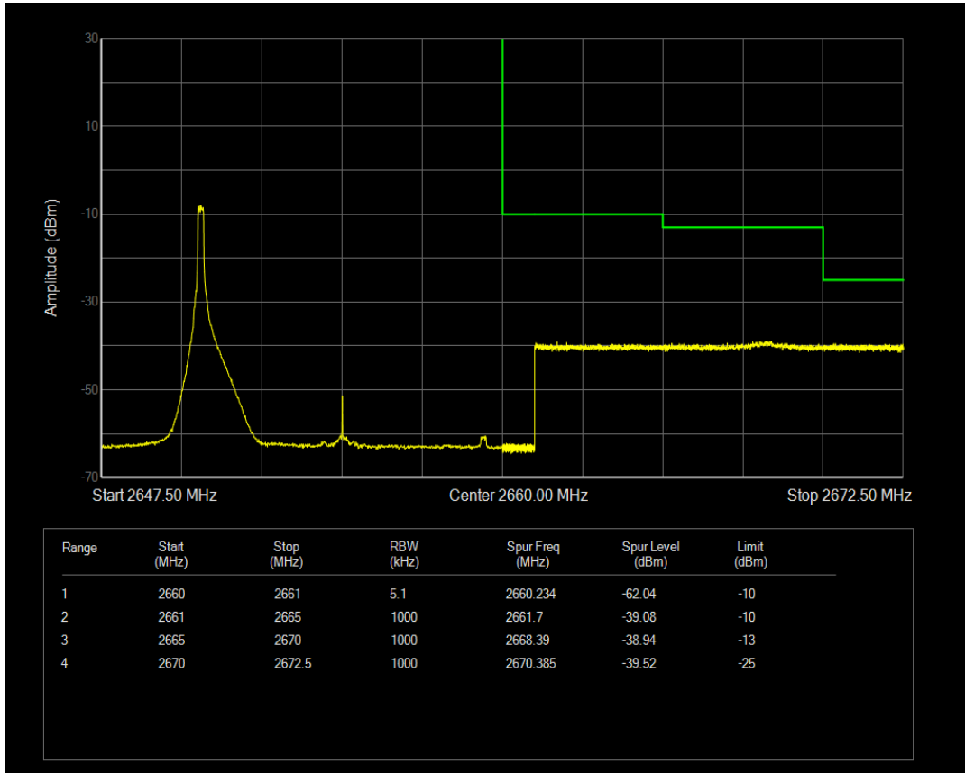
Band41 QAM16 BW=10MHz Channel=41240 RB Size=1 Position=#Max
