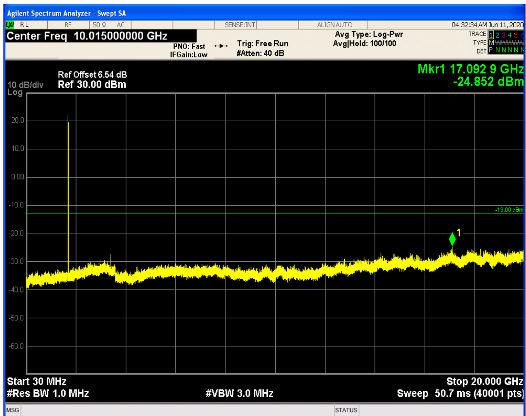
LTE Band66 QPSK BW=5MHz Channel=132647 RB Size=25 Position=#0
