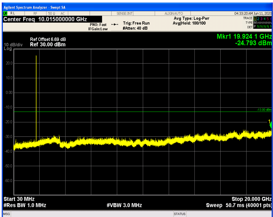
LTE Band66 QAM16 BW=5MHz Channel=132647 RB Size=1 Position=#0
