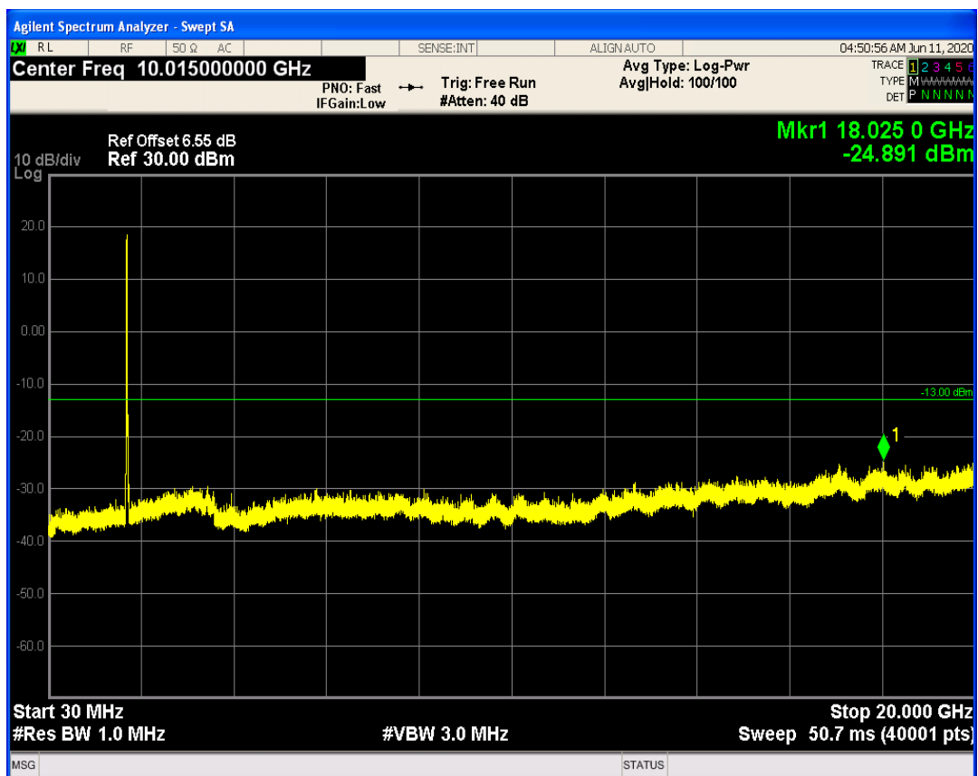
LTE Band66 QPSK BW=20MHz Channel=132572 RB Size=1 Position=#0
