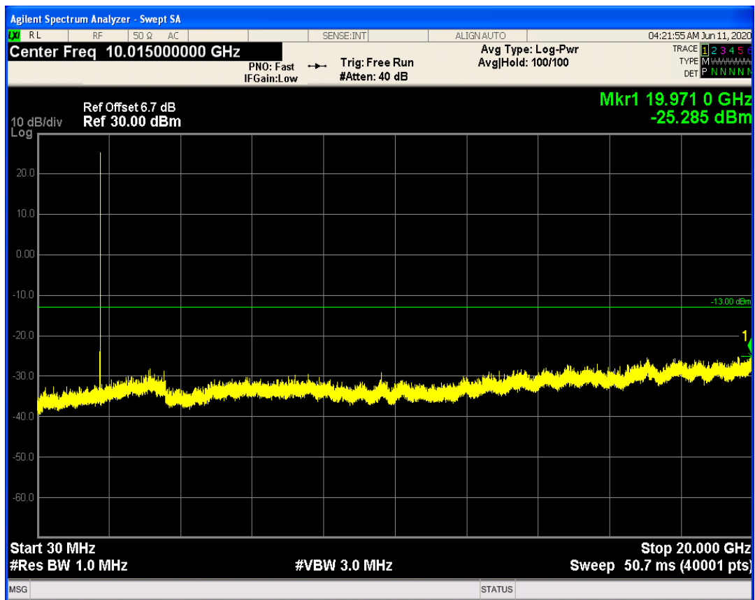
LTE Band66 QAM16 BW=1.4MHz Channel=132665 RB Size=1 Position=#0
