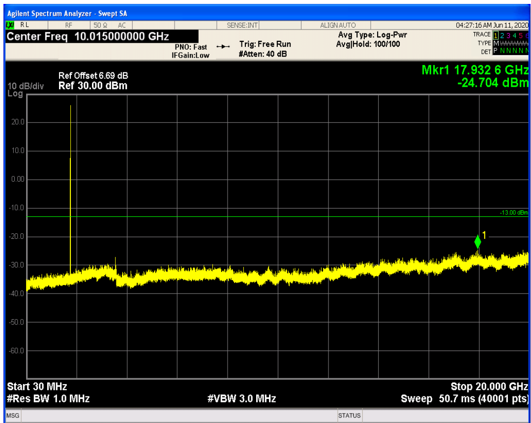
LTE Band66 QPSK BW=3MHz Channel=132657 RB Size=15 Position=#0
