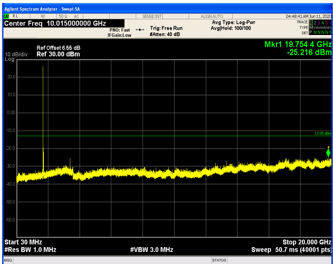
LTE Band66 QAM16 BW=15MHz Channel=132597 RB Size=75 Position=#0
