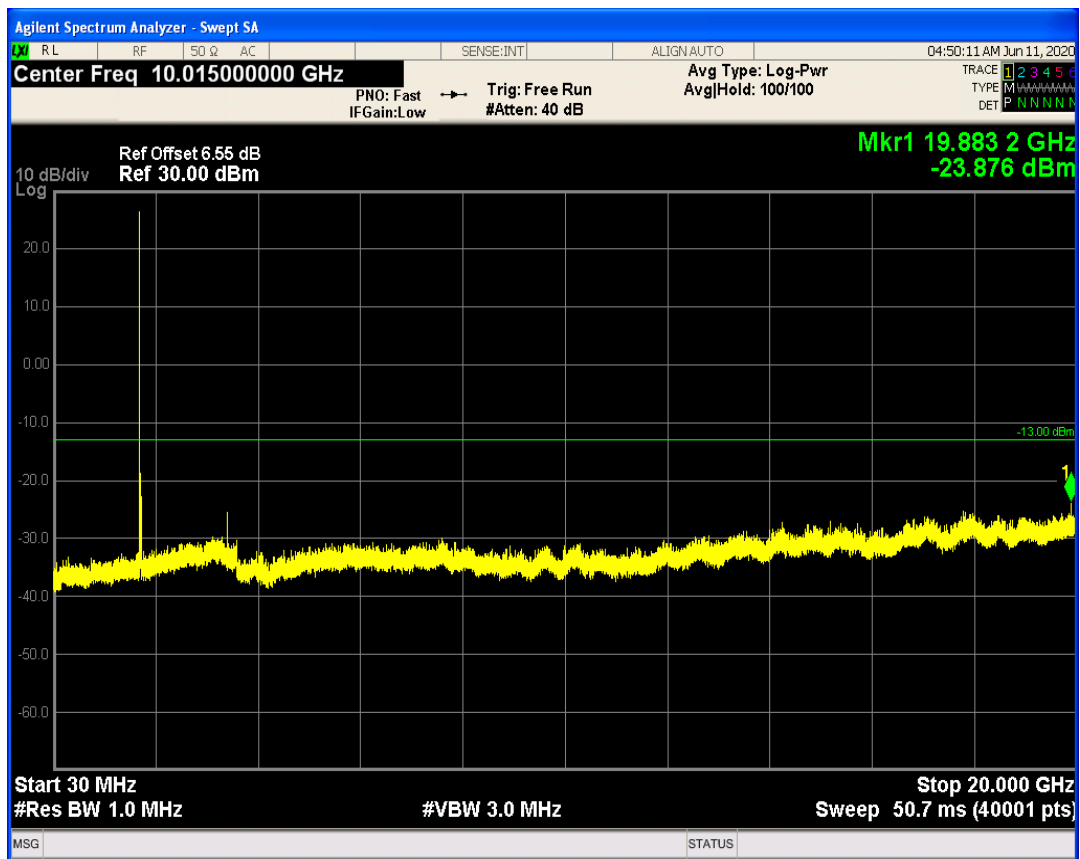
LTE Band66 QAM16 BW=20MHz Channel=132072 RB Size=100 Position=#0
