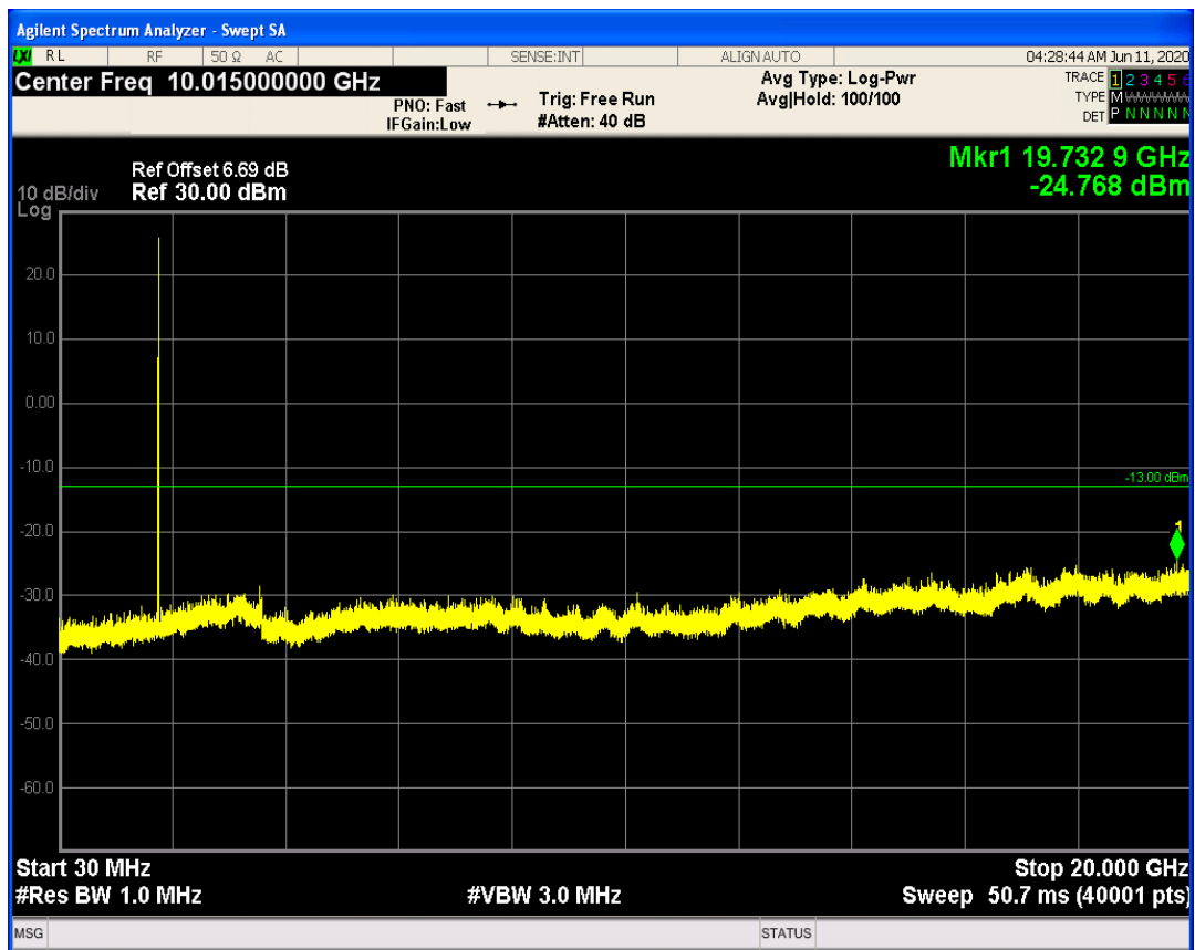
LTE Band66 QPSK BW=5MHz Channel=131997 RB Size=1 Position=#0
