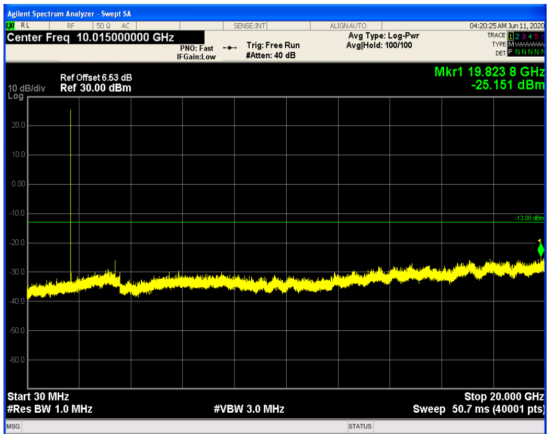
LTE Band66 QPSK BW=1.4MHz Channel=132665 RB Size=1 Position=#0
