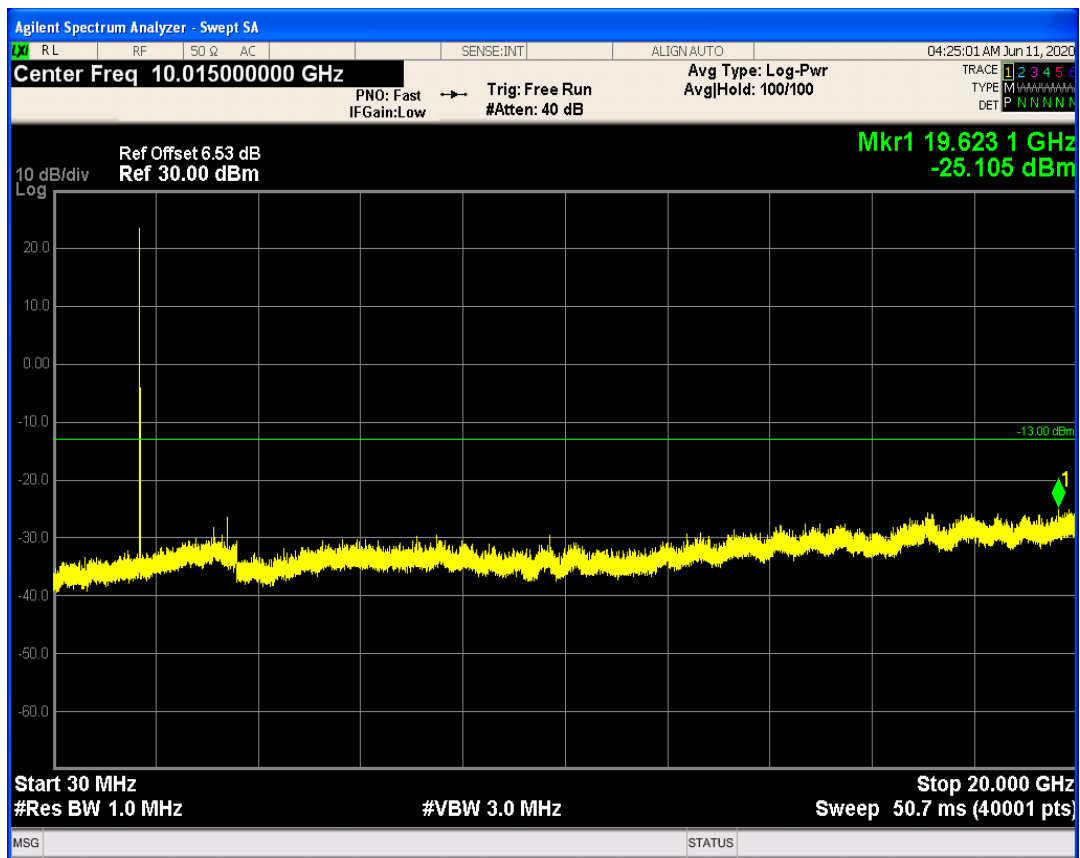
LTE Band66 QAM16 BW=3MHz Channel=131987 RB Size=15 Position=#0
