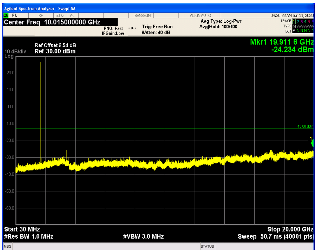
LTE Band66 QAM16 BW=3MHz Channel=132657 RB Size=15 Position=#0
