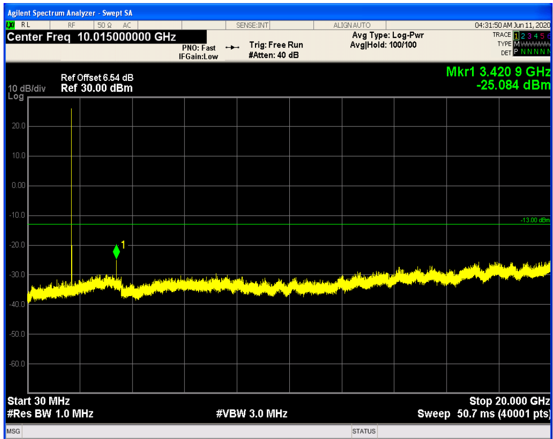
LTE Band66 QAM16 BW=5MHz Channel=131997 RB Size=25 Position=#0
