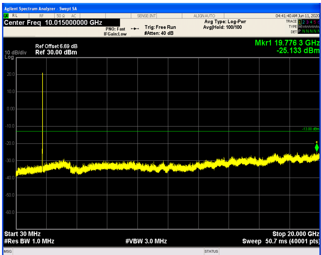
LTE Band66 QPSK BW=15MHz Channel=132047 RB Size=1 Position=#0
