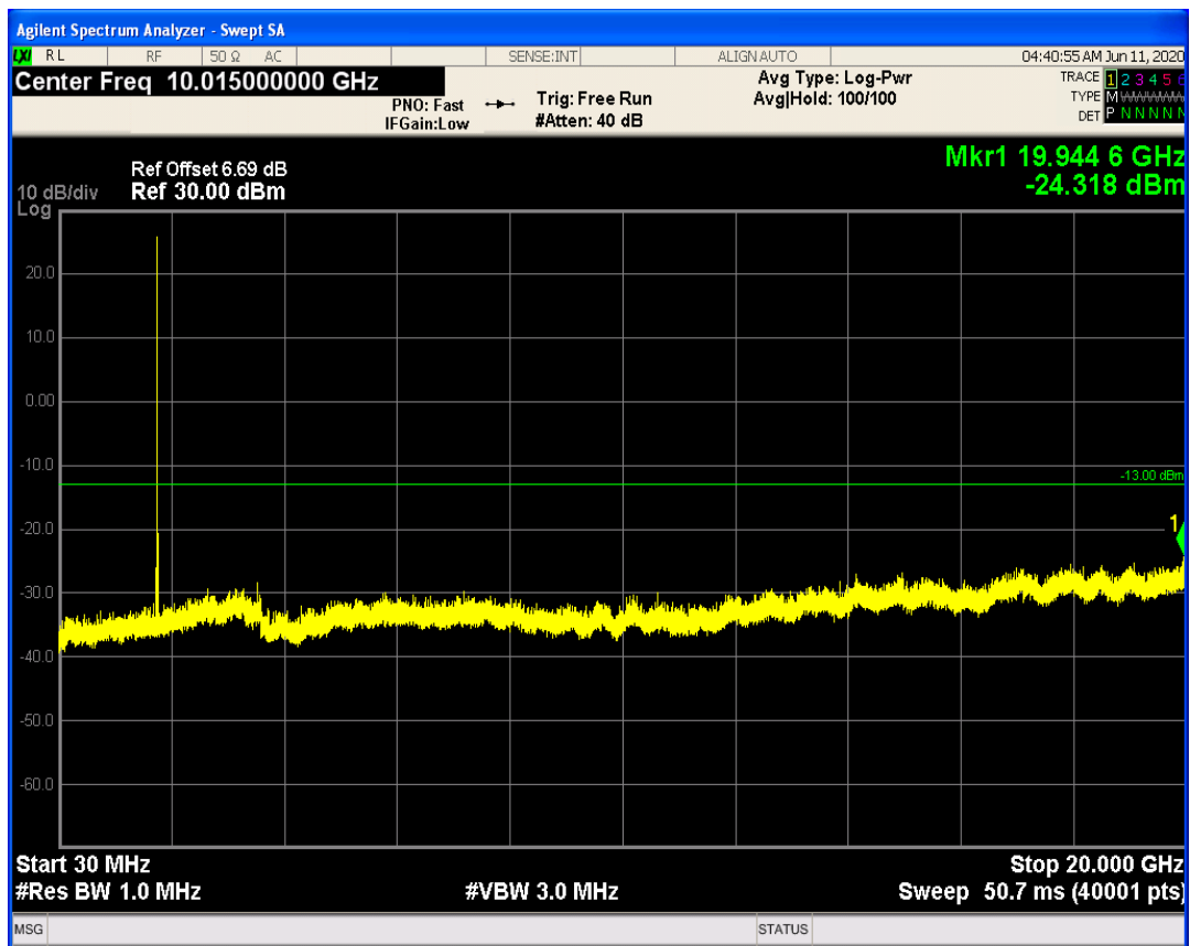
LTE Band66 QAM16 BW=10MHz Channel=132622 RB Size=50 Position=#0
