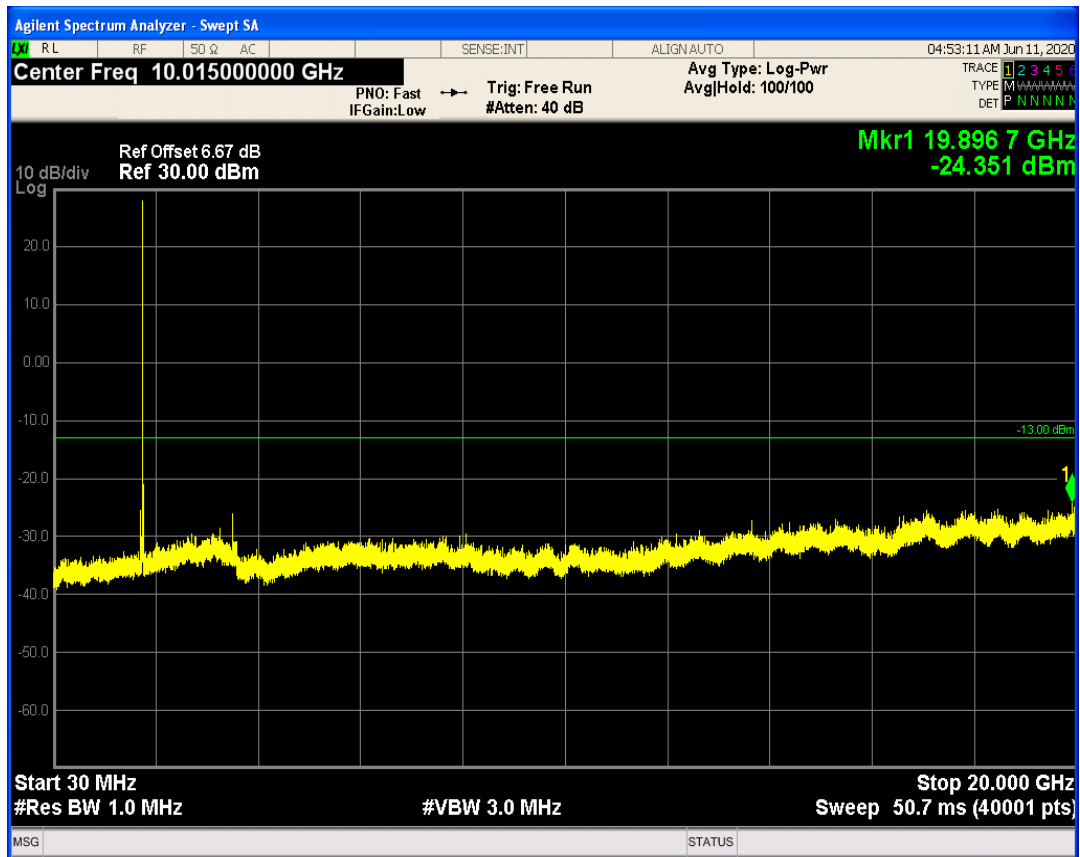
LTE Band66 QAM16 BW=20MHz Channel=132572 RB Size=100 Position=#0
