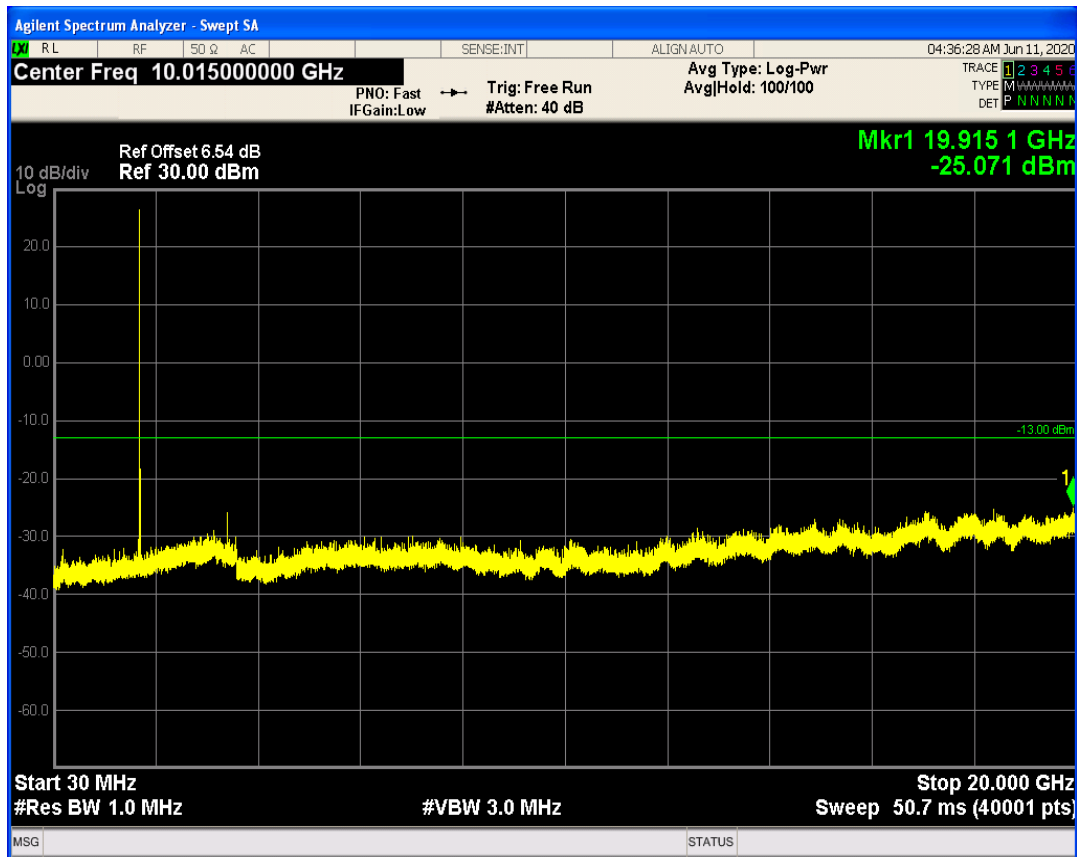
LTE Band66 QPSK BW=10MHz Channel=132022 RB Size=50 Position=#0
