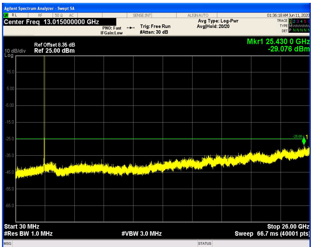
LTE Band7 QPSK BW=20MHz Channel=21350 RB Size=100 Position=#0
