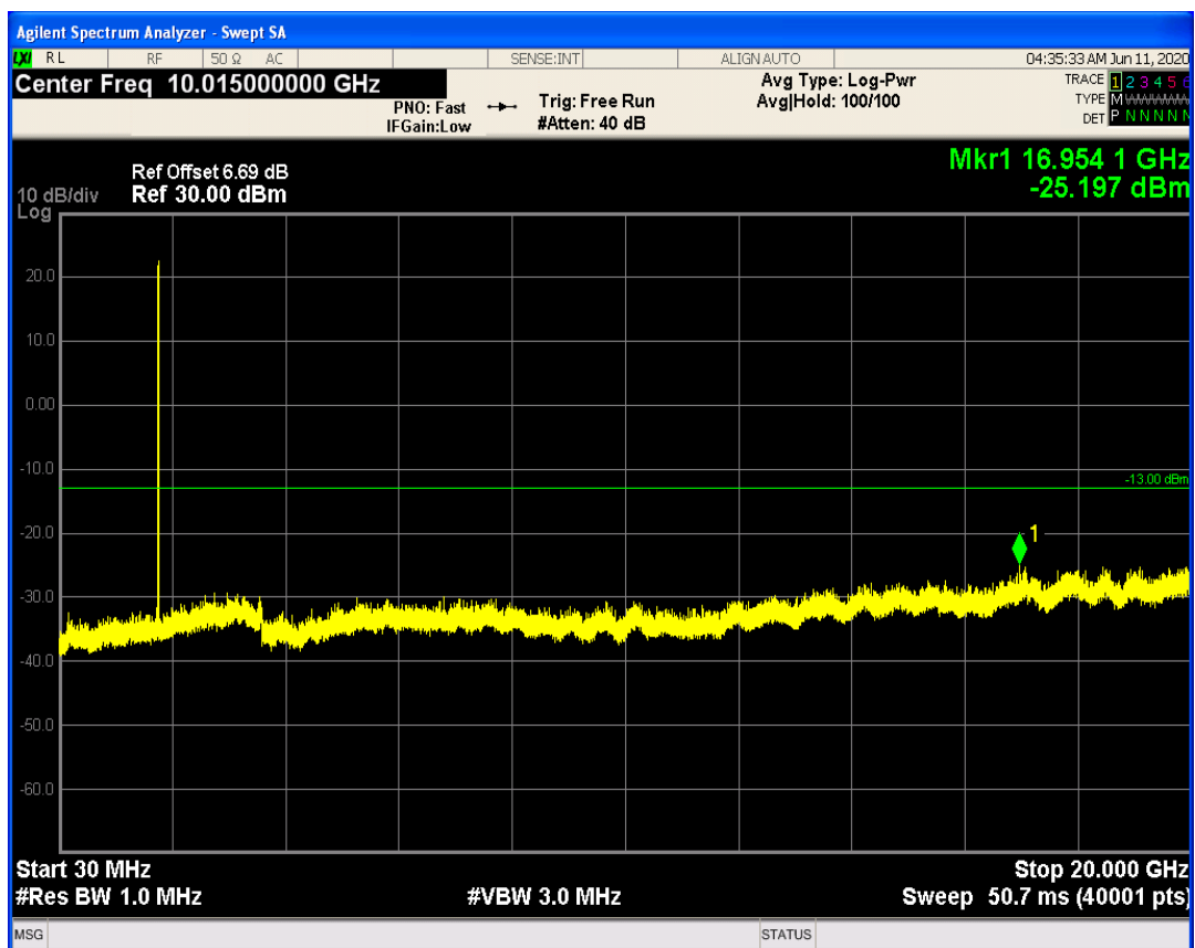
LTE Band66 QPSK BW=10MHz Channel=132022 RB Size=1 Position=#0
