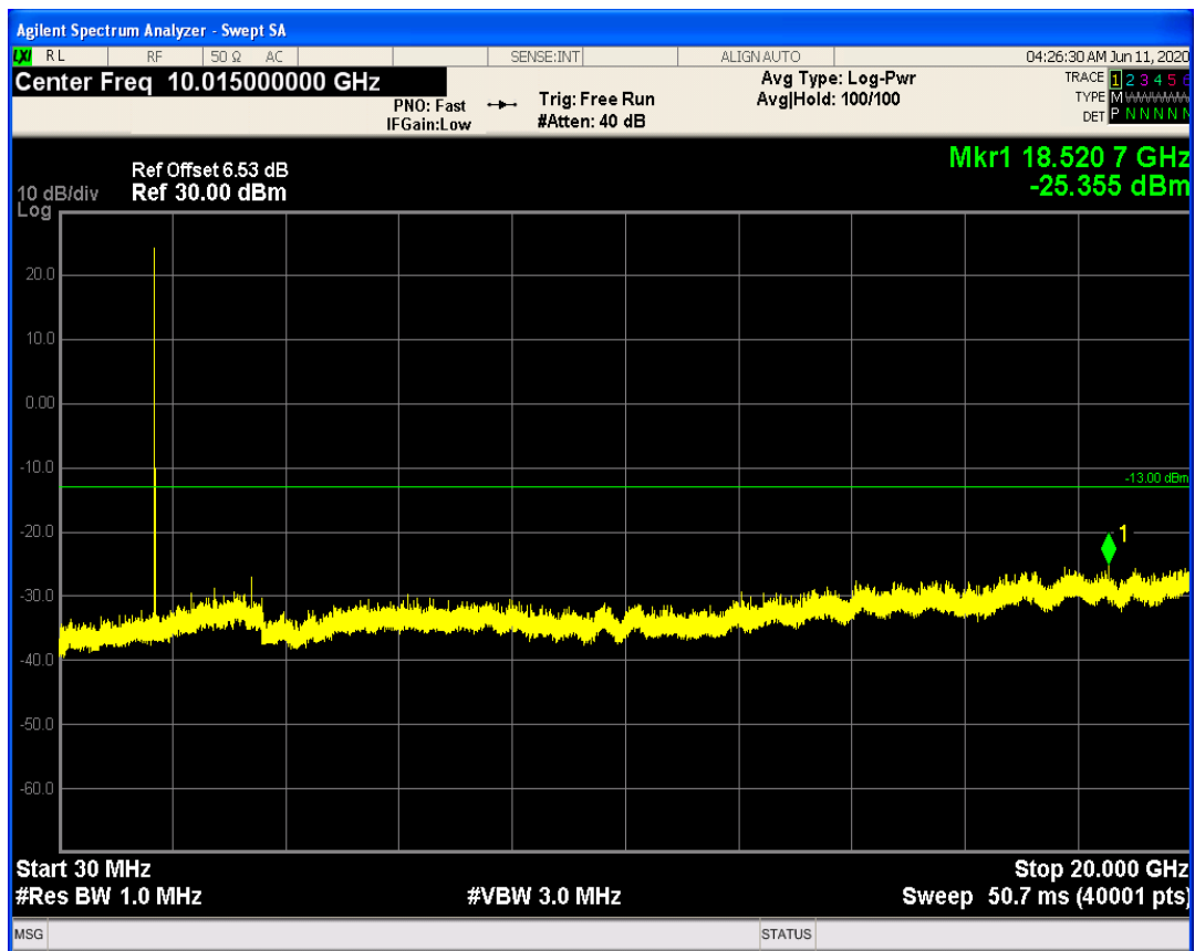
LTE Band66 QAM16 BW=3MHz Channel=131987 RB Size=1 Position=#0
