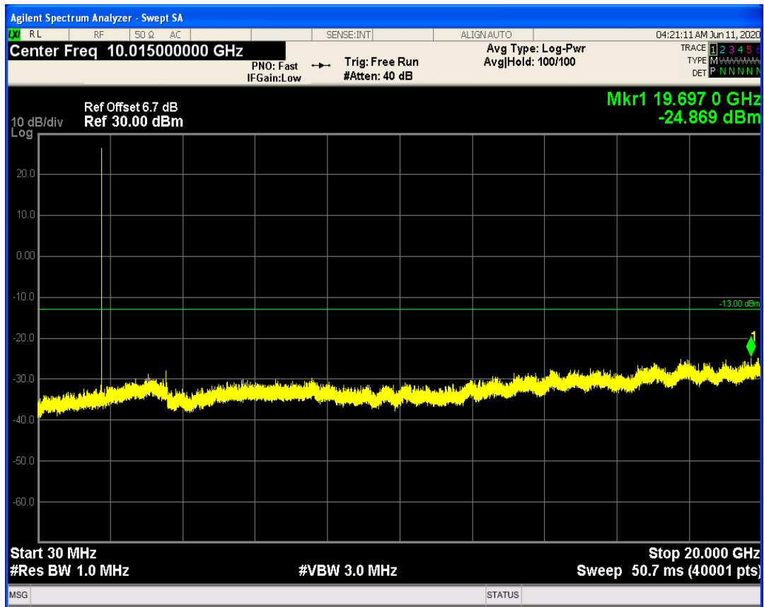
LTE Band66 QPSK BW=1.4MHz Channel=132665 RB Size=6 Position=#0
