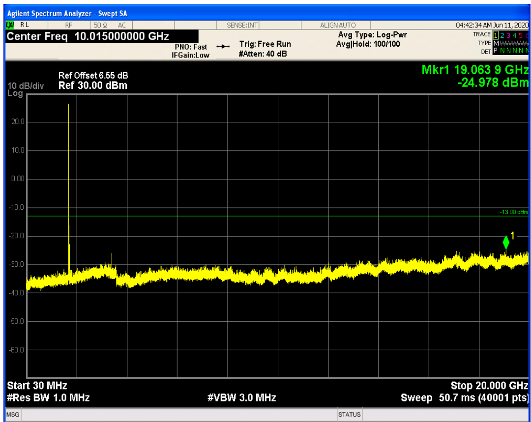
LTE Band66 QPSK BW=15MHz Channel=132047 RB Size=75 Position=#0
