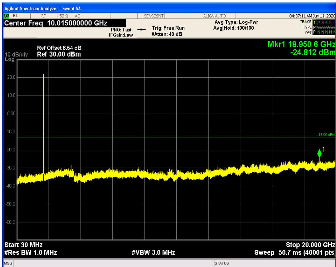
LTE Band66 QAM16 BW=10MHz Channel=132022 RB Size=1 Position=#0
