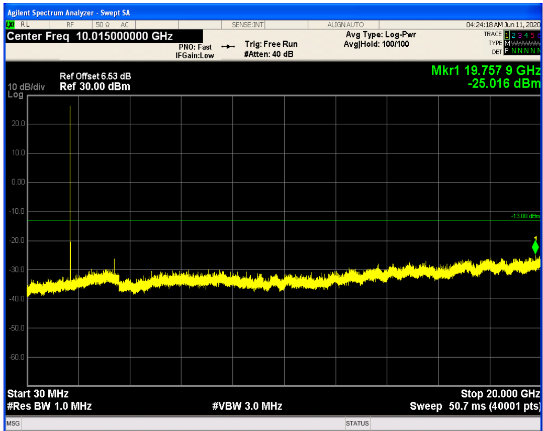
LTE Band66 QPSK BW=3MHz Channel=131987 RB Size=15 Position=#0
