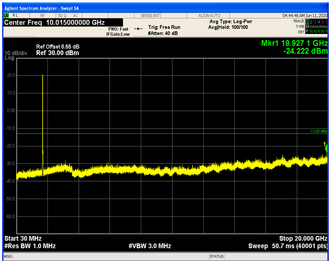
LTE Band66 QPSK BW=15MHz Channel=132597 RB Size=1 Position=#0
