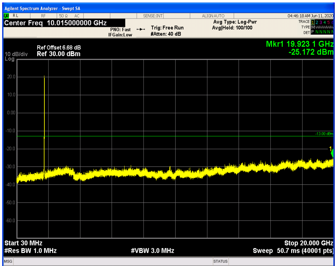
LTE Band66 QAM16 BW=15MHz Channel=132597 RB Size=1 Position=#0
