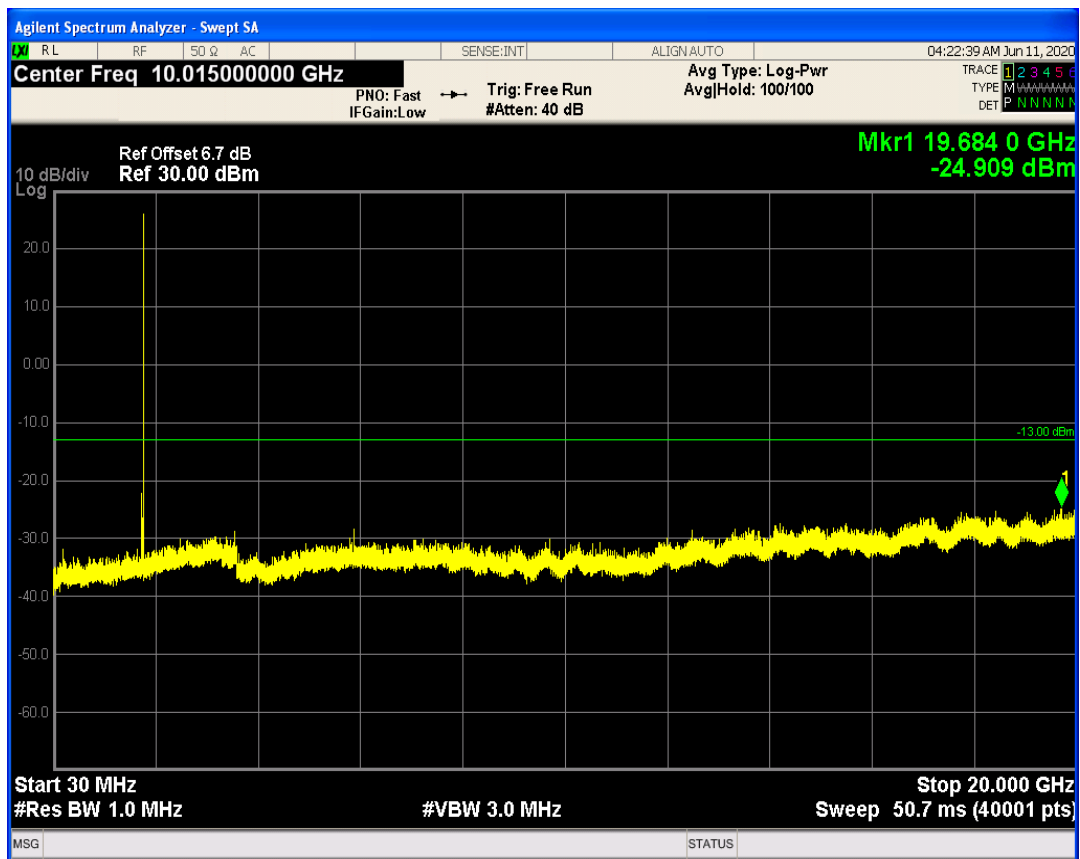
LTE Band66 QAM16 BW=1.4MHz Channel=132665 RB Size=6 Position=#0
