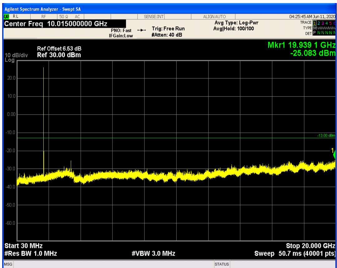
LTE Band66 QPSK BW=3MHz Channel=132657 RB Size=1 Position=#0
