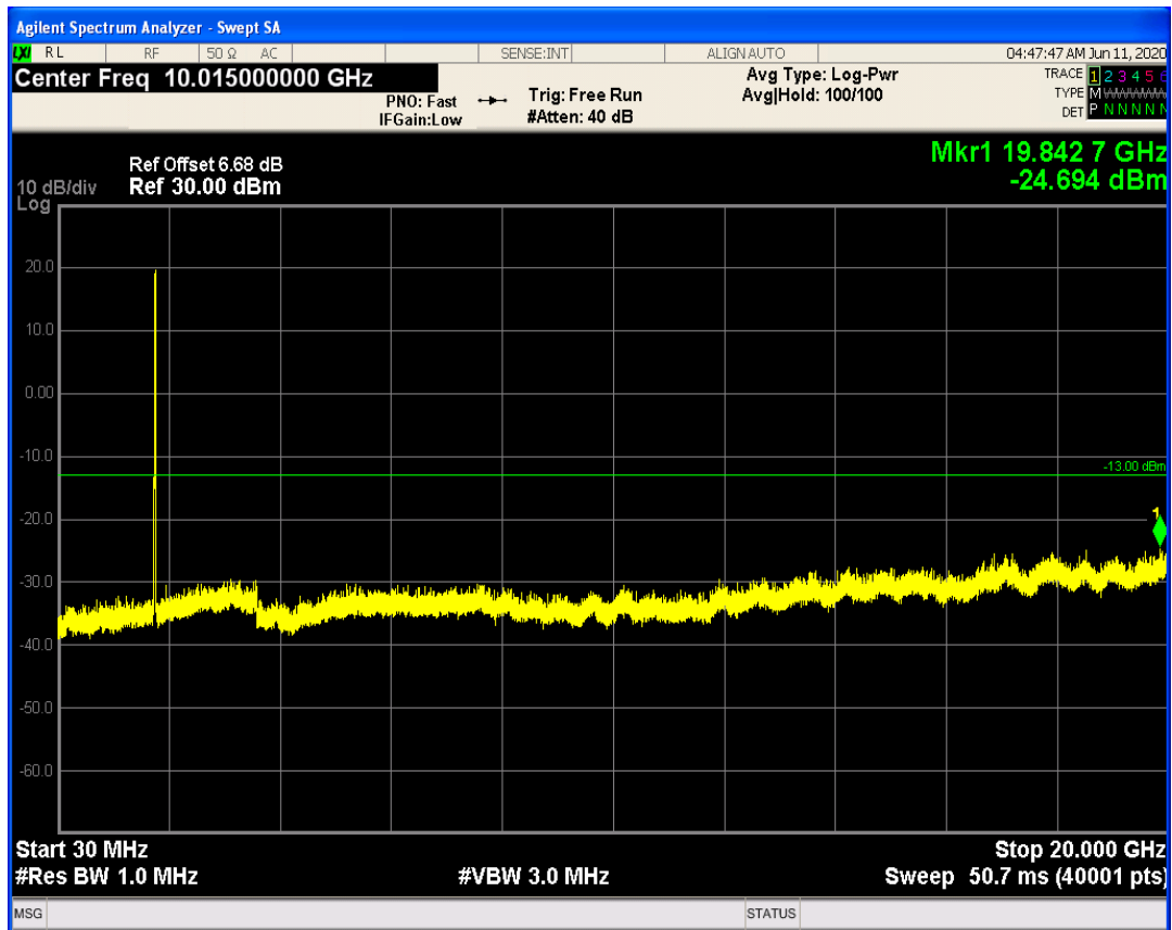
LTE Band66 QPSK BW=20MHz Channel=132072 RB Size=100 Position=#0
