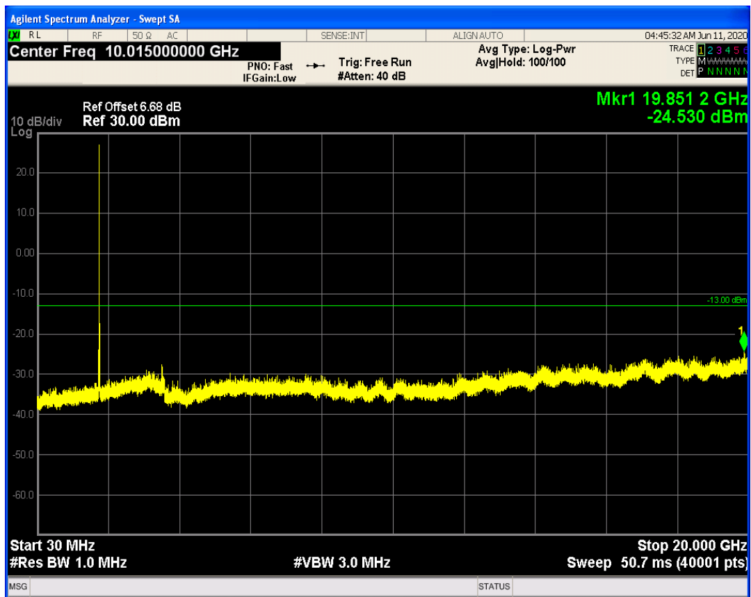
LTE Band66 QPSK BW=15MHz Channel=132597 RB Size=75 Position=#0
