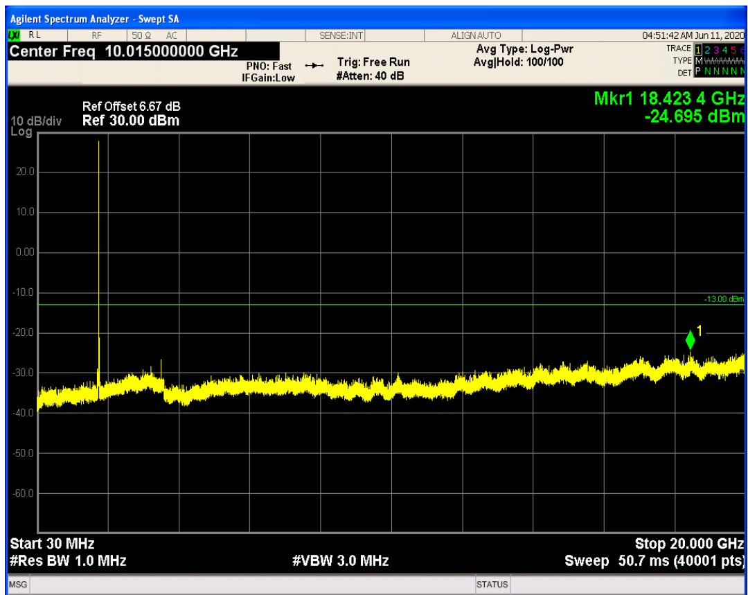
LTE Band66 QPSK BW=20MHz Channel=132572 RB Size=100 Position=#0
