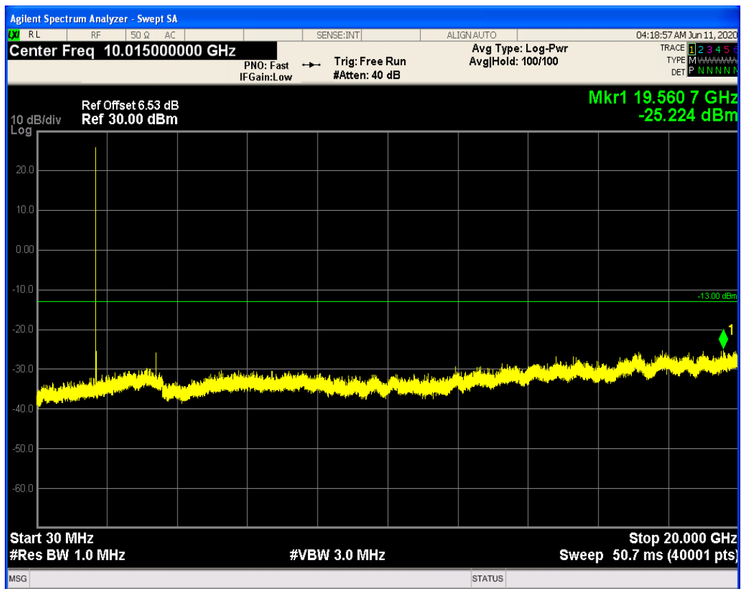
LTE Band66 QAM16 BW=1.4MHz Channel=131979 RB Size=1 Position=#0
