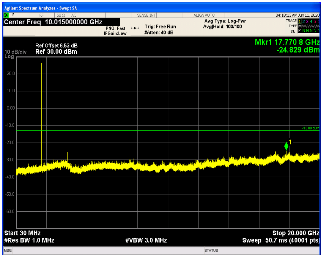
LTE Band66 QPSK BW=1.4MHz Channel=131979 RB Size=6 Position=#0
