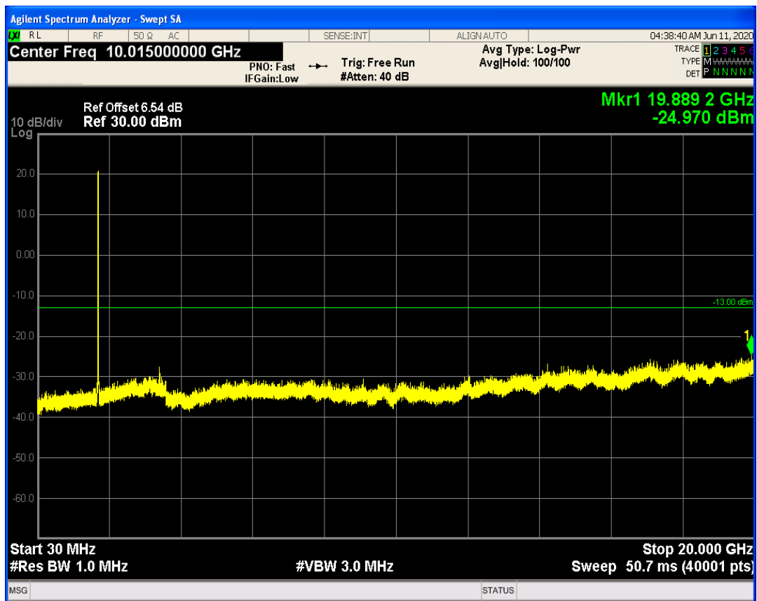
LTE Band66 QPSK BW=10MHz Channel=132622 RB Size=50 Position=#0
