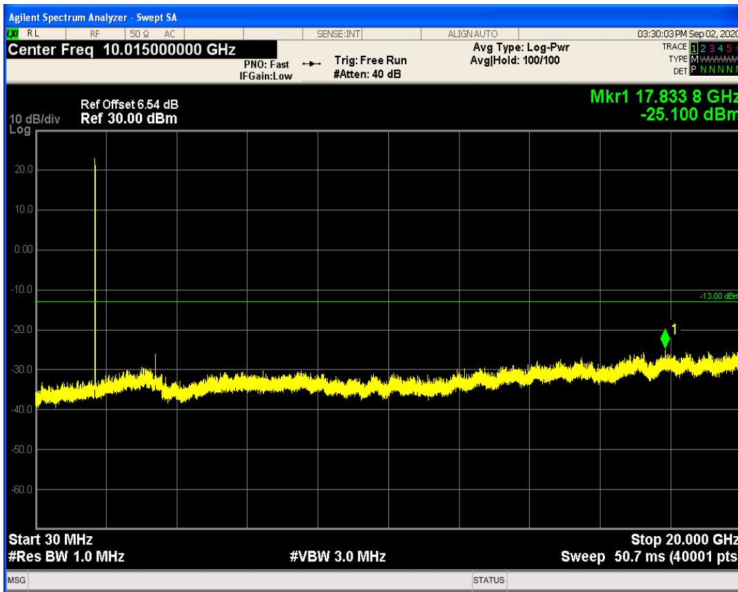
LTE Band66 QAM16 BW=5MHz Channel=131997 RB Size=1 Position=#0
