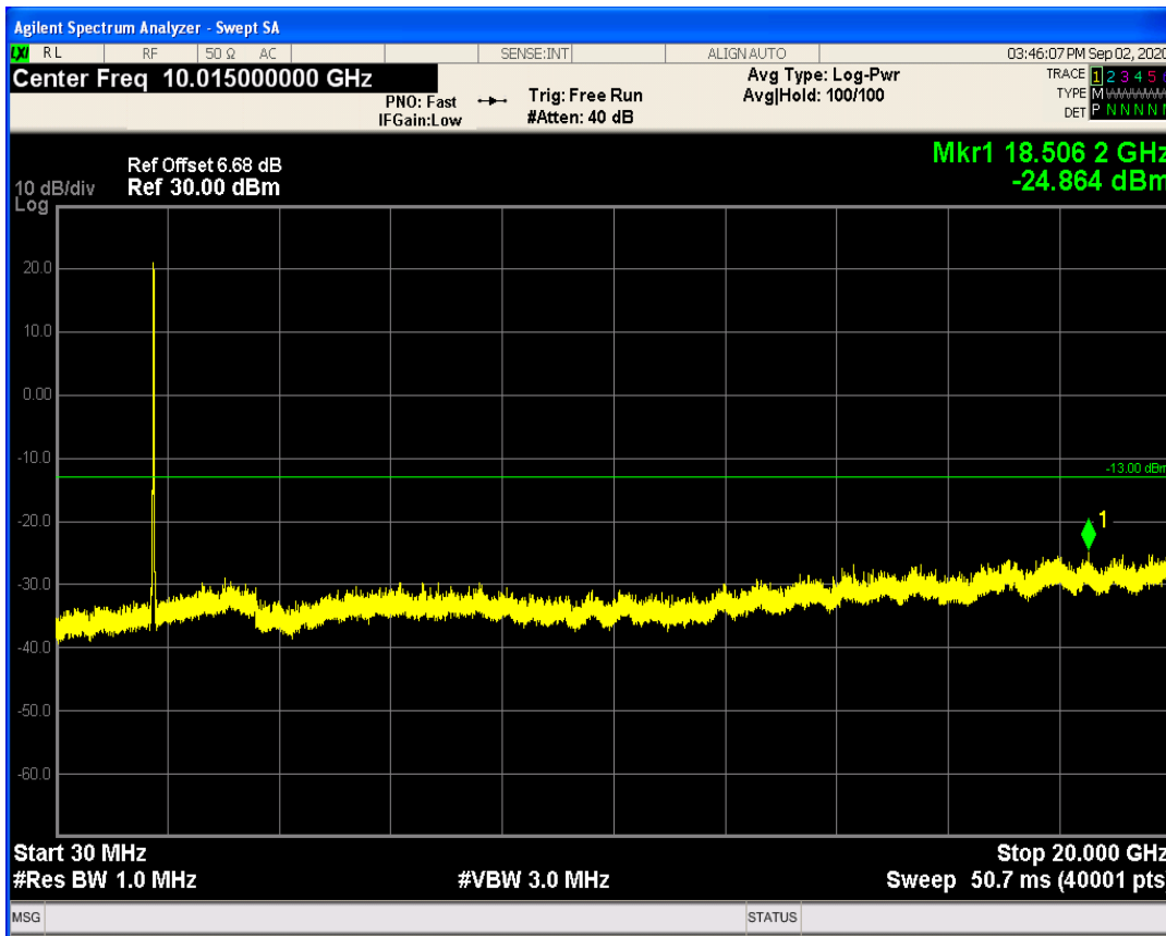
LTE Band66 QAM16 BW=15MHz Channel=132597 RB Size=1 Position=#0
