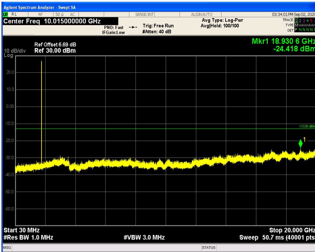
LTE Band66 QPSK BW=10MHz Channel=132022 RB Size=1 Position=#0
