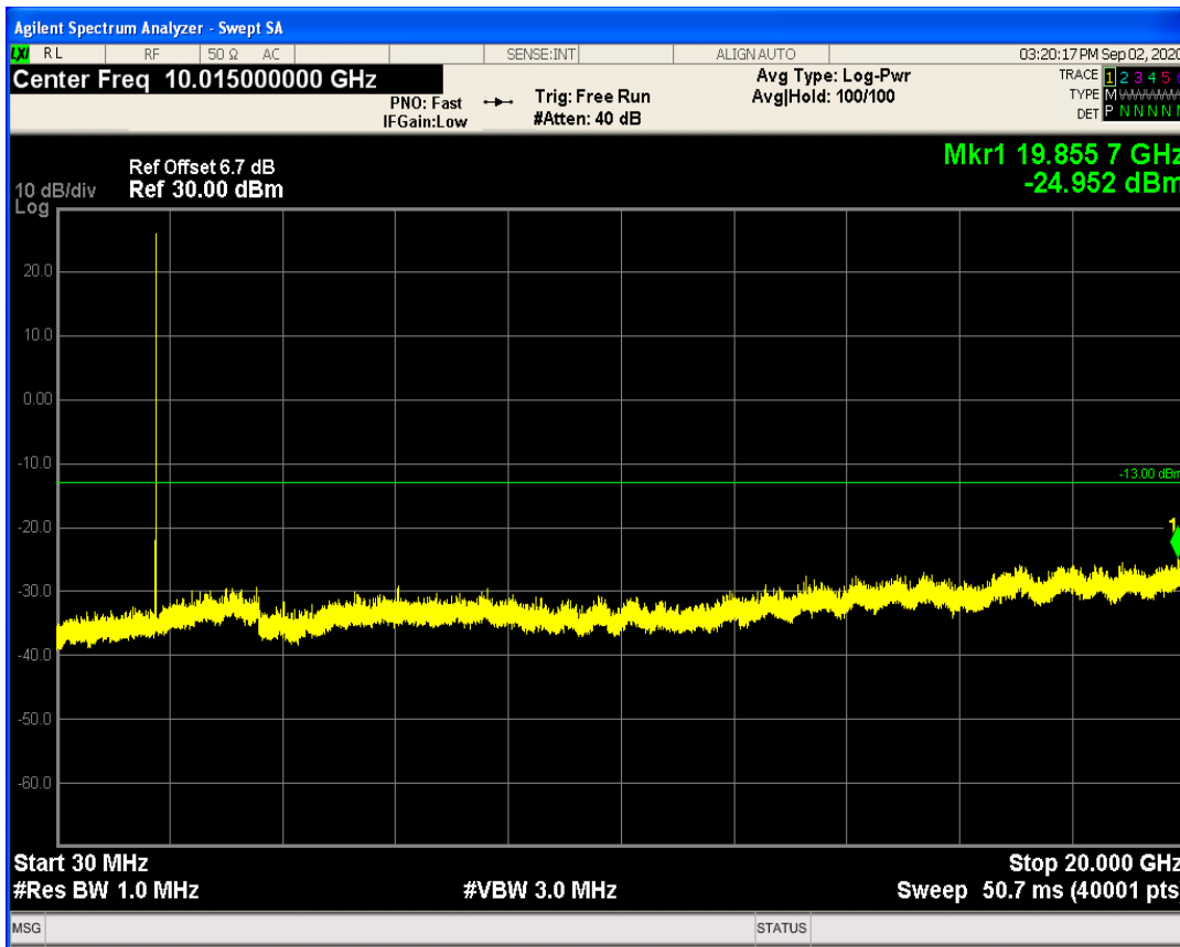
LTE Band66 QAM16 BW=1.4MHz Channel=132665 RB Size=1 Position=#0
