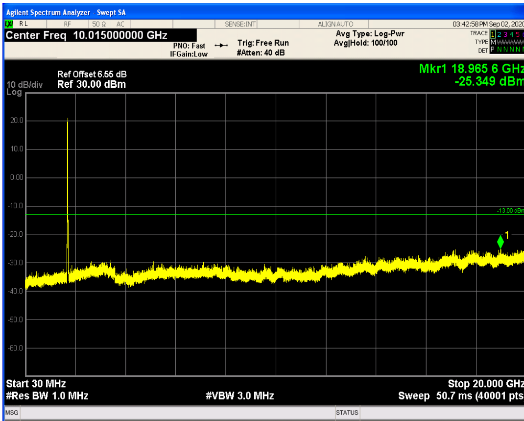
LTE Band66 QAM16 BW=15MHz Channel=132047 RB Size=1 Position=#0
