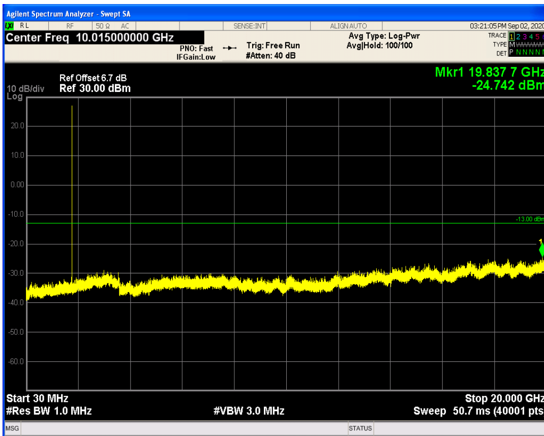
LTE Band66 QPSK BW=3MHz Channel=131987 RB Size=1 Position=#0
