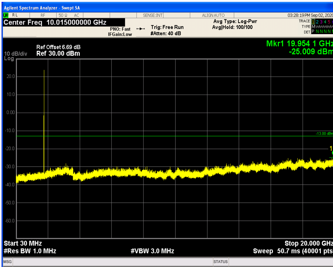
LTE Band66 QPSK BW=5MHz Channel=131997 RB Size=1 Position=#0
