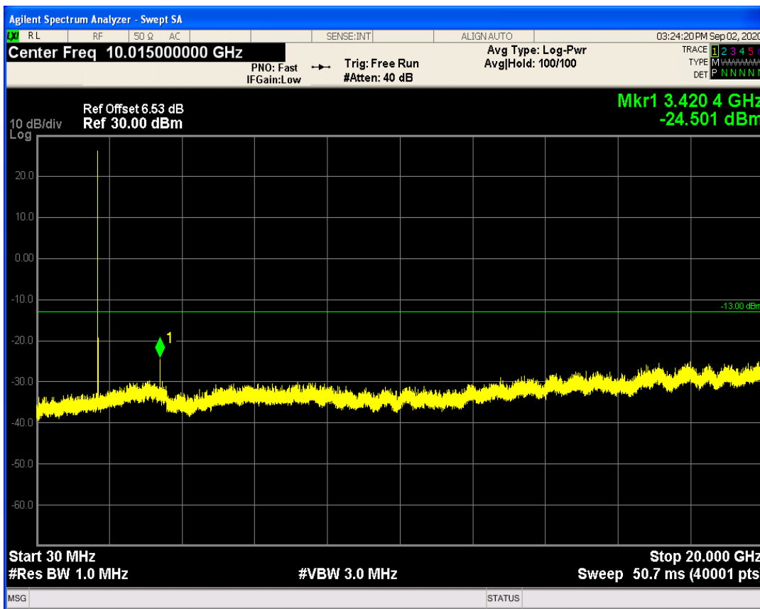
LTE Band66 QPSK BW=3MHz Channel=132657 RB Size=1 Position=#0
