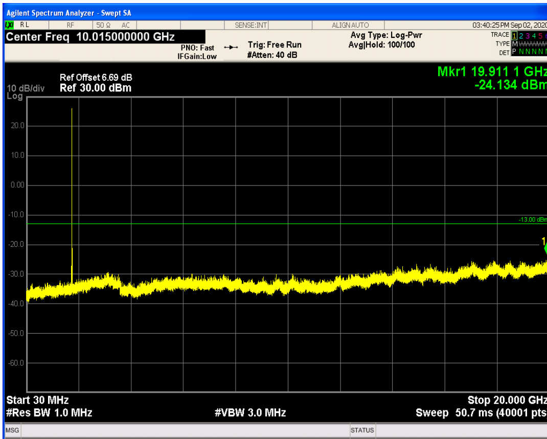
LTE Band66 QPSK BW=15MHz Channel=132047 RB Size=1 Position=#0
