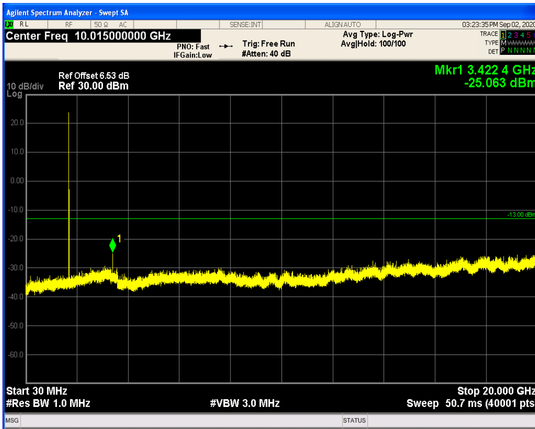
LTE Band66 QAM16 BW=3MHz Channel=131987 RB Size=1 Position=#0
