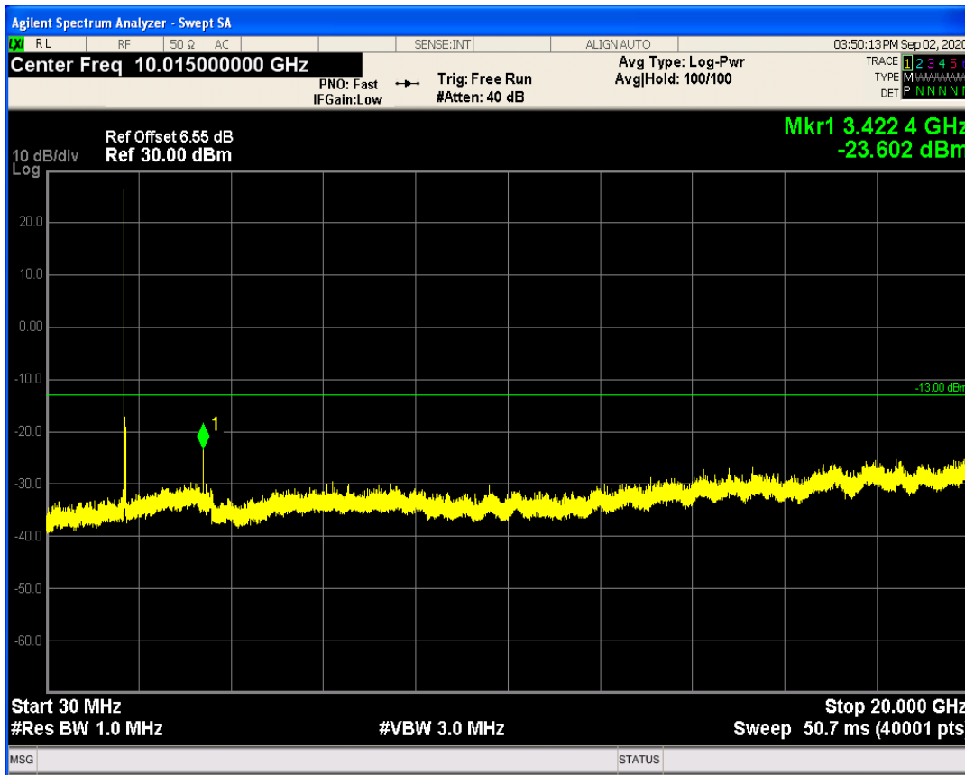
LTE Band66 QPSK BW=20MHz Channel=132572 RB Size=1 Position=#0
