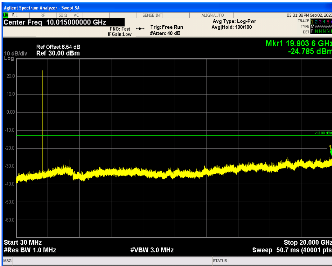
LTE Band66 QPSK BW=5MHz Channel=132647 RB Size=1 Position=#0
