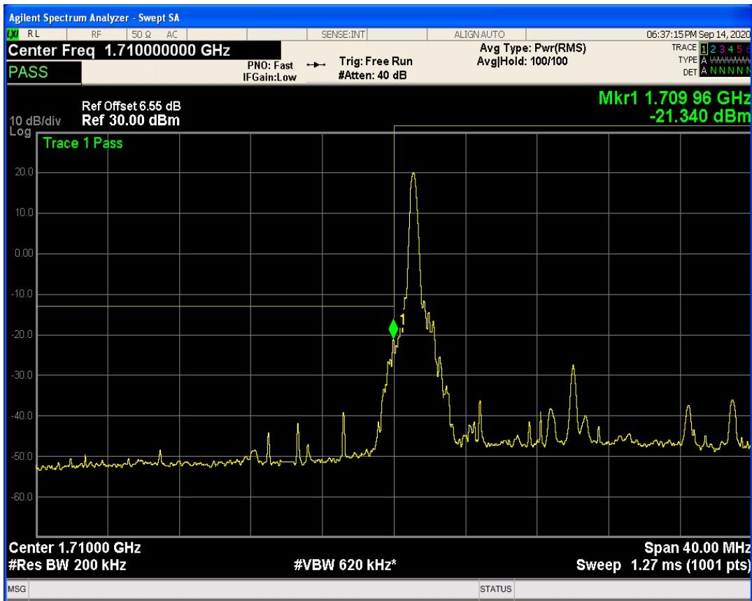
LTE Band66 QPSK BW=20MHz Channel=132072 RB Size=100 Position=#0
