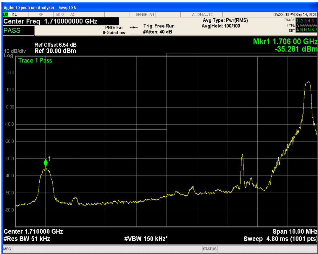
LTE Band66 QAM16 BW=5MHz Channel=131997 RB Size=25 Position=#0
