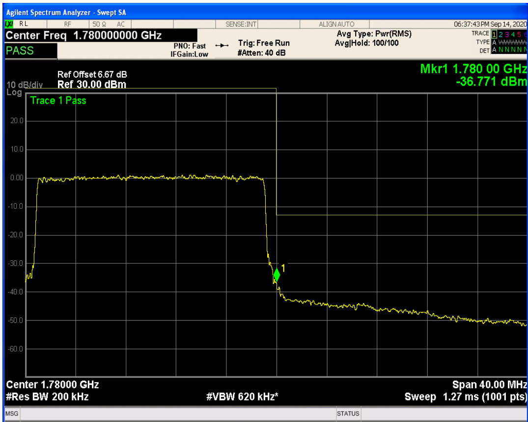
LTE Band66 QAM16 BW=20MHz Channel=132572 RB Size=1 Position=#0
