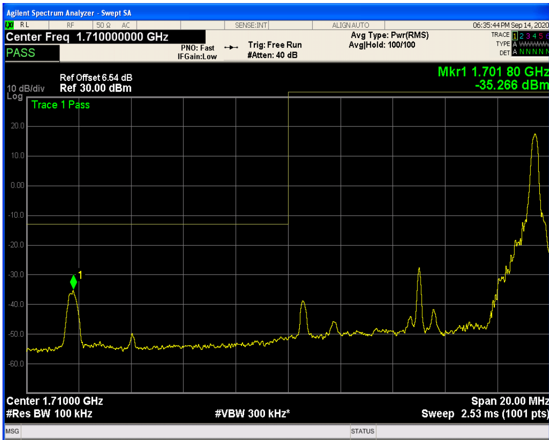
LTE Band66 QAM16 BW=10MHz Channel=132022 RB Size=50 Position=#0
