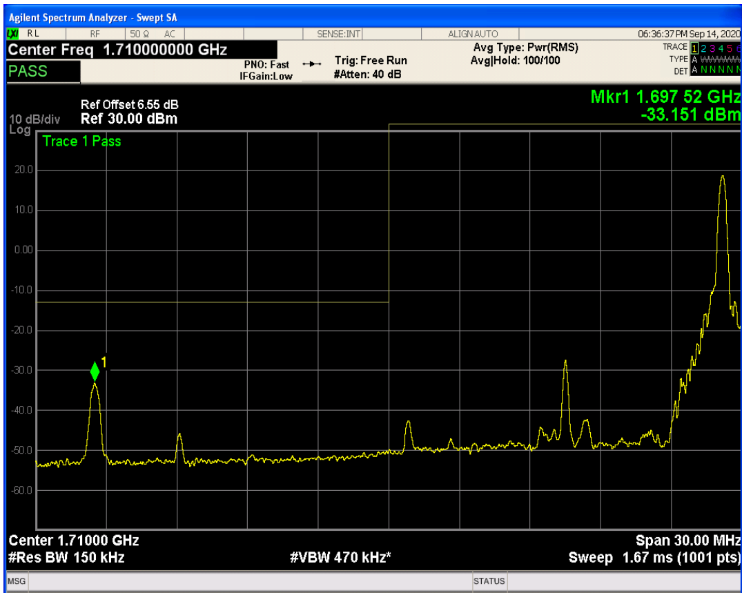
LTE Band66 QAM16 BW=15MHz Channel=132047 RB Size=75 Position=#0
