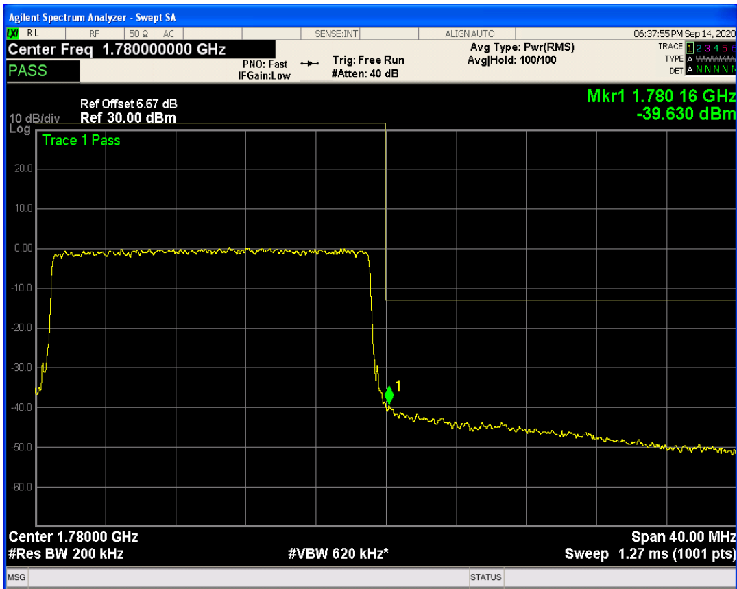
LTE Band66 QAM16 BW=20MHz Channel=132572 RB Size=1 Position=#Max
