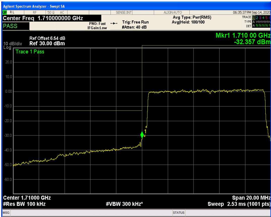
LTE Band66 QAM16 BW=10MHz Channel=132022 RB Size=1 Position=#0
