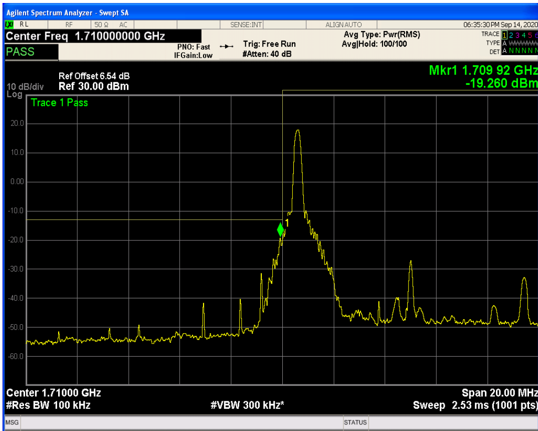
LTE Band66 QPSK BW=10MHz Channel=132022 RB Size=1 Position=#Max
