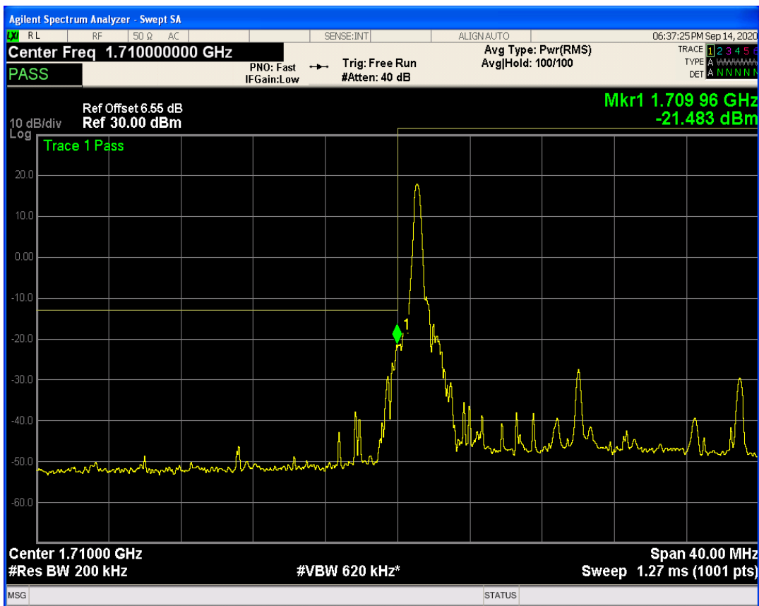
LTE Band66 QAM16 BW=20MHz Channel=132072 RB Size=1 Position=#Max
