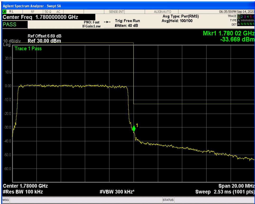
LTE Band66 QAM16 BW=10MHz Channel=132622 RB Size=1 Position=#0
