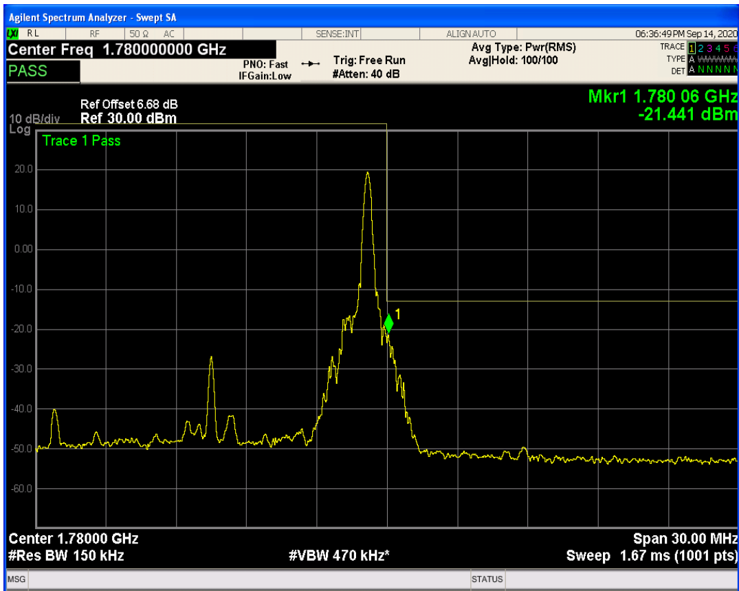
LTE Band66 QPSK BW=15MHz Channel=132597 RB Size=1 Position=#0
