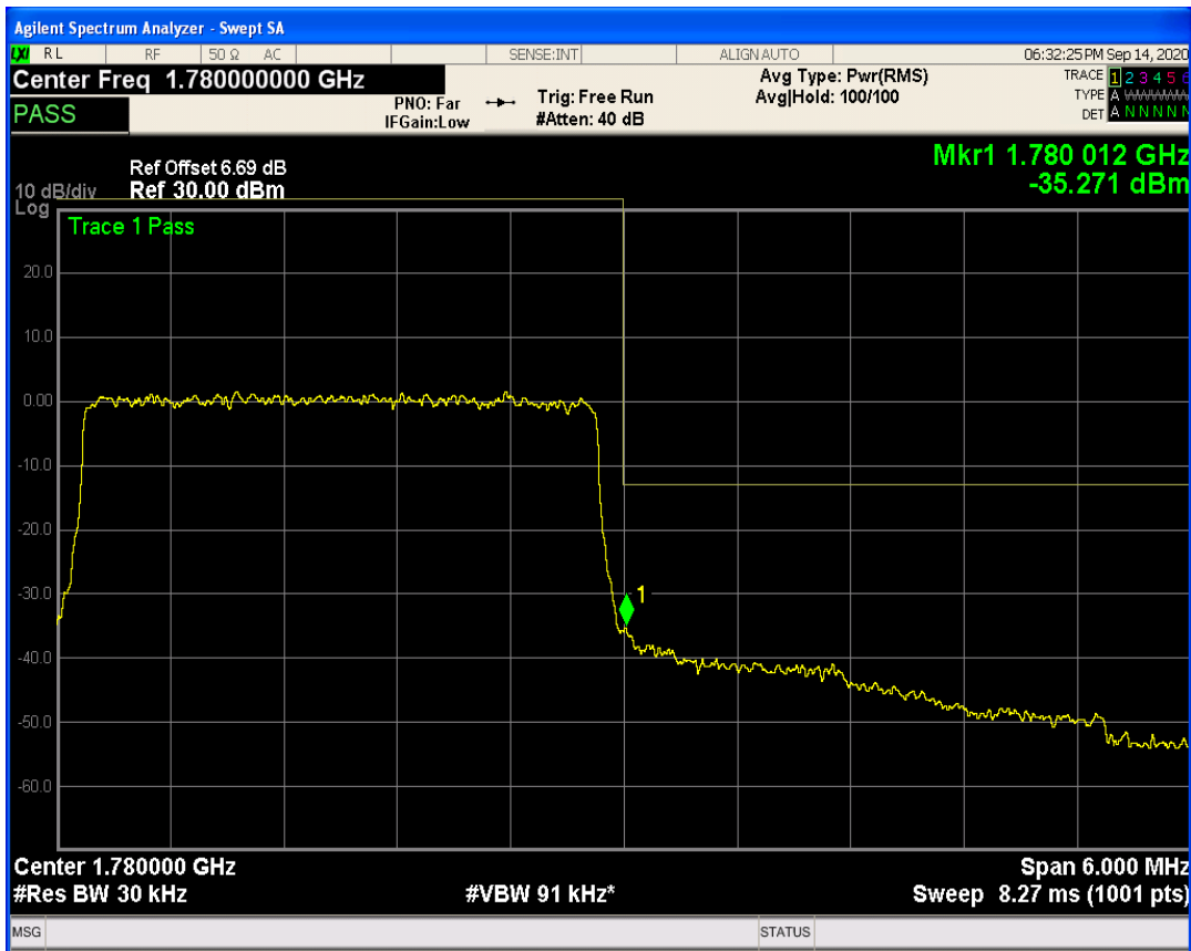
LTE Band66 QAM16 BW=3MHz Channel=132657 RB Size=1 Position=#0
