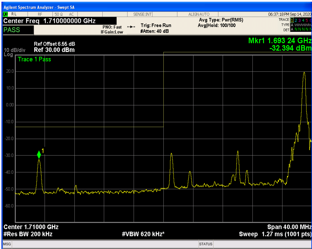
LTE Band66 QAM16 BW=20MHz Channel=132072 RB Size=1 Position=#0
