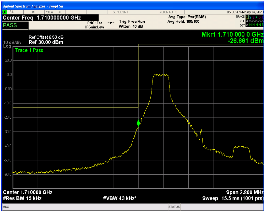
LTE Band66 QPSK BW=1.4MHz Channel=131979 RB Size=1 Position=#Max
