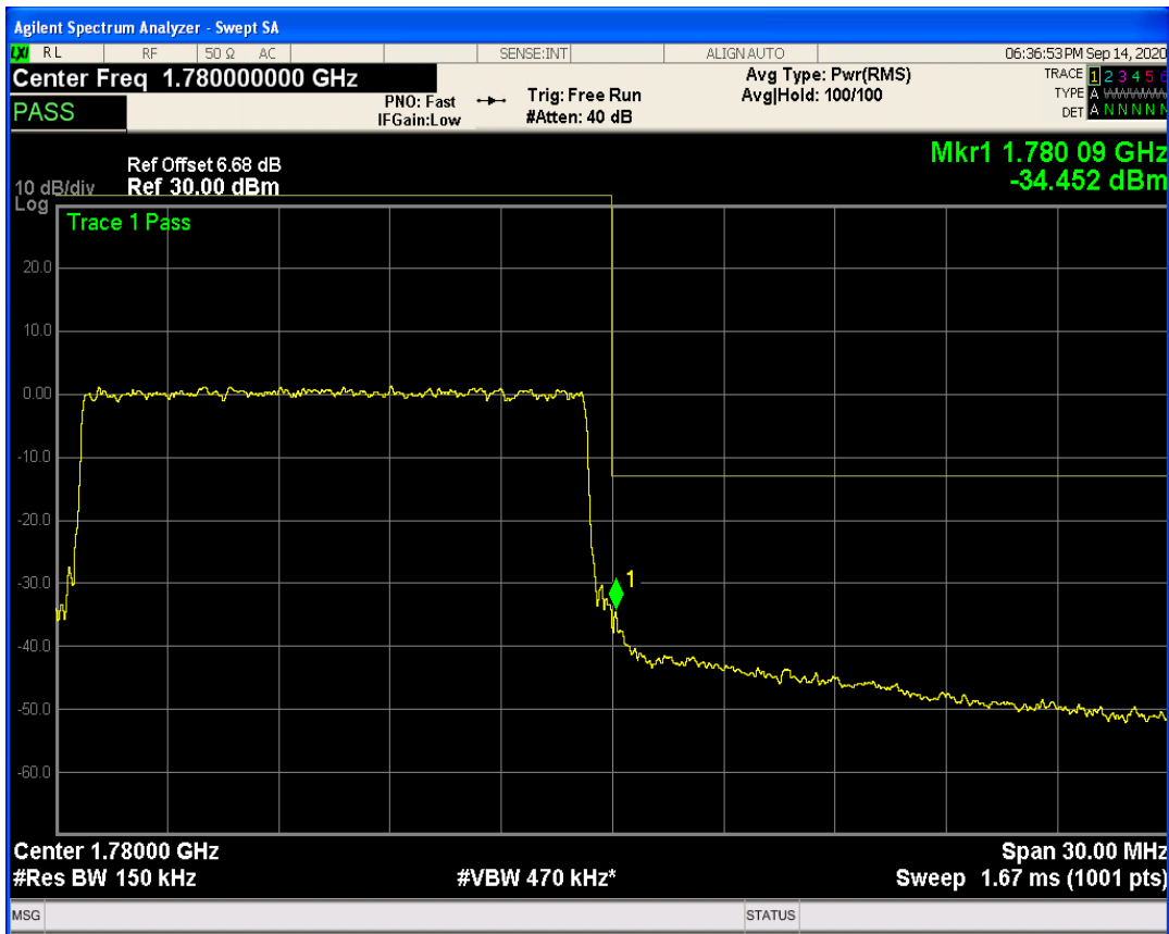
LTE Band66 QAM16 BW=15MHz Channel=132597 RB Size=1 Position=#Max
