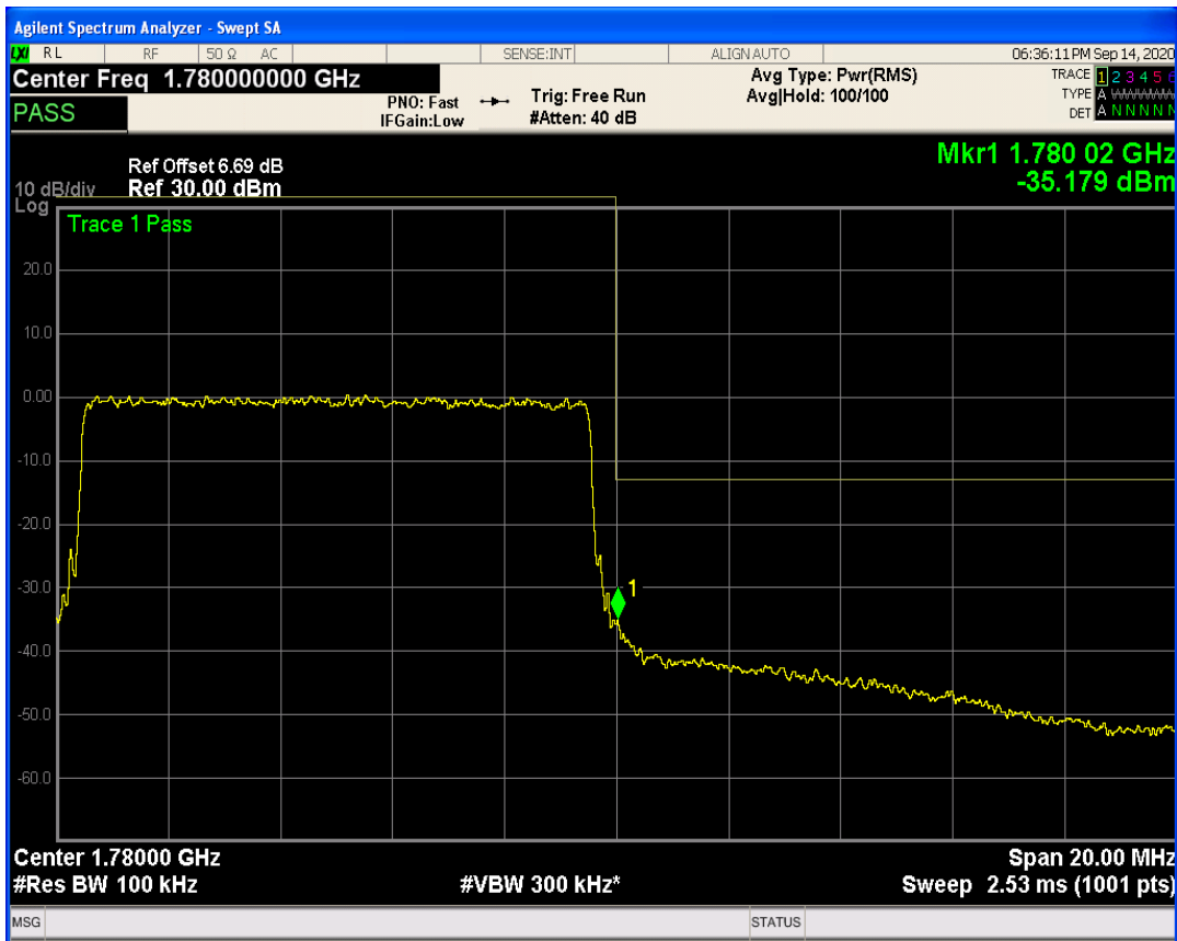
LTE Band66 QAM16 BW=10MHz Channel=132622 RB Size=1 Position=#Max
