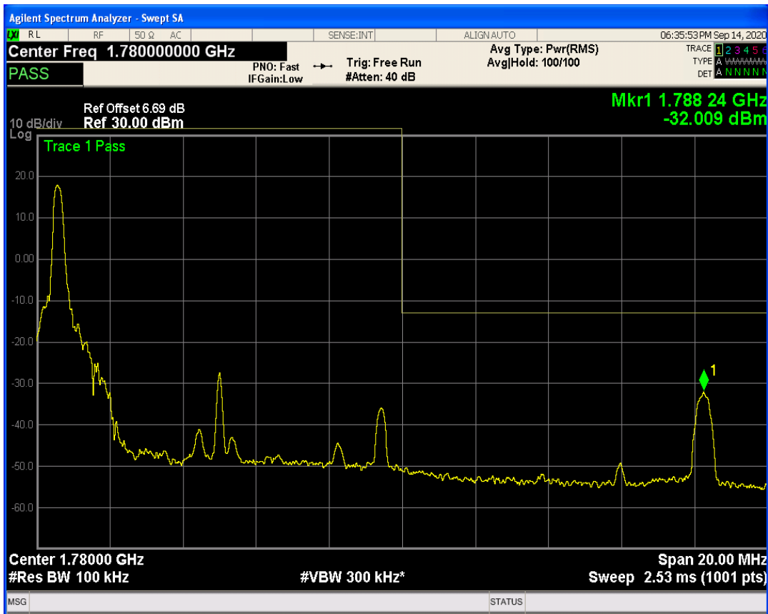
LTE Band66 QPSK BW=10MHz Channel=132622 RB Size=1 Position=#Max
