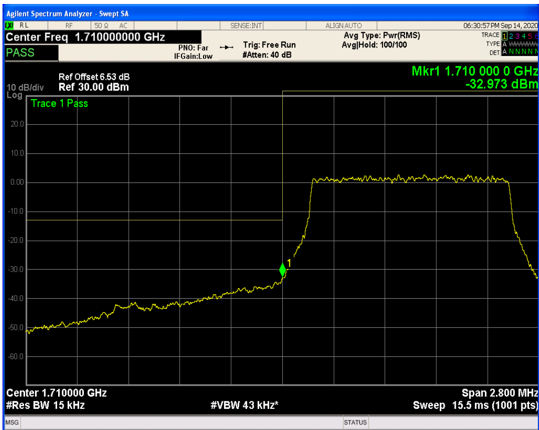
LTE Band66 QAM16 BW=1.4MHz Channel=131979 RB Size=1 Position=#Max
