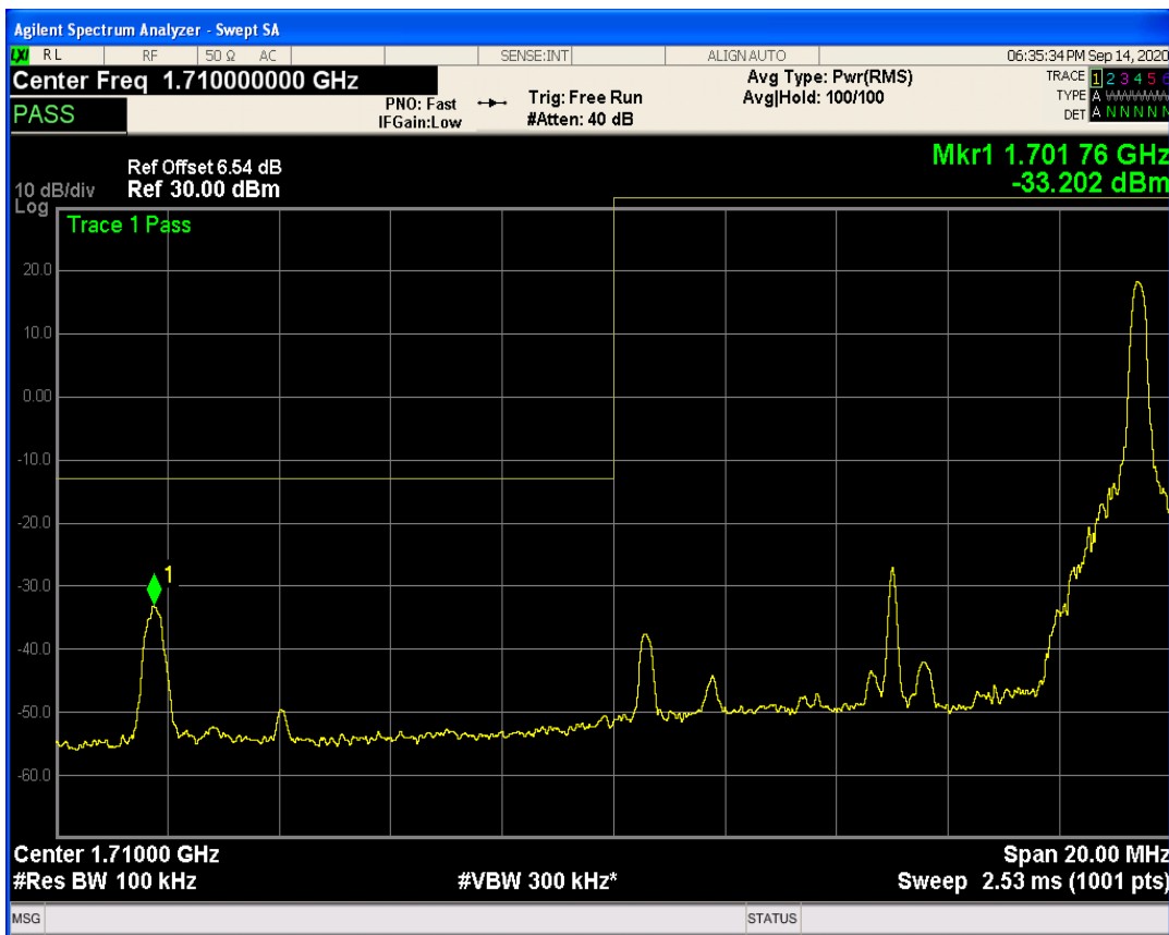
LTE Band66 QPSK BW=10MHz Channel=132022 RB Size=50 Position=#0
