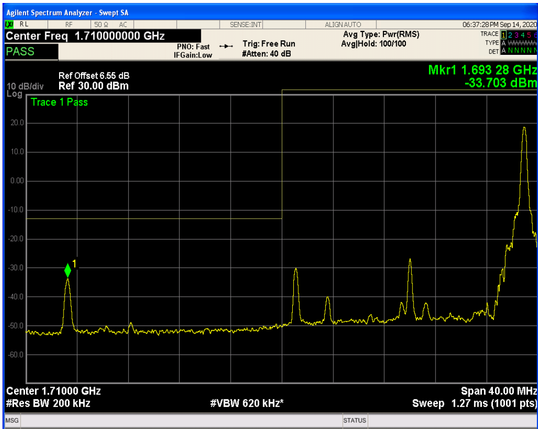
LTE Band66 QAM16 BW=20MHz Channel=132072 RB Size=100 Position=#0
