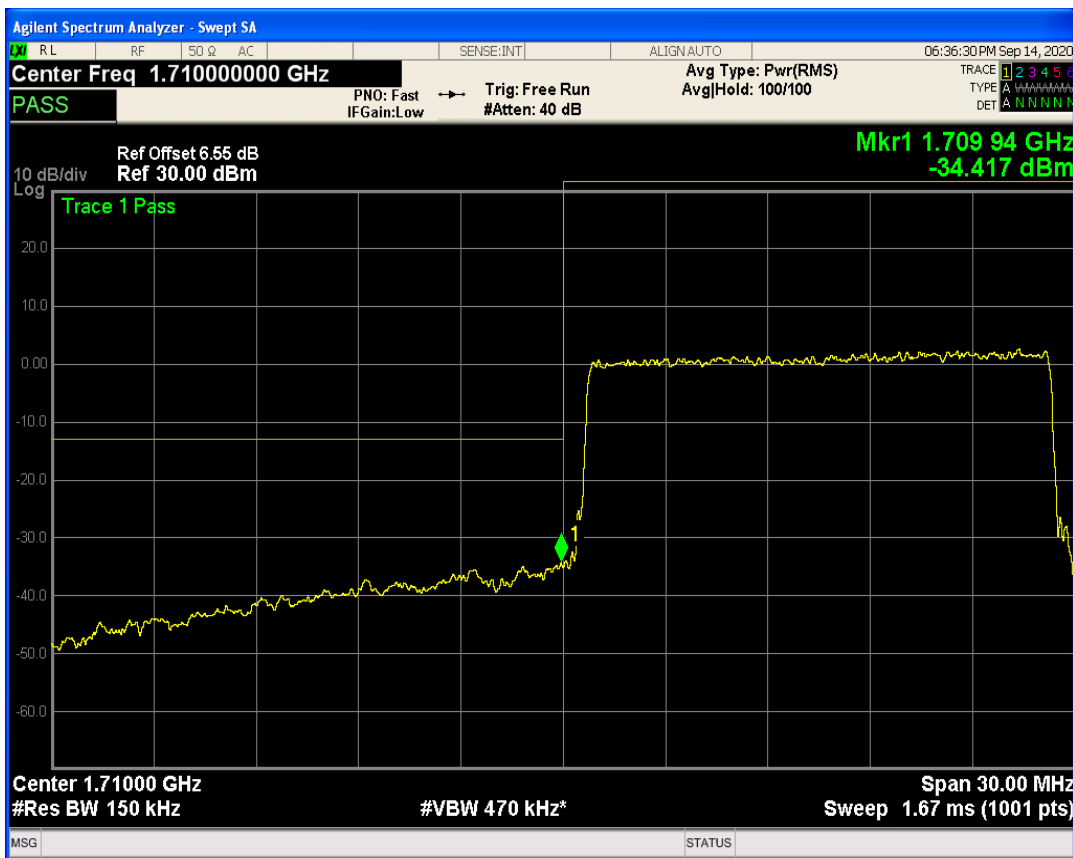
LTE Band66 QAM16 BW=15MHz Channel=132047 RB Size=1 Position=#Max
