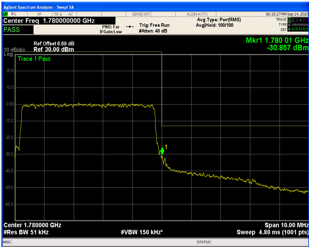
LTE Band66 QAM16 BW=5MHz Channel=132647 RB Size=1 Position=#Max
