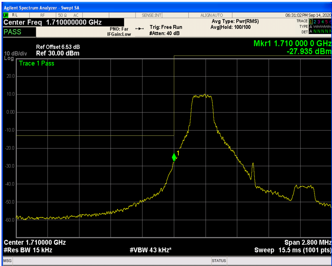
LTE Band66 QPSK BW=1.4MHz Channel=131979 RB Size=6 Position=#0
