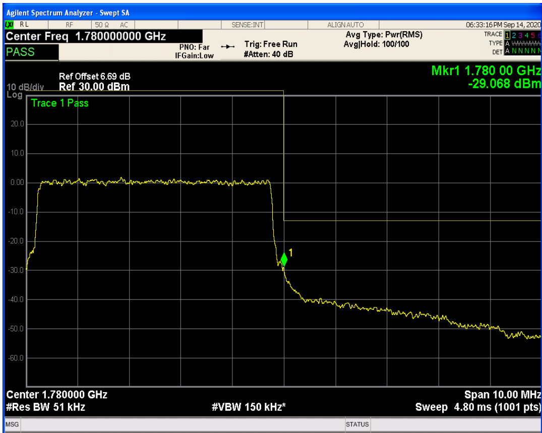
LTE Band66 QAM16 BW=5MHz Channel=132647 RB Size=1 Position=#0
