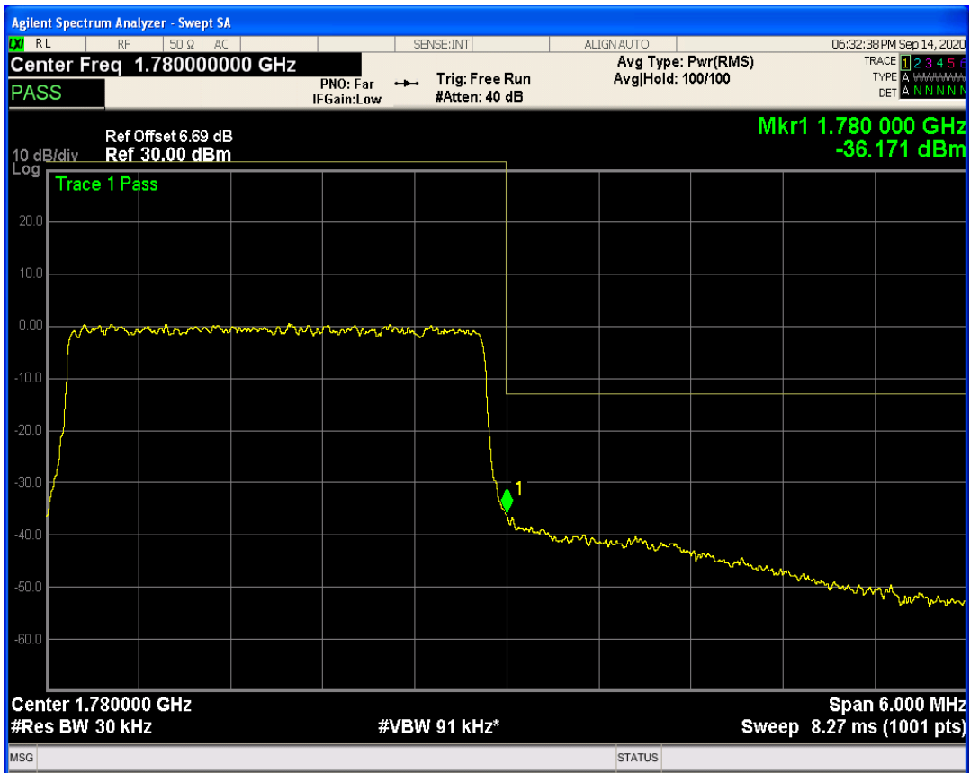
LTE Band66 QAM16 BW=3MHz Channel=132657 RB Size=1 Position=#Max
