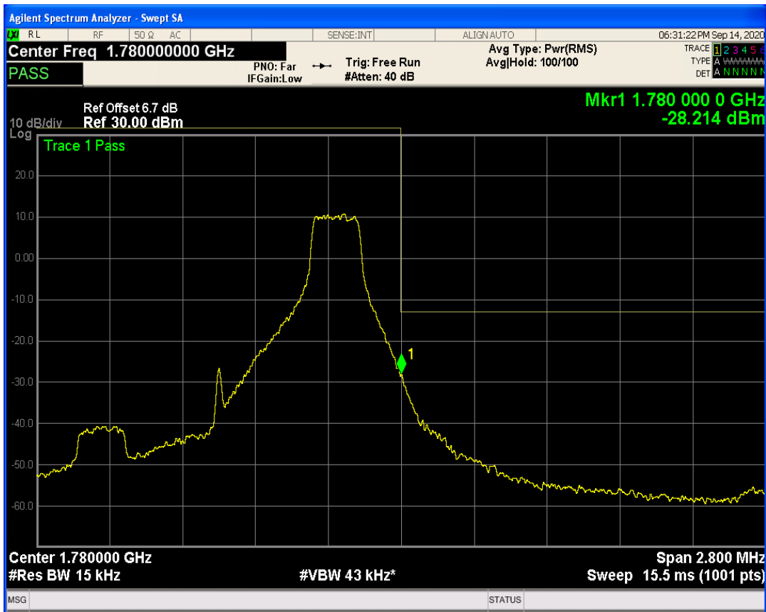
LTE Band66 QPSK BW=1.4MHz Channel=132665 RB Size=1 Position=#0
