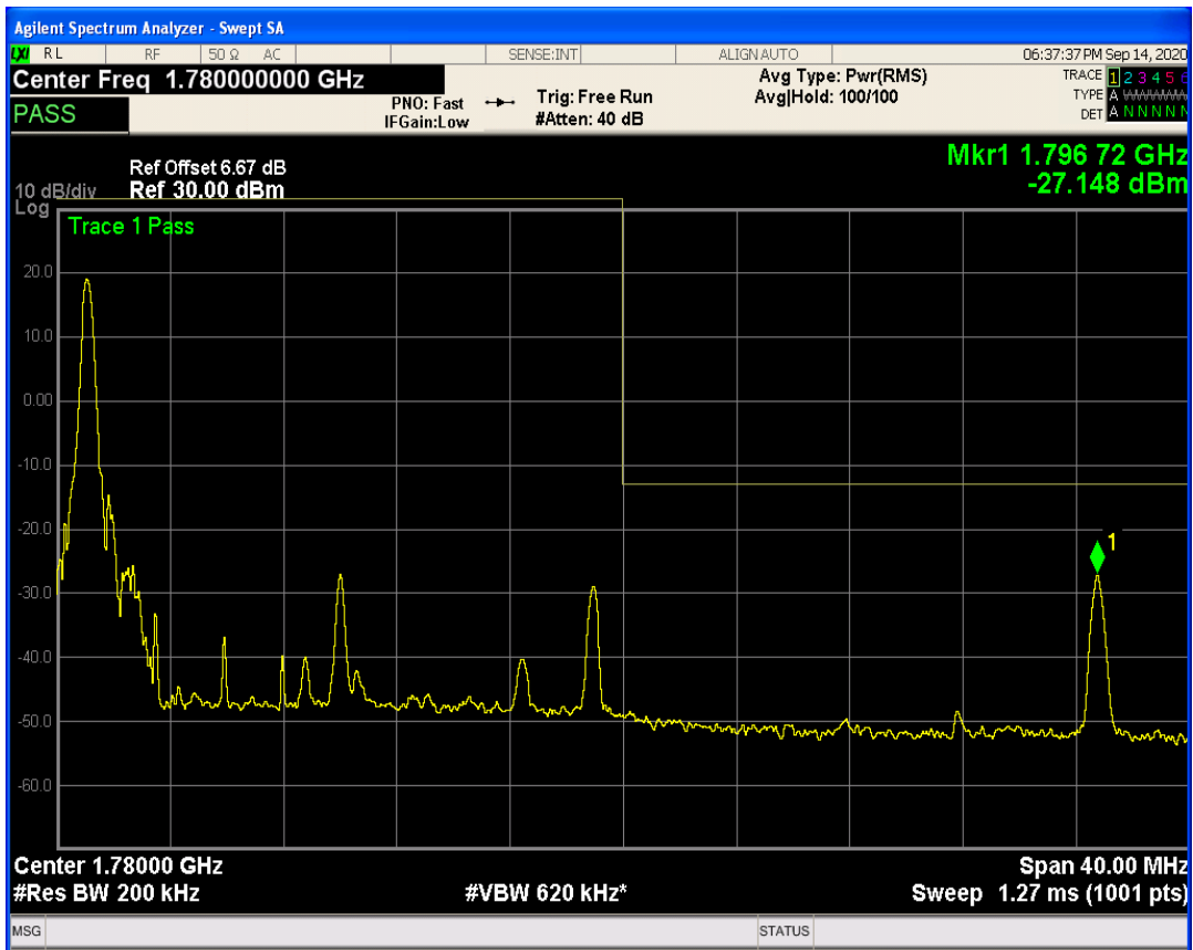
LTE Band66 QPSK BW=20MHz Channel=132572 RB Size=1 Position=#Max
