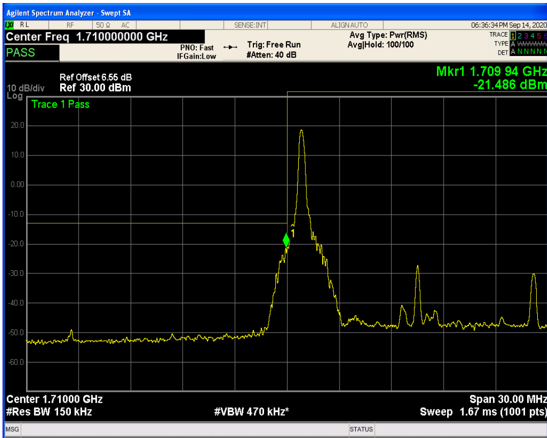
LTE Band66 QPSK BW=15MHz Channel=132047 RB Size=75 Position=#0
