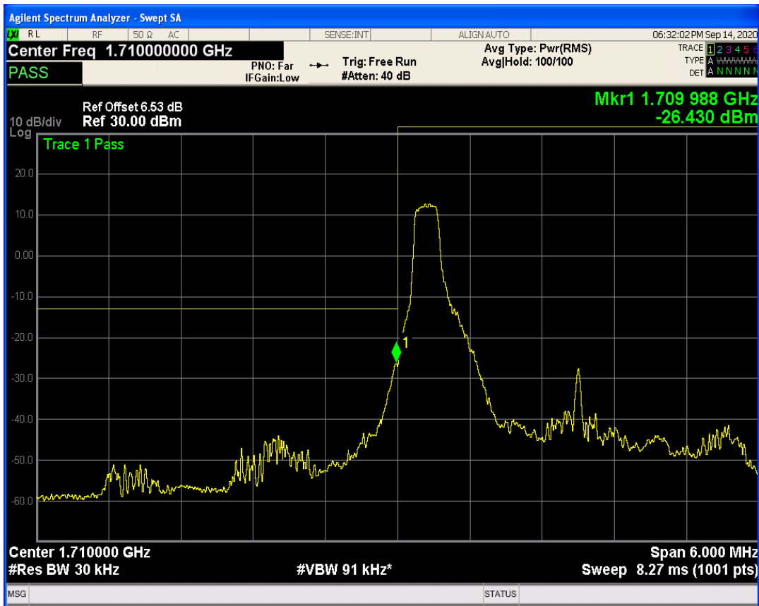
LTE Band66 QPSK BW=3MHz Channel=131987 RB Size=15 Position=#0
