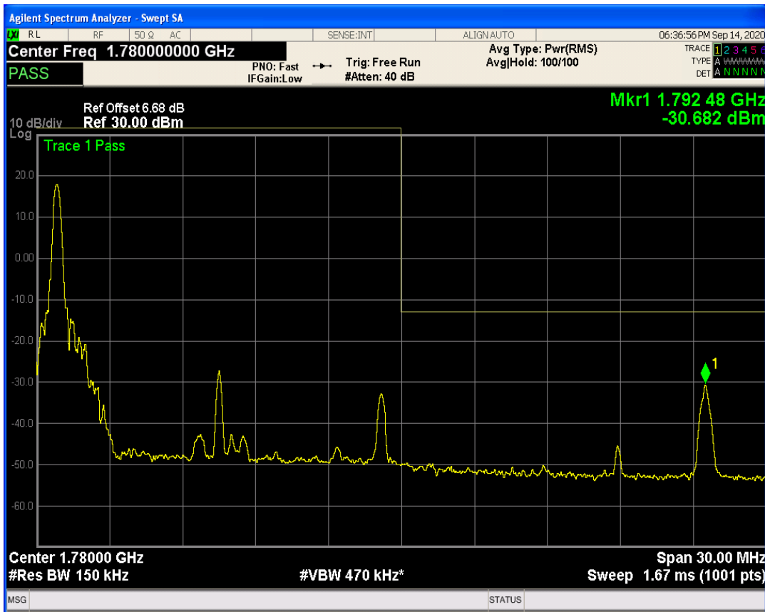
LTE Band66 QAM16 BW=15MHz Channel=132597 RB Size=75 Position=#0
