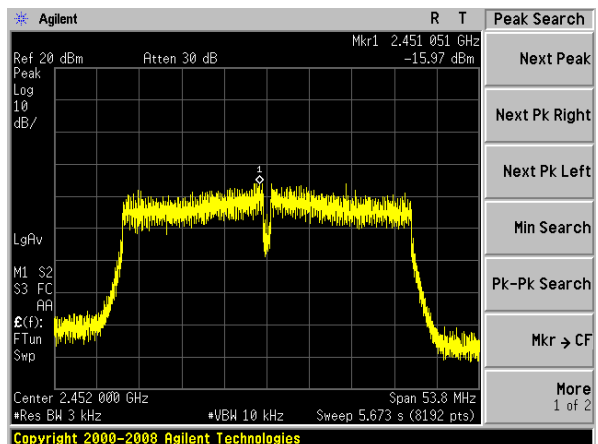
(802.11n40) PSD plot on channel 11
