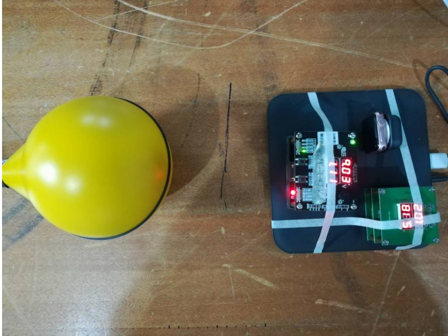
H-Filed Strength View Position A (Distance 15cm)
