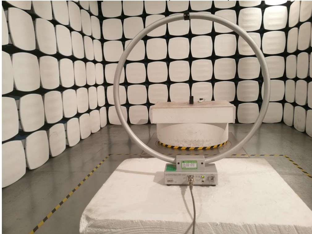
Radiated Emission(9kHz-30MHz)
