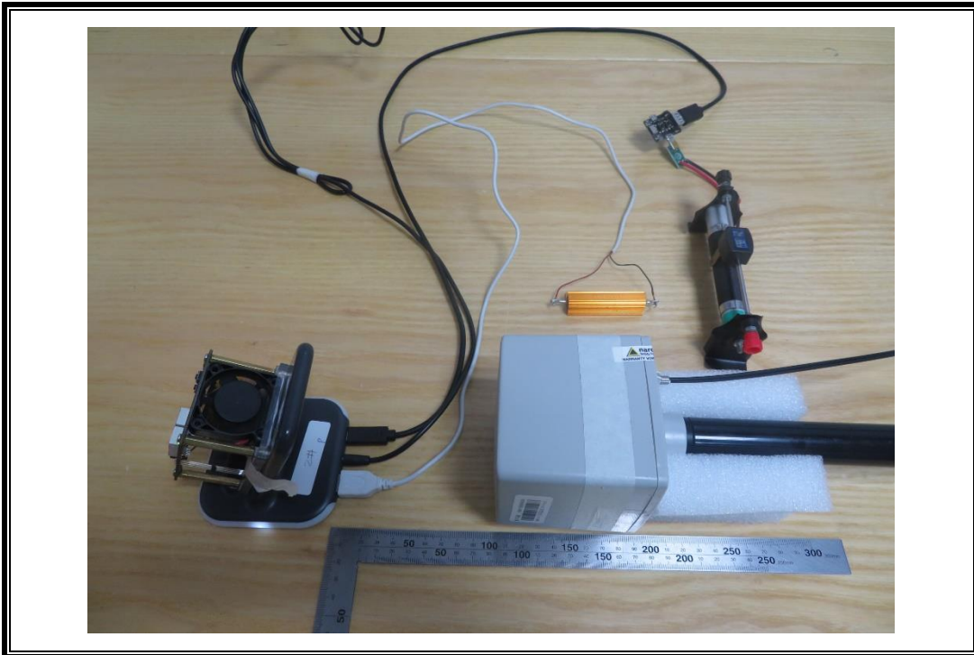
E-FILED AND H-FILED STRENGTH MEASUREMENT SETUP-3 (coil 1)
