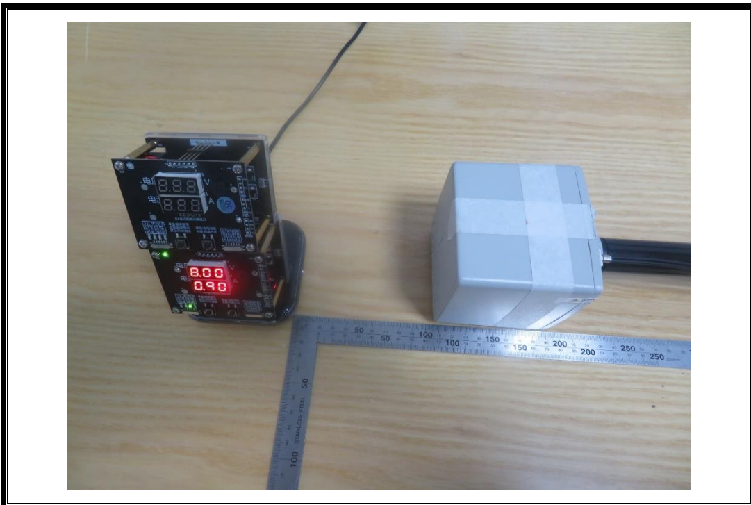
E-FILED AND H-FILED STRENGTH MEASUREMENT SETUP-6 (2 loads)
