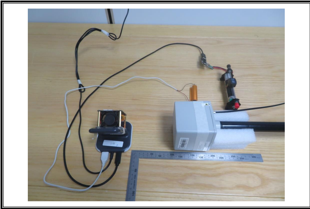
E-FILED AND H-FILED STRENGTH MEASUREMENT SETUP-5 (coil 1)
