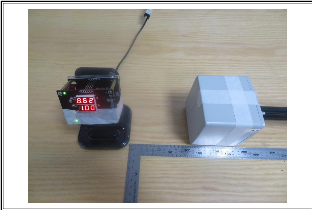
E-FILED AND H-FILED STRENGTH MEASUREMENT SETUP-6 (coil 2)
