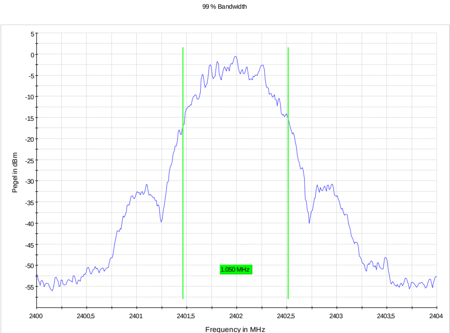
99 % Bandwidth,2402 MHz, -30 °C, 15 V
