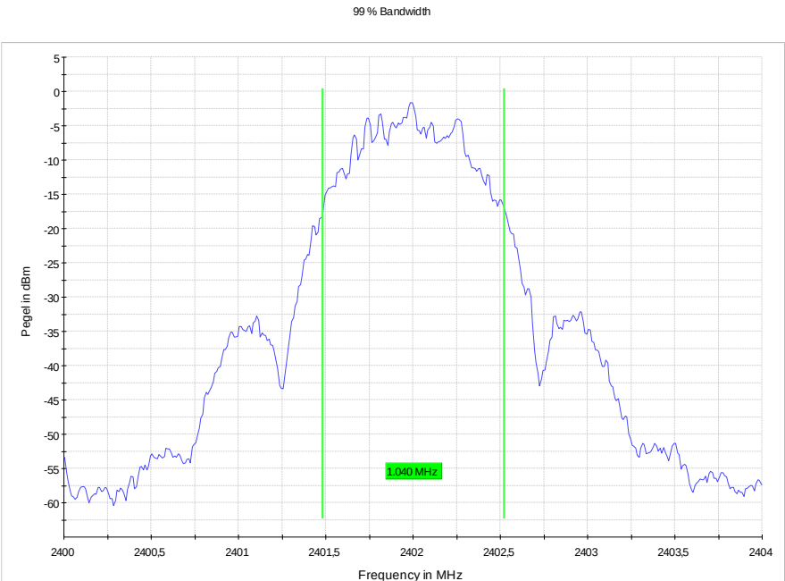
99 % Bandwidth,2402 MHz, 50 °C, 15 V
