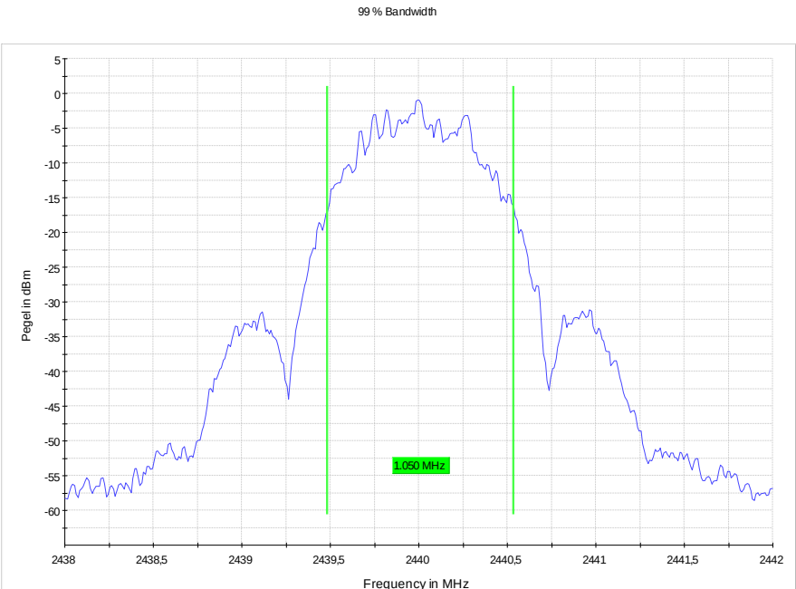
99 % Bandwidth, 2440 MHz, 20 °C, 17.25 V
