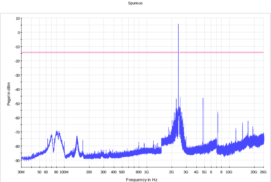
Spurious Conducted Emissions, 2402 MHz
