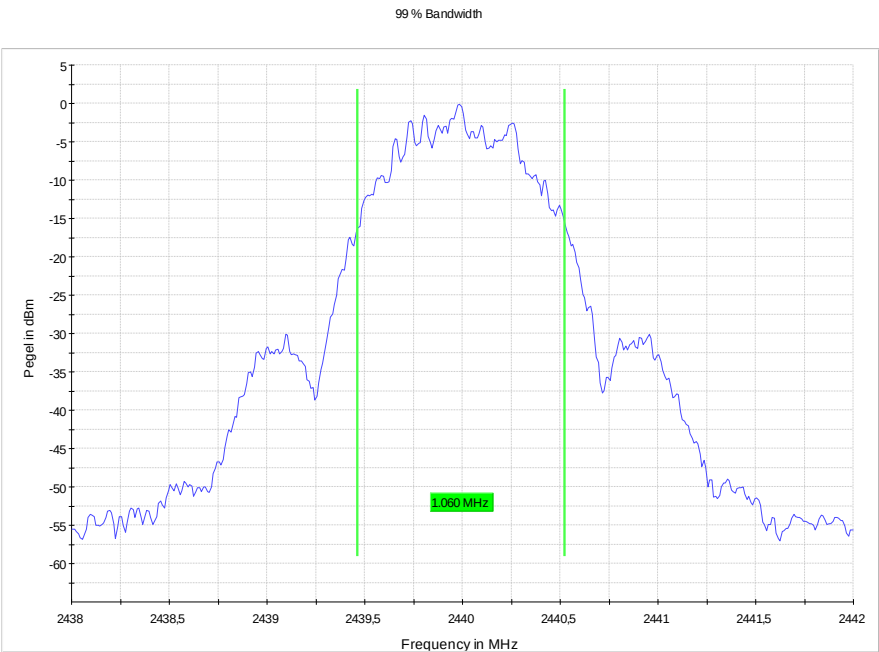
99 % Bandwidth, 2440 MHz, -30 °C, 15 V
