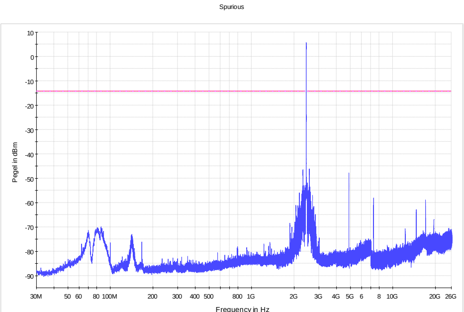
Spurious Conducted Emissions, 2440 MHz
