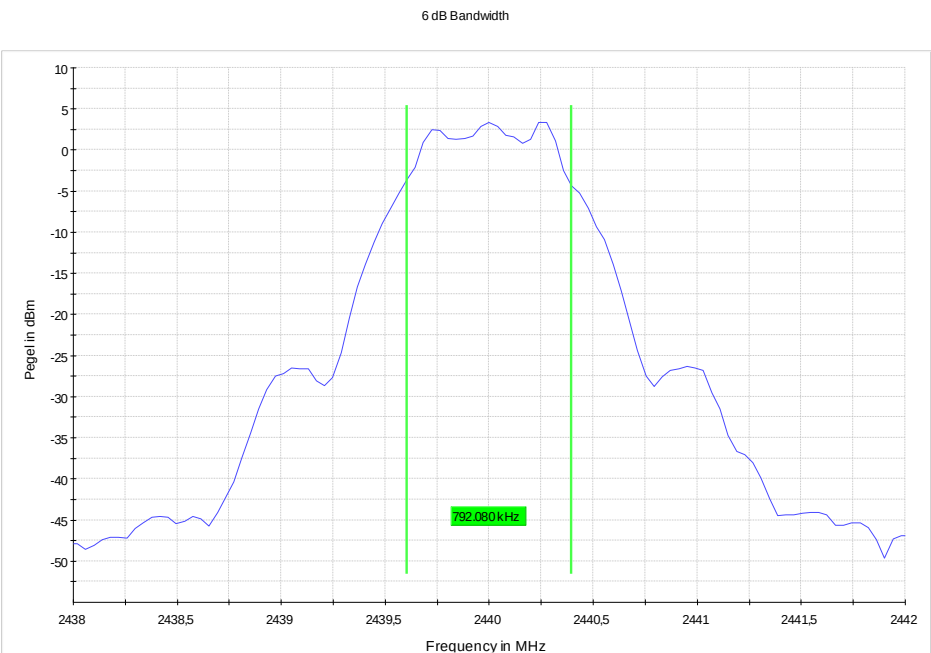
6 dB Bandwidth, 2440 MHz
