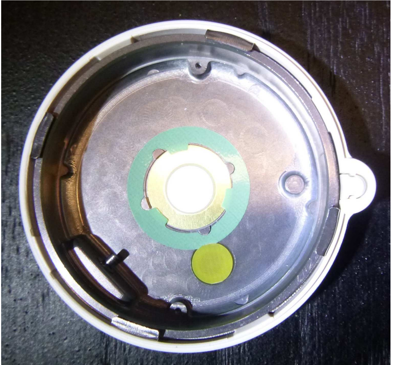
PCB Removed
