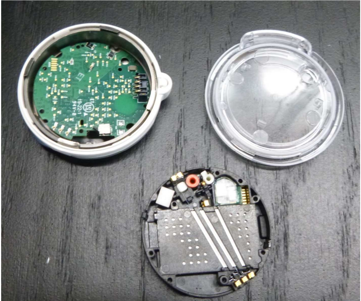
Covers Removed
