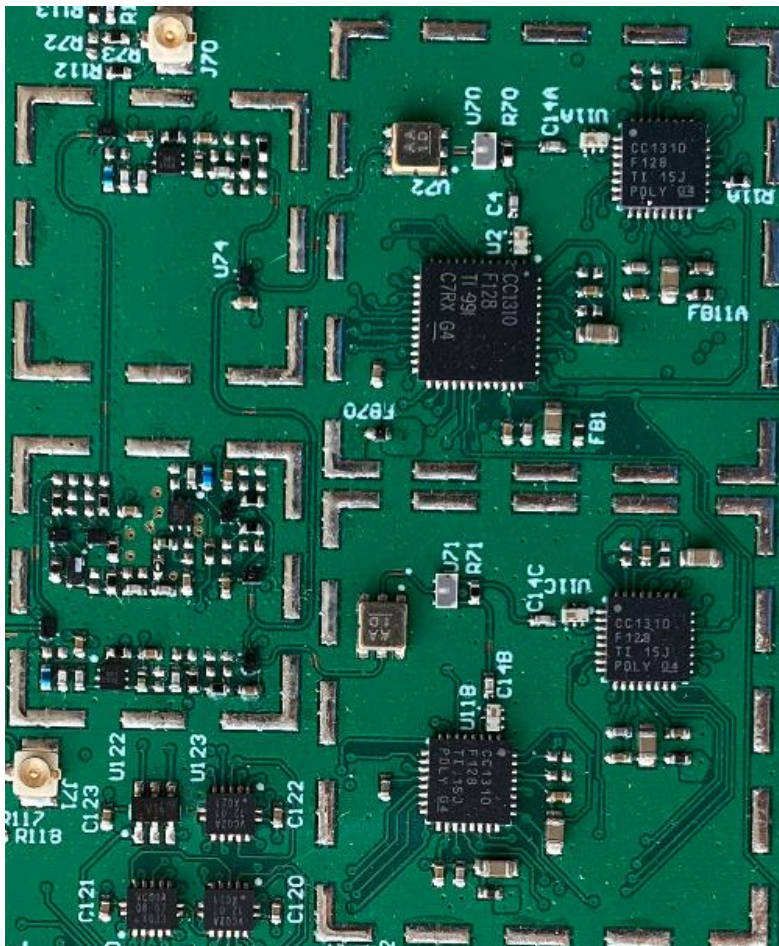
Figure 1: Closeup picture of components inside the shield boxes of part 102545 - SDS Module (US)
