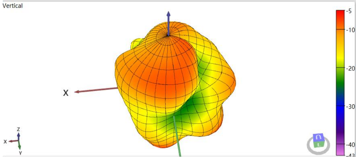
antenna 2440MHz 3D-Vertical Pattern
