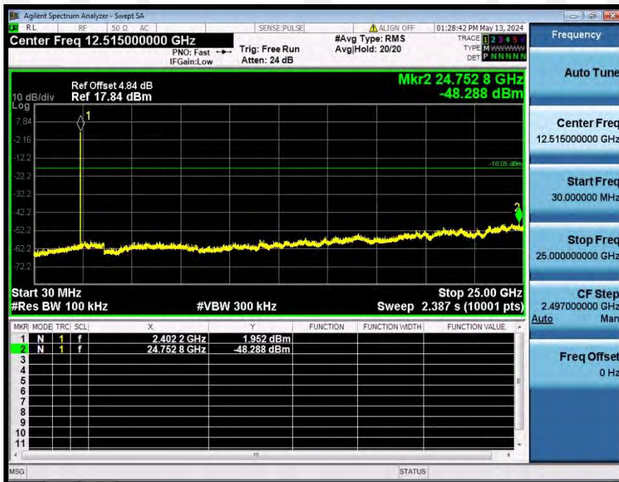
2_Spurious_Emissions_NVNT_ANT1_1-DH1_2402
