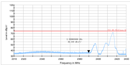
802.11b-Channel 1 Peak
