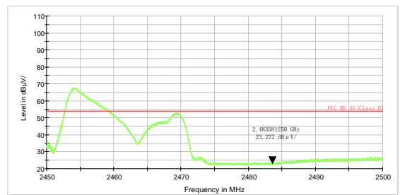
802.11g-Channel 11 Average
