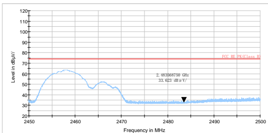
802.11b-Channel 11 Peak
