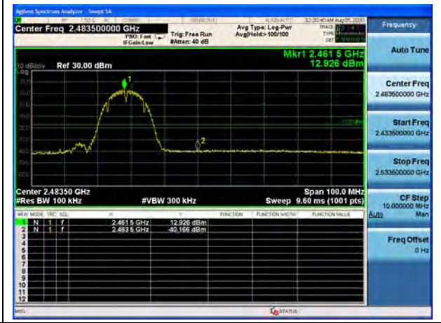
802.11b, Channel No.: 11
