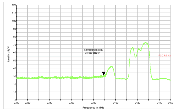
802.11g-Channel 3 Average
