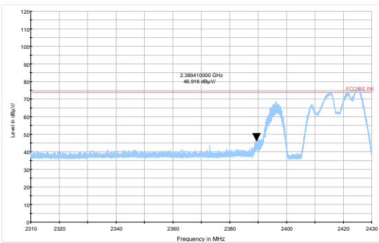
802.11n HT20 -Channel 2 Peak
