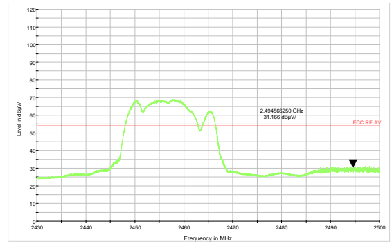
802.11n HT20 -Channel 10 Average
