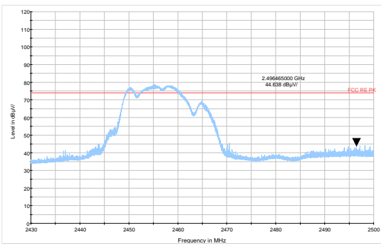
802.11g-Channel 10 Peak
