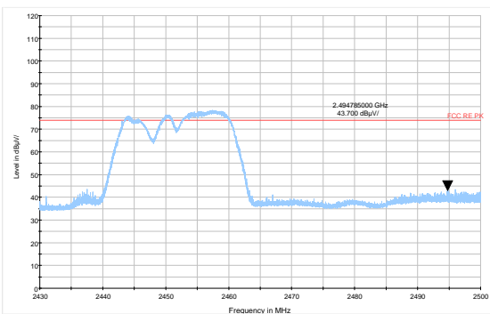
802.11n HT20 -Channel 9 Peak
