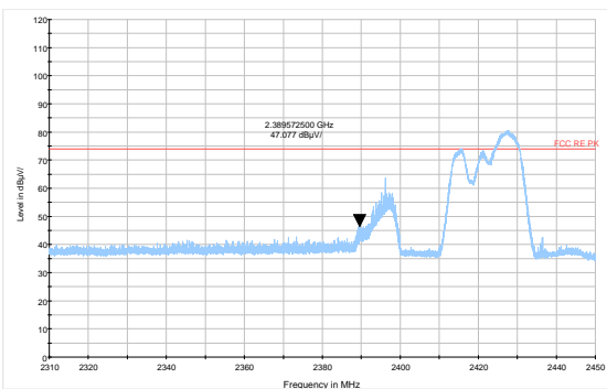
802.11n HT20 -Channel 3 Peak
