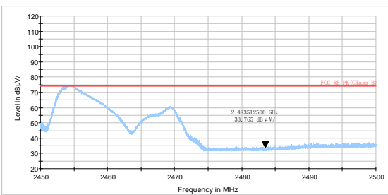
802.11g-Channel 11 Peak
