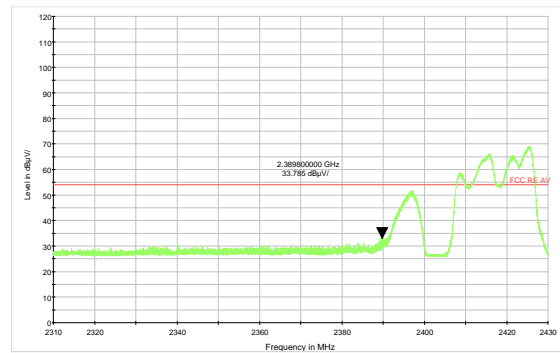
802.11n HT20 -Channel 2 Average
