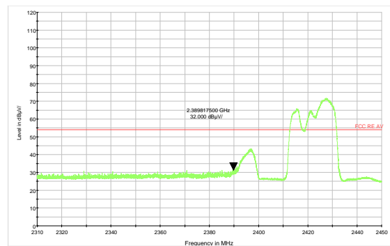
802.11n HT20 -Channel 3 Average
