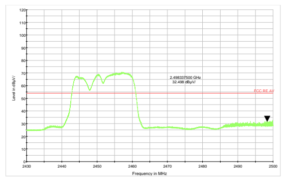
802.11g-Channel 9 Average
