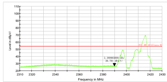
802.11b-Channel 1 Average
