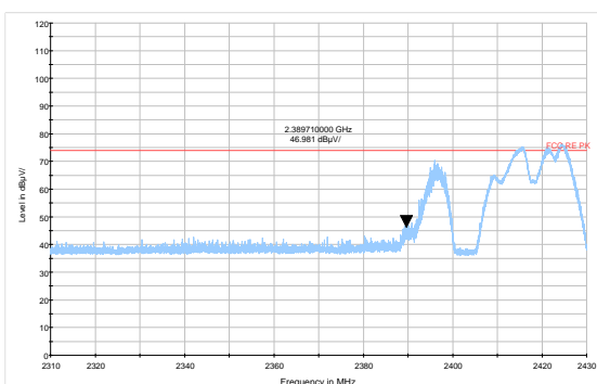
802.11g-Channel 2 Peak
