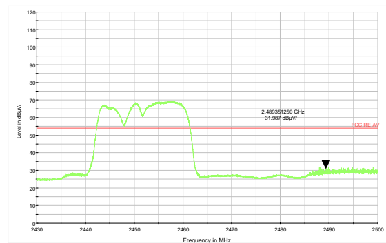
802.11n HT20 -Channel 9 Average
