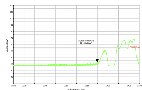
802.11g-Channel 2 Average
