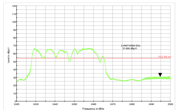
802.11n HT40 -Channel 8 Average
