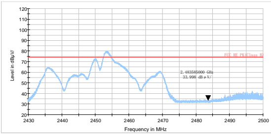
802.11n HT40 -Channel 9 Peak
