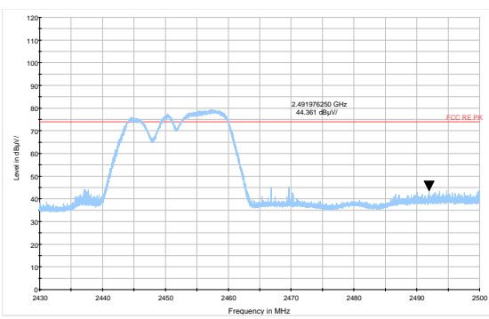
802.11g-Channel 9 Peak
