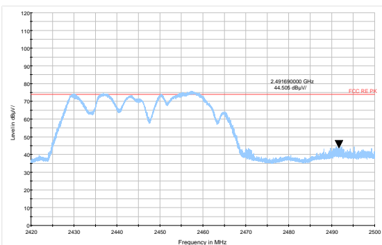
802.11n HT40 -Channel 8 Peak
