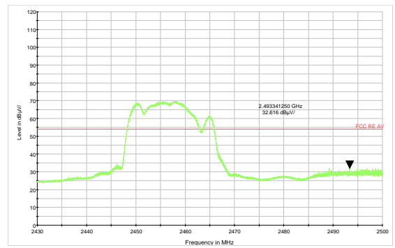
802.11g-Channel 10 Average
