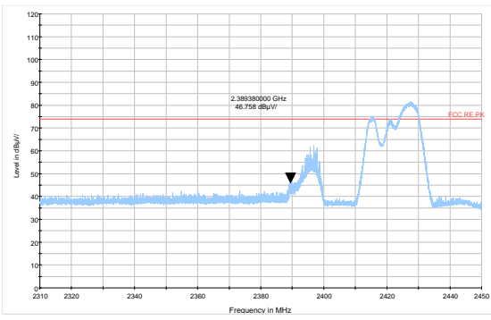
802.11g-Channel 3 Peak
