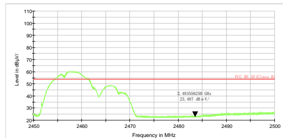
802.11b-Channel 11 Average
