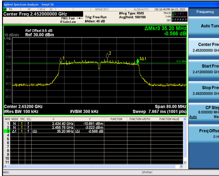
11N40SISO_Ant1_2452
